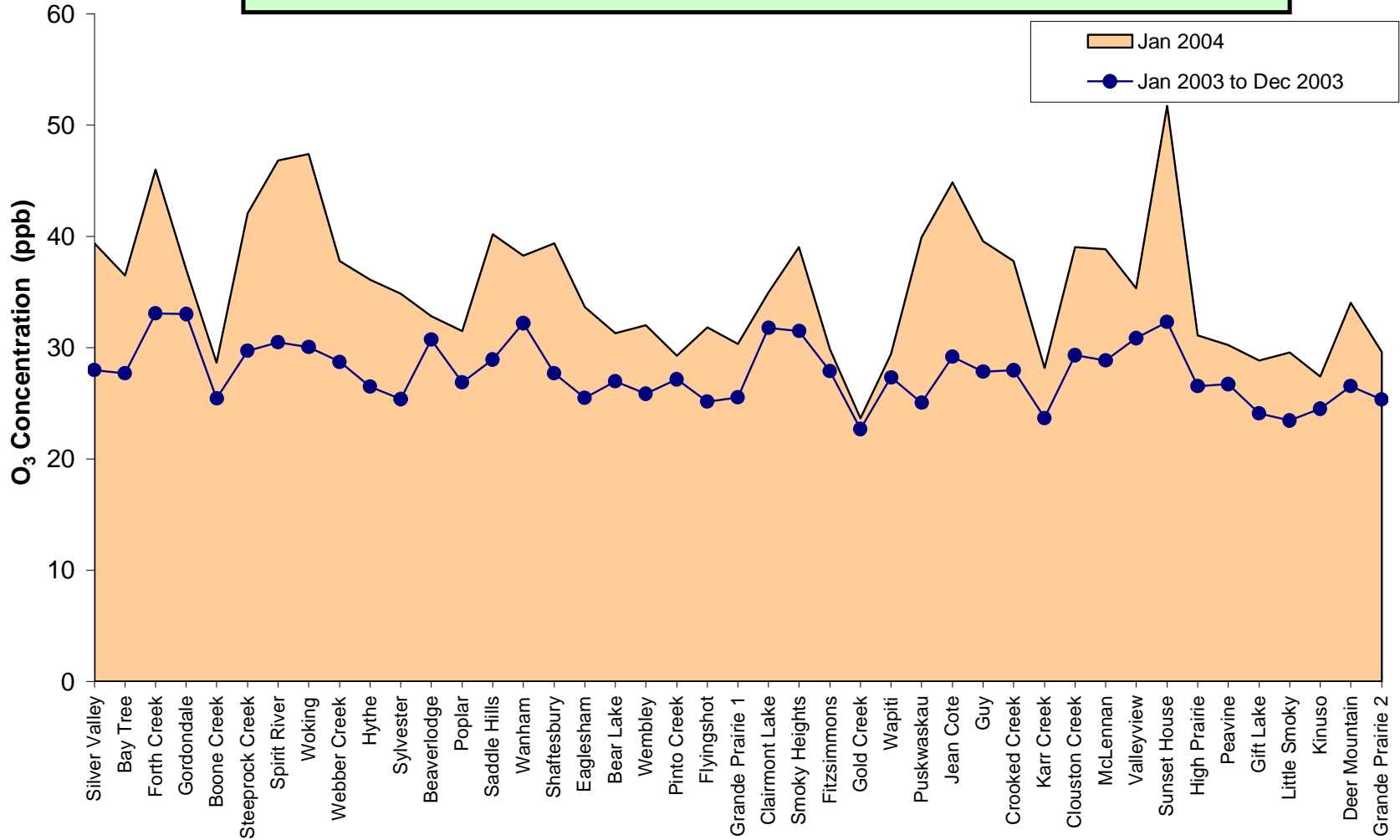
Figure 6. O 3 Summary Chart
