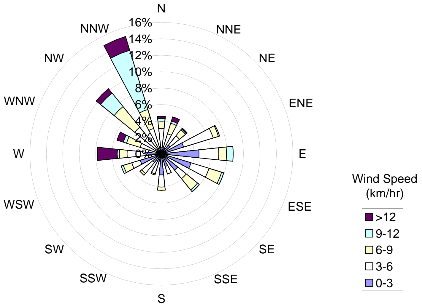
Figure 1. Wind Rose for the 1-hr Average Wind Speed Data Collected at the Beaverlodge Station during January 2004
