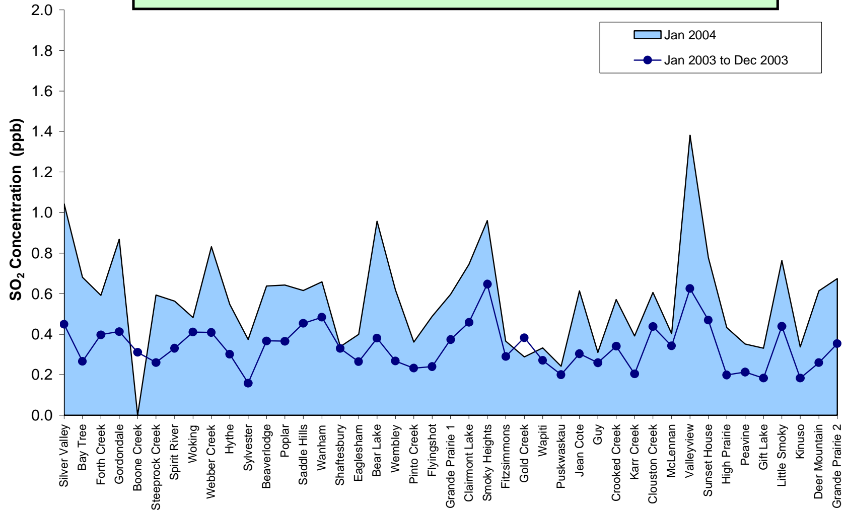
Figure 4. SO 2 Summary Chart
