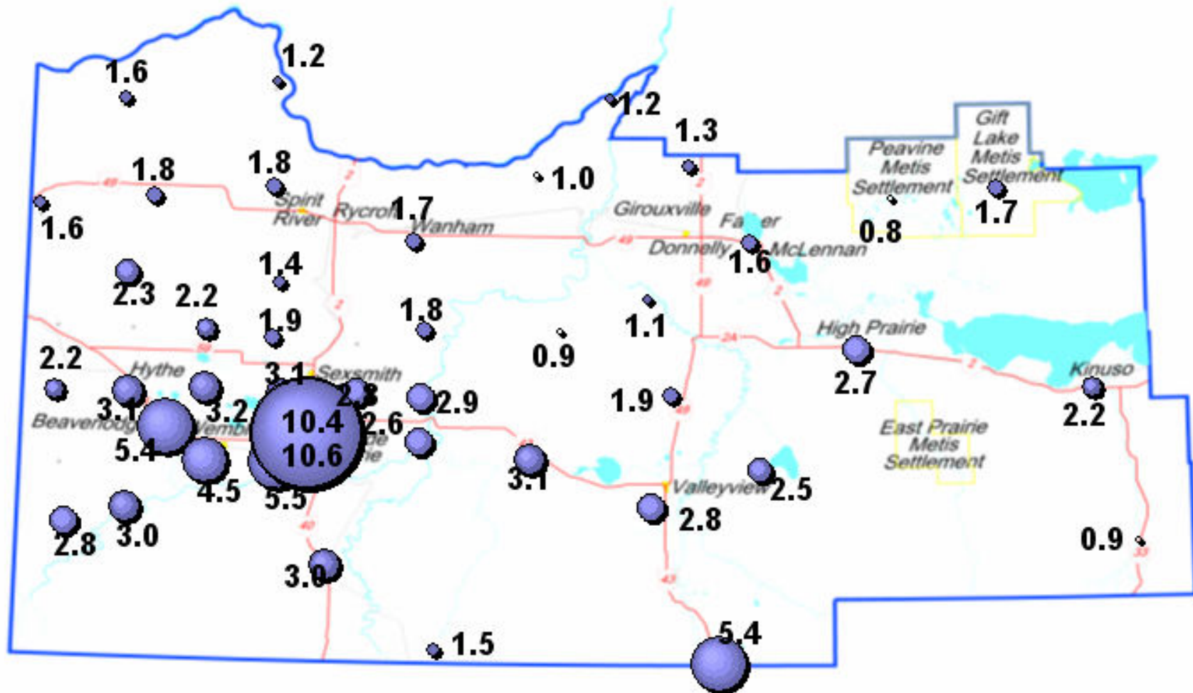
Figure 7. NO 2 Bubble Chart
