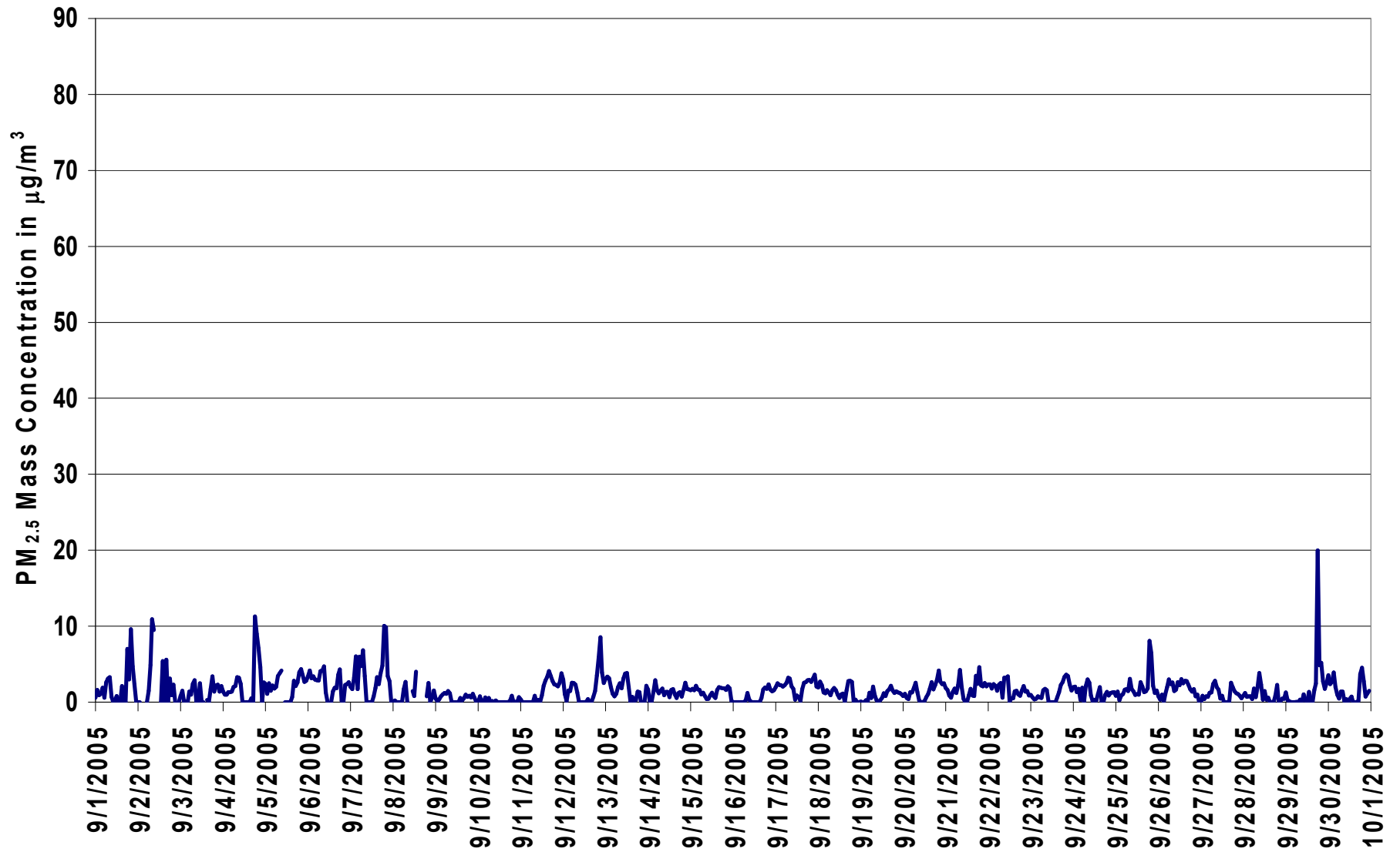
Figure 42. PASZA - Beaverlodge Particulate Matter (less than 2.5 microns) 1-hr Average Monthly Trend
