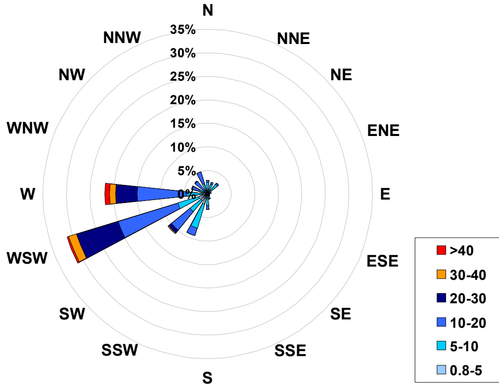
1-hr Average Wind Rose (in km/hr) Located at the Smoky Heights Site for September 2005
