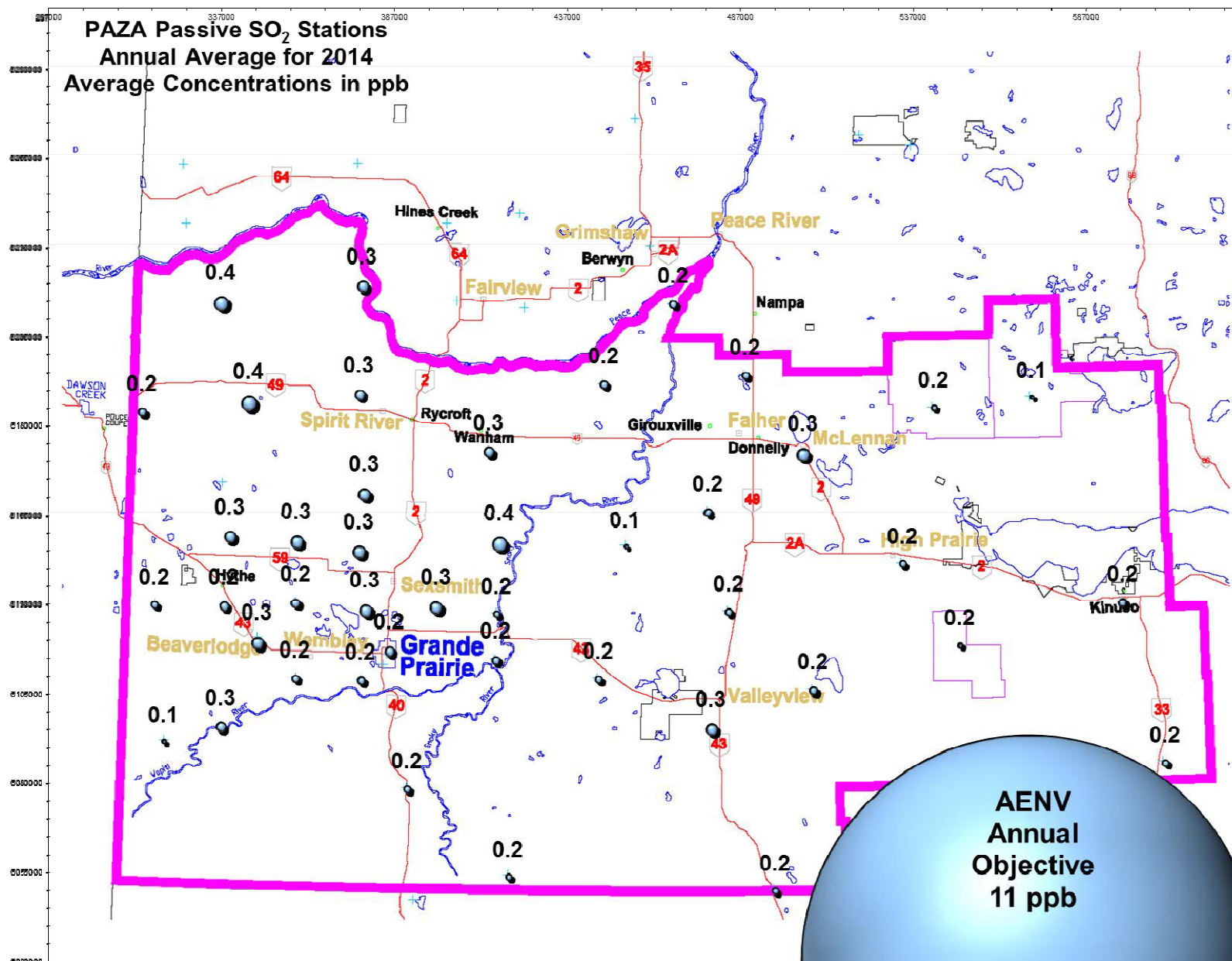
Figure 11. PAZA SO 2 Bubble Chart – 2014 Annual Average
