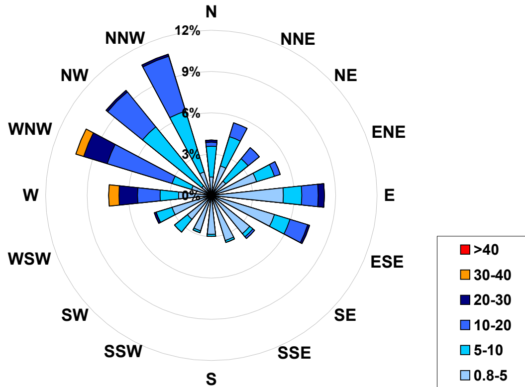
1-hr Average Wind Rose (in km/hr) Located at the Beaverlodge Site for February 2006
