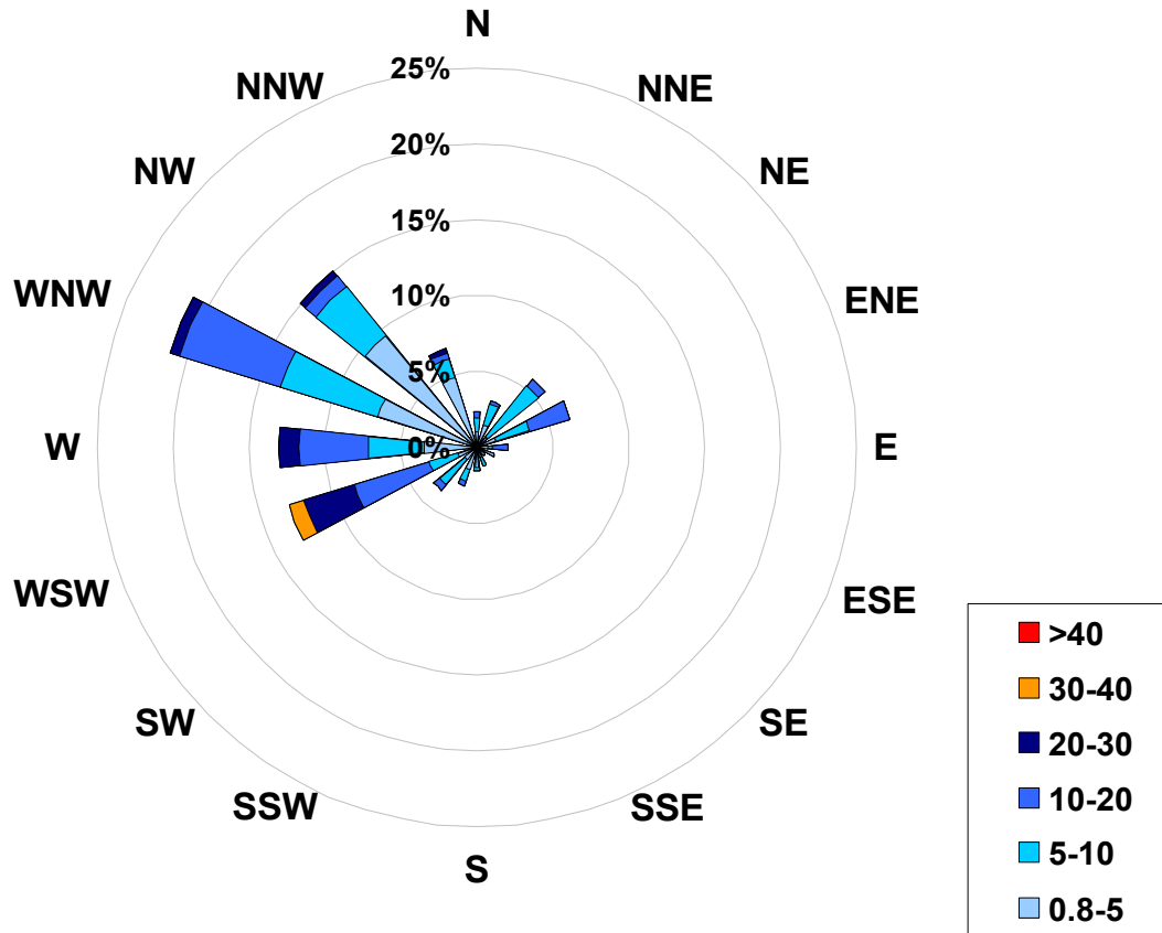
1-hr Average Wind Rose (in km/hr) Located at the Henry Pirker Site for February 2006
