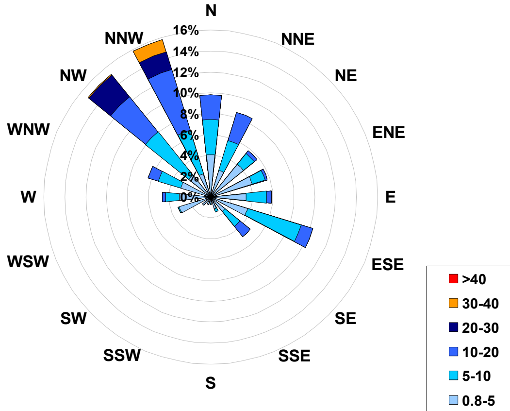
1-hr Average Wind Rose (in km/hr) Located at the Evergreen Park Site for February 2006
