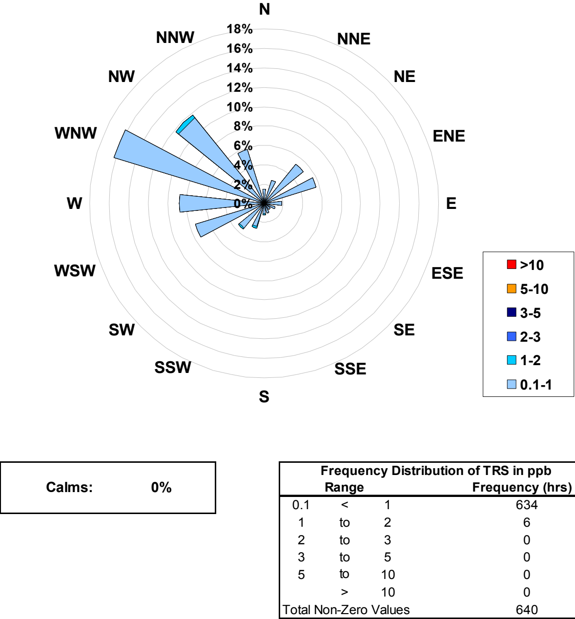
1-hr Average Concentration Rose for Total Reduced Sulphur (in ppb) Located at the Henry Pirker Site for February 2006
