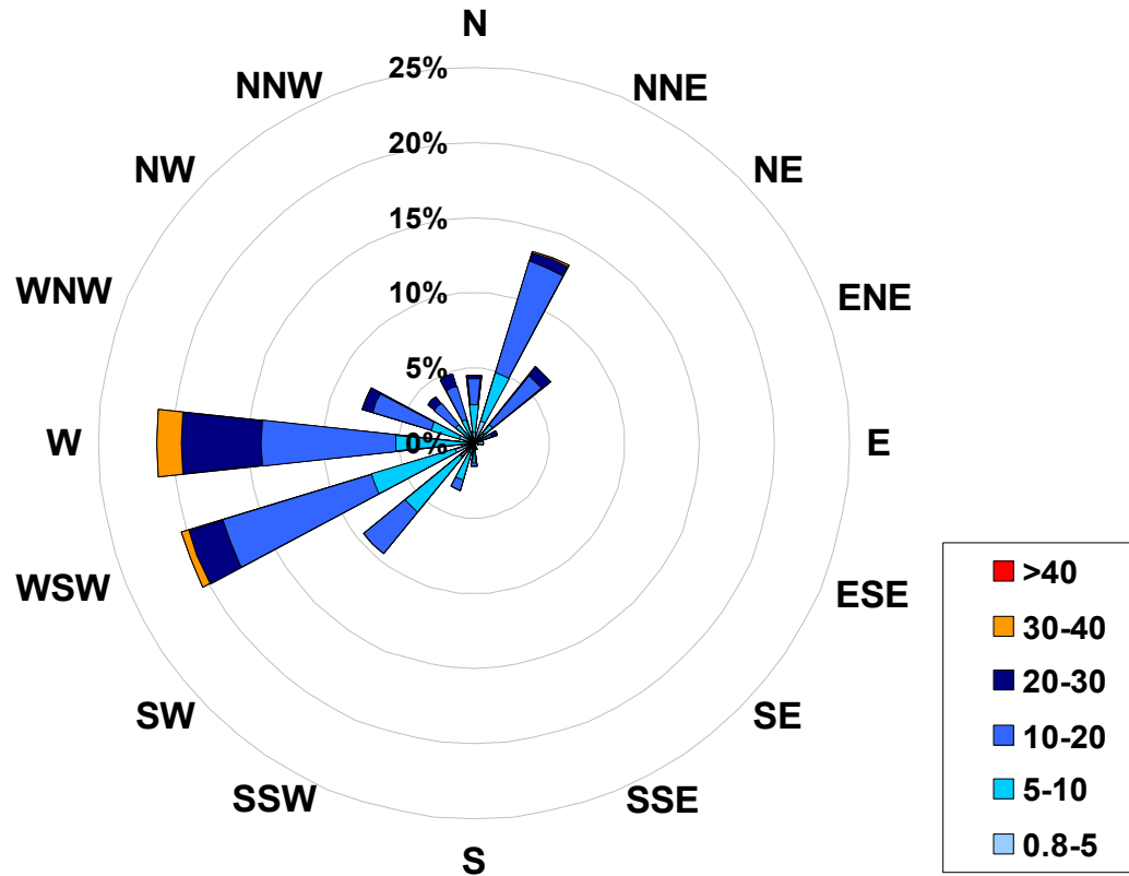
1-hr Average Wind Rose (in km/hr) Located at the Smoky Heights Site for February 2006
