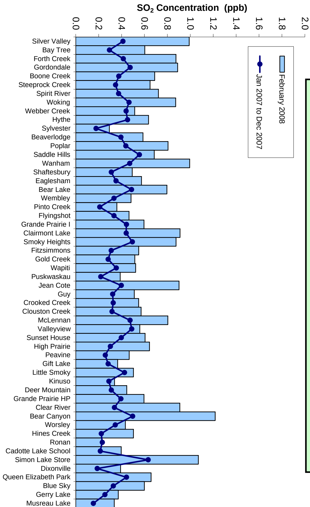
Figure 63. SO 2 Summary Chart
