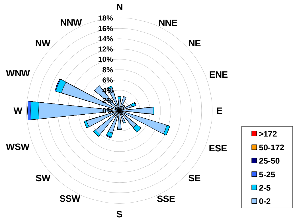
1-hr Average Concentration Rose for Sulphur Dioxide (in ppb) Located at the Portable-Spirit River Site for February 2008
