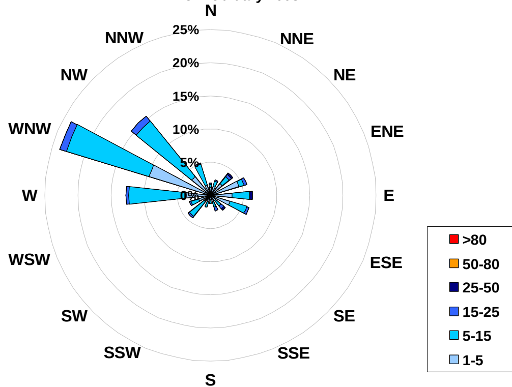
1-hr Average Concentration Rose for Particulate Matter (less than 2.5 microns) (in micrograms per cubic meter) Located at the Henry Pirker Site for February 2008
