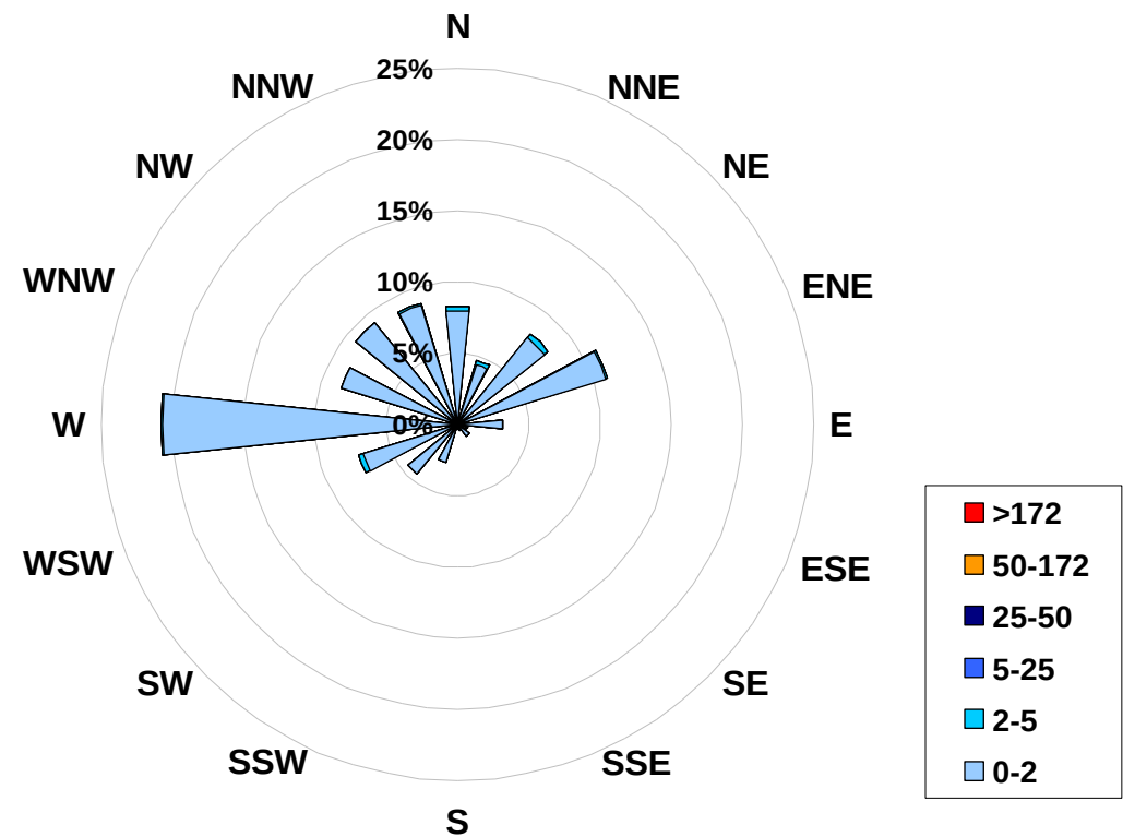
1-hr Average Concentration Rose for Sulphur Dioxide (in ppb) Located at the Evergreen Park Site for February 2008
