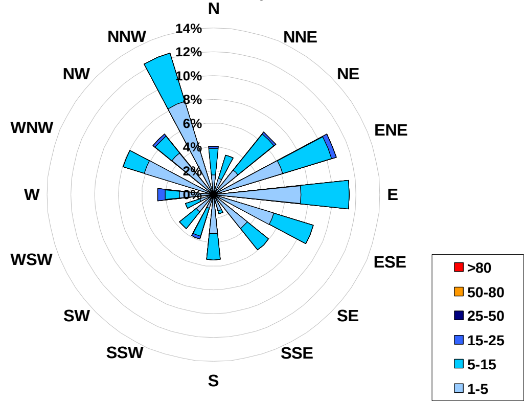
1-hr Average Concentration Rose for Particulate Matter (less than 2.5 microns) (in micrograms per cubic meter) Located at the Beaverlodge Site for February 2008
