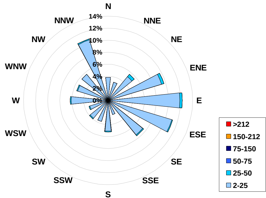
1-hr Average Concentration Rose for Nitrogen Dioxide (in ppb) Located at the Beaverlodge Site for February 2008
