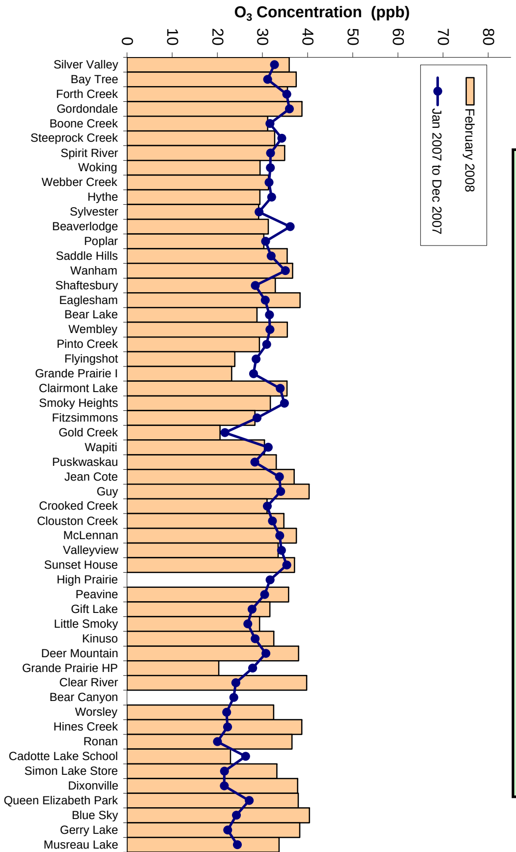
Figure 65. O 3 Summary Chart
