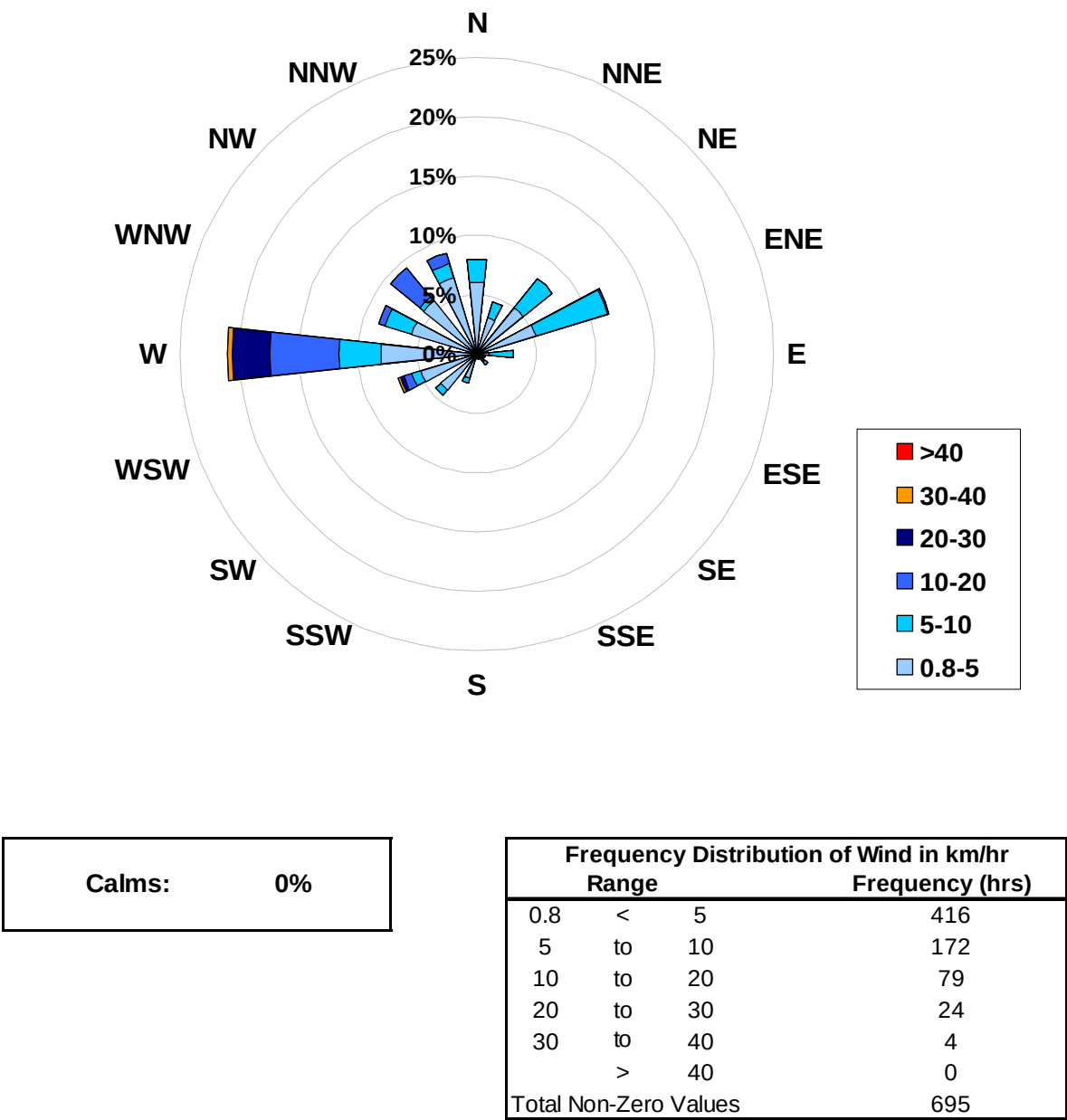
1-hr Average Wind Rose (in km/hr) Located at the Evergreen Park Site for February 2008
