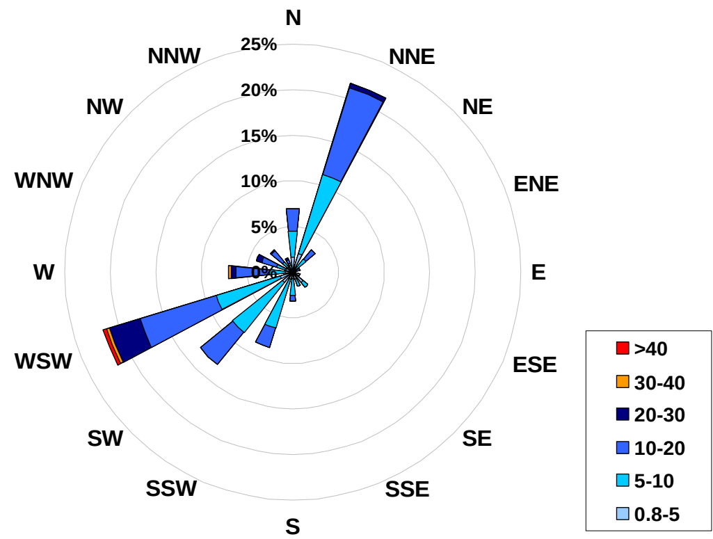
1-hr Average Wind Rose (in km/hr) Located at the Smoky Heights Site for February 2008
