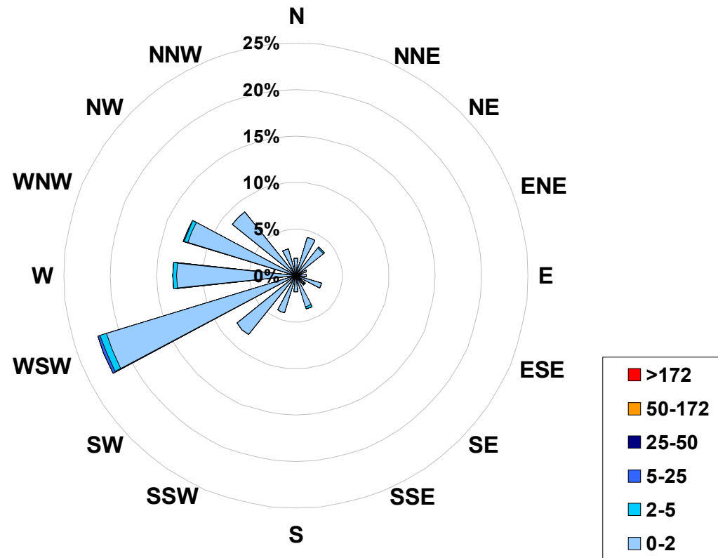
1-hr Average Concentration Rose for Sulphur Dioxide (in ppb) Located at the Henry Pirker Site for July 2006
