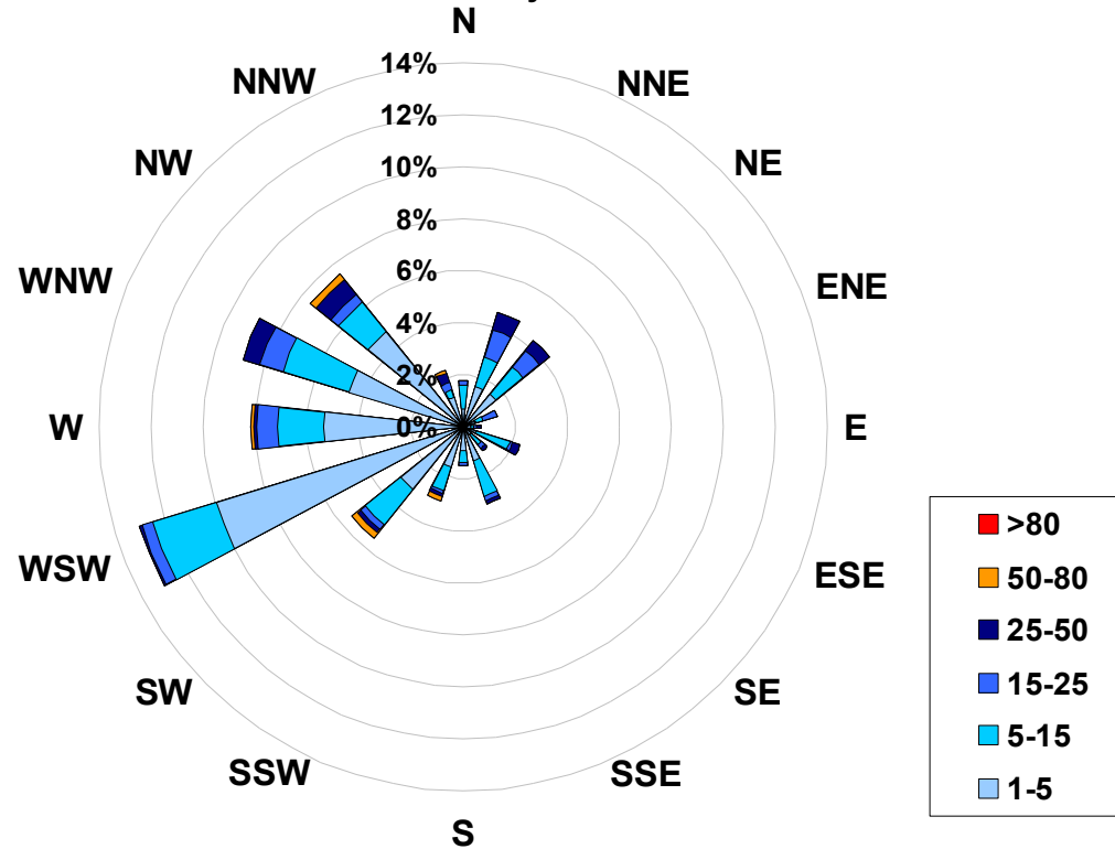
1-hr Average Concentration Rose for Particulate Matter (less than 2.5 microns) (in micrograms per cubic meter) Located at the Henry Pirker Site for July 2006
