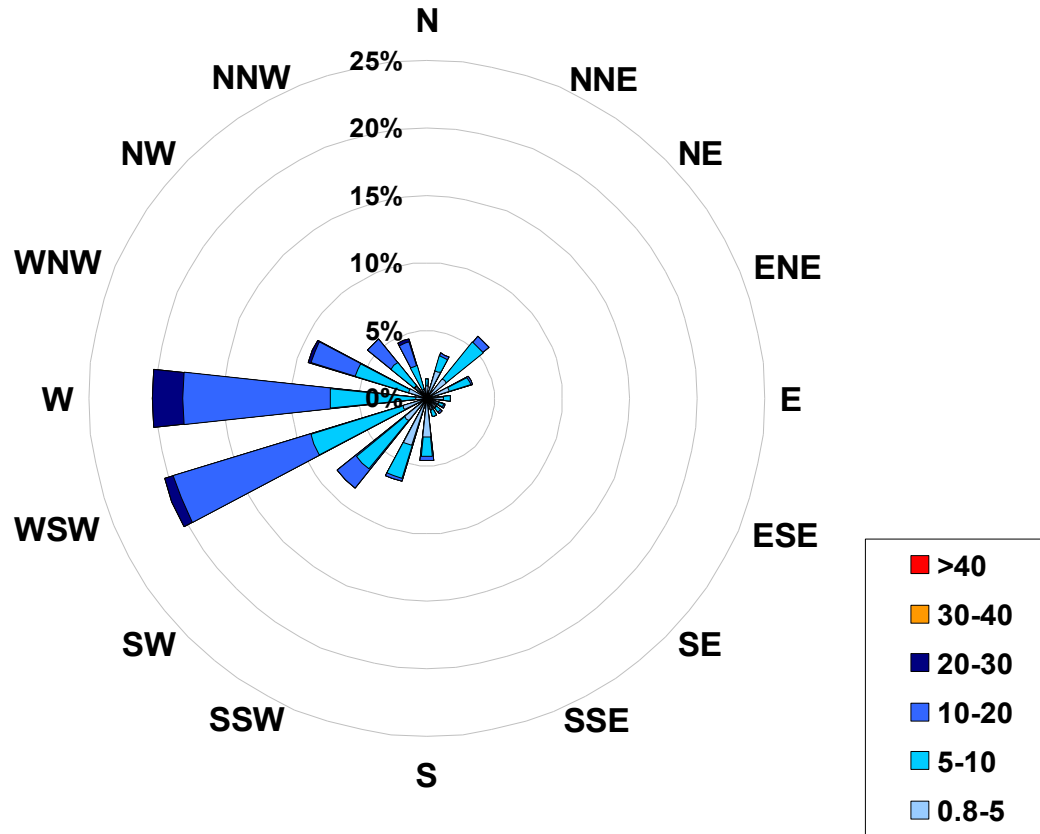
1-hr Average Wind Rose (in km/hr) Located at the Evergreen Park Site for July 2006
