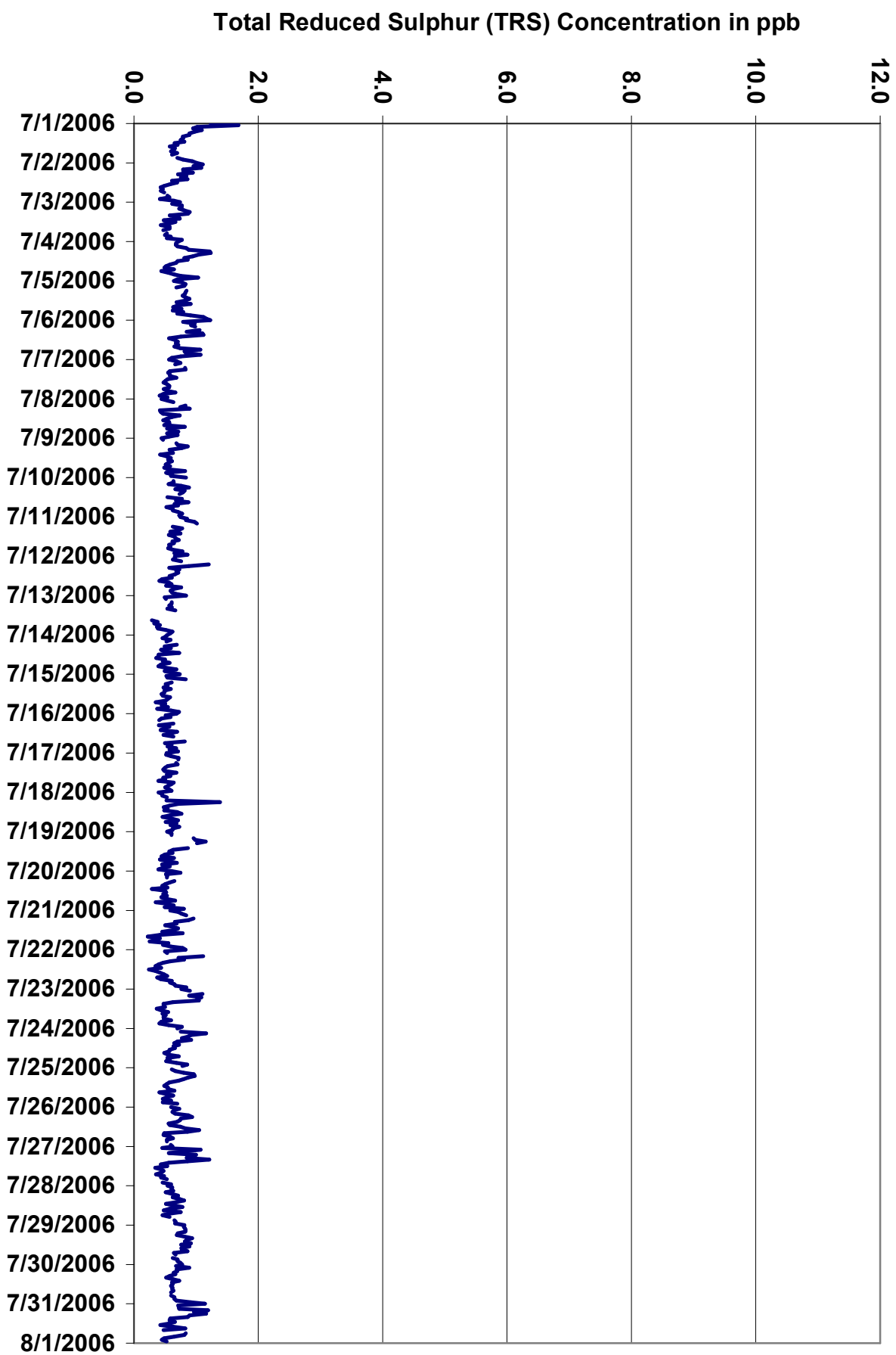
Figure 14. PASZA - Henry Pirkner Total Reduced Sulphur Instantaneous (30 Second) Maximum Value Monthly Trend
