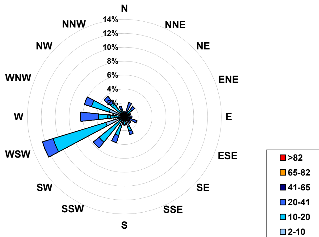
1-hr Average Concentration Rose for Ozone (in ppb) Located at the Henry Pirker Site for July 2006
