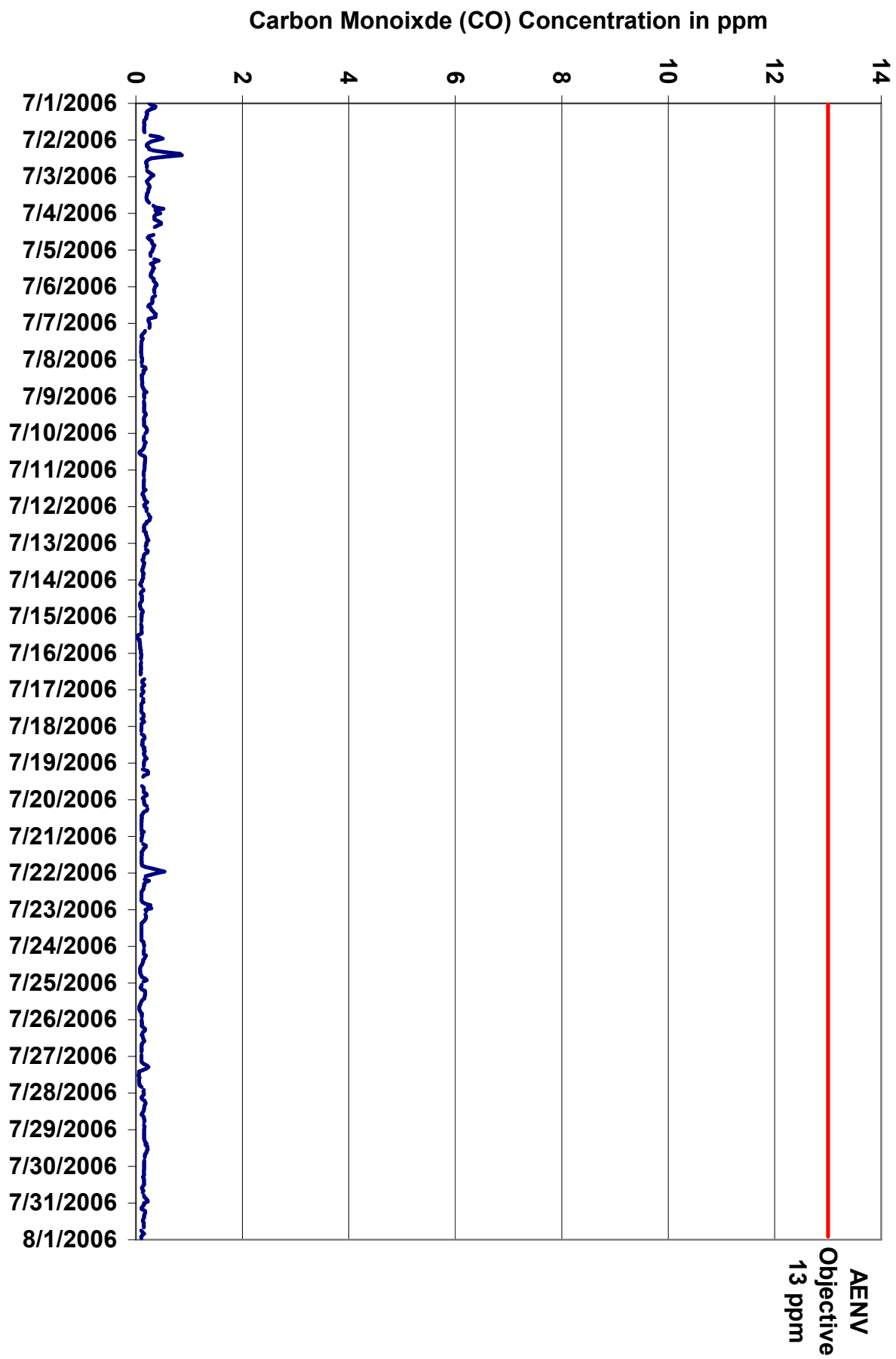
Figure 9. PASZA - Henry Parker Carbon Monoxide 1-hr Average Monthly Trend
