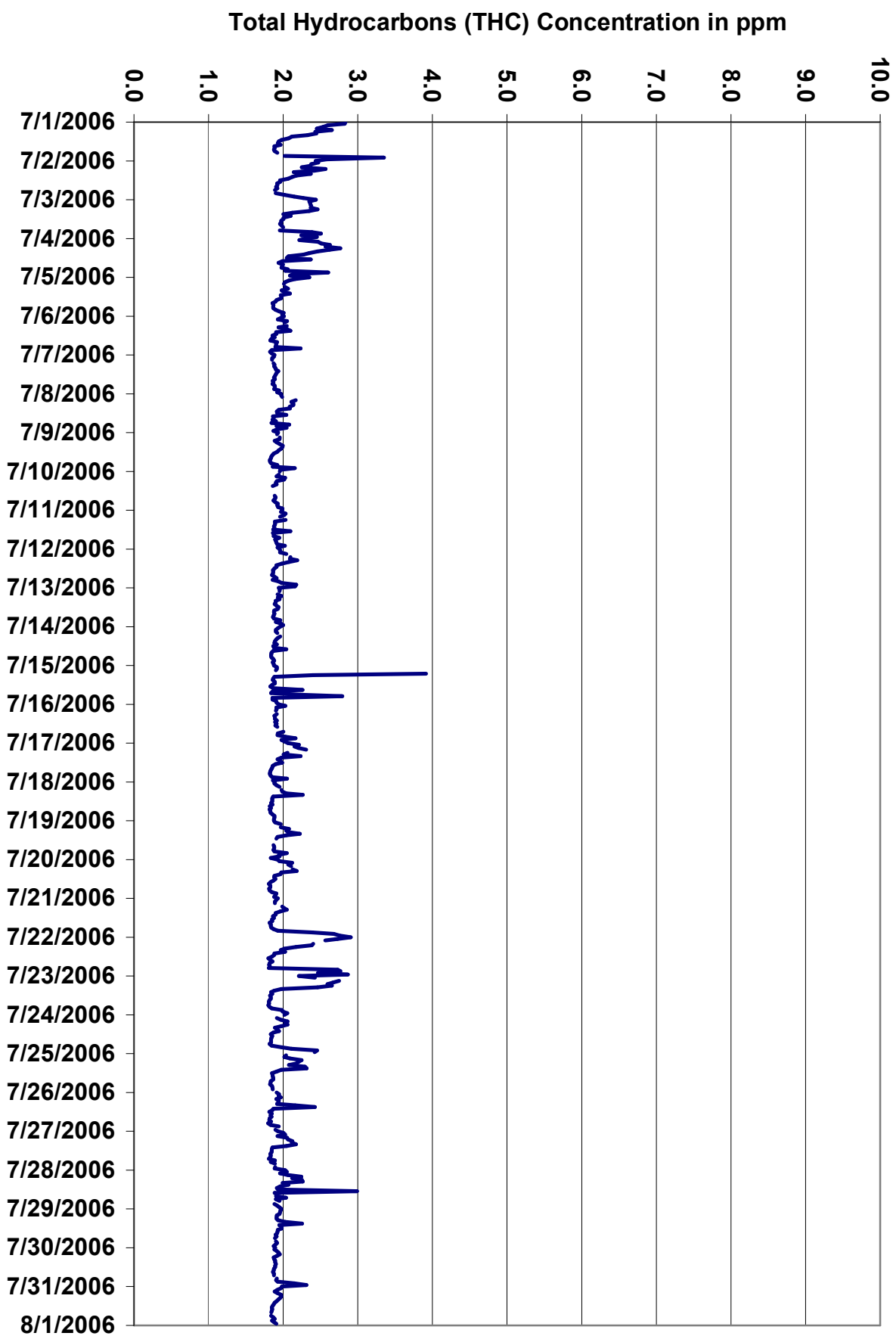
Figure 12. PASZA - Henry Pitker Total Hydrocarbons Instantaneous (30 Second) Maximum Value Monthly Trend
