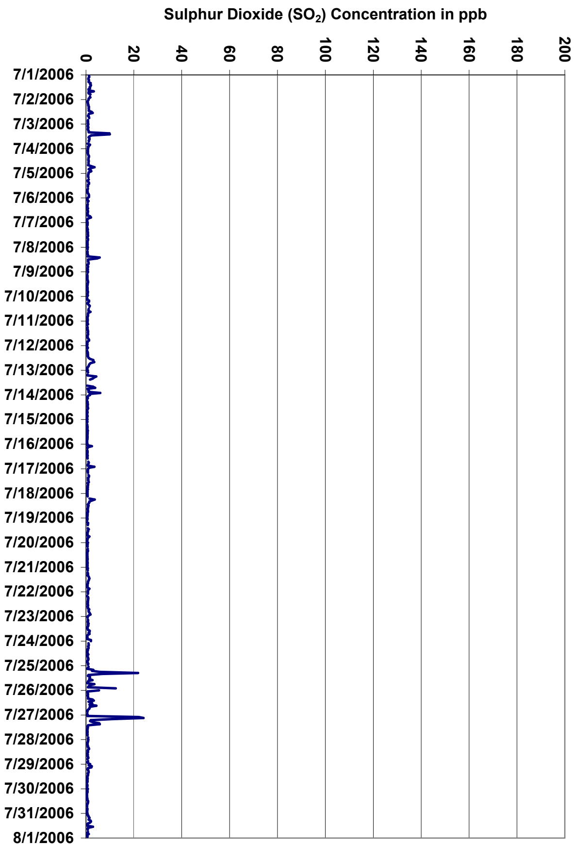
Figure 2. PASZA - Henry Pitker Sulphur Dioxide Instantaneous (30 Second) Maximum Value Monthly Trend
