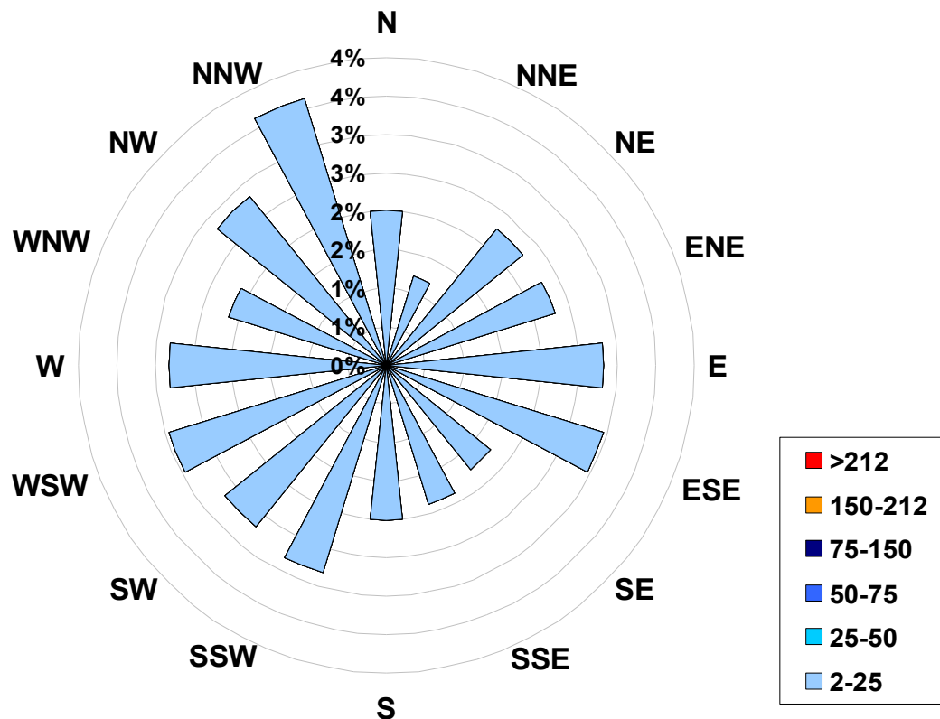
1-hr Average Concentration Rose for Nitrogen Dioxide (in ppb) Located at the Beaverlodge Site for July 2006
