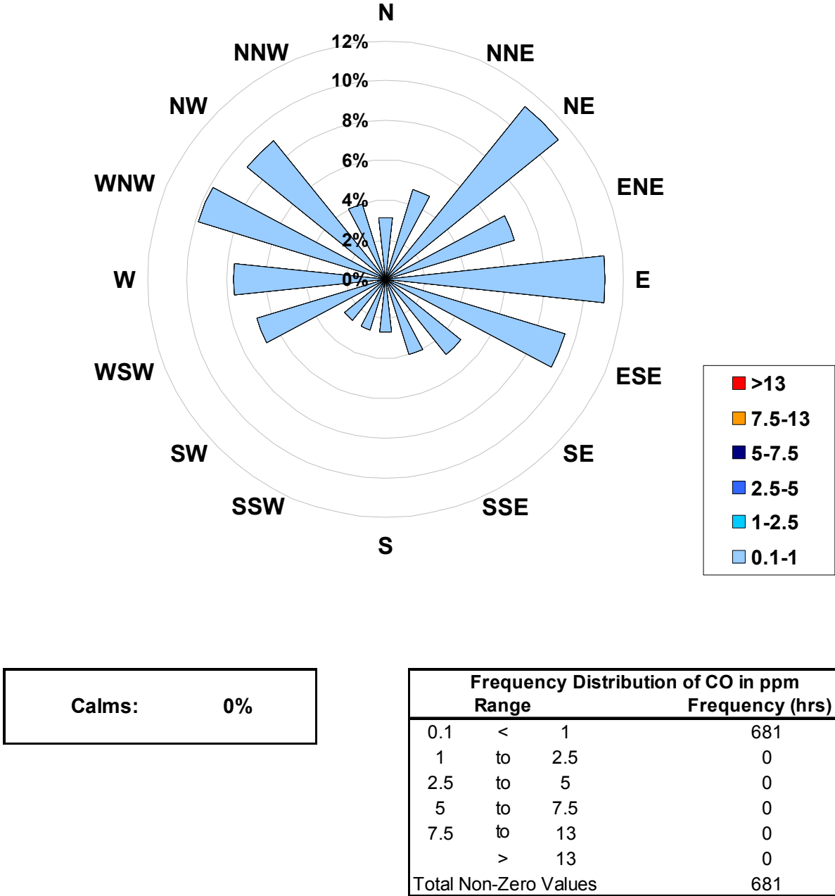
1-hr Average Concentration Rose for Carbon Monoxide (in ppm) Located at the Henry Pirker Site for June 2005
