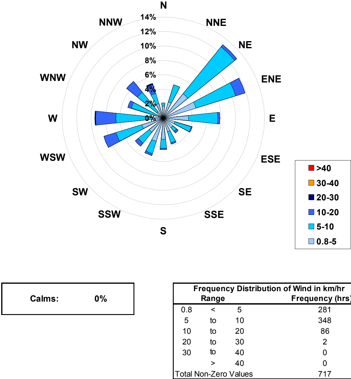
1-hr Average Wind Rose (in km/hr) Located at the Evergreen Park Site for June 2005
