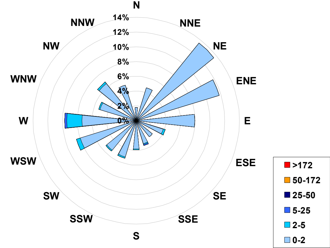
1-hr Average Concentration Rose for Sulphur Dioxide (in ppb) Located at the Evergreen Park Site for June 2005
