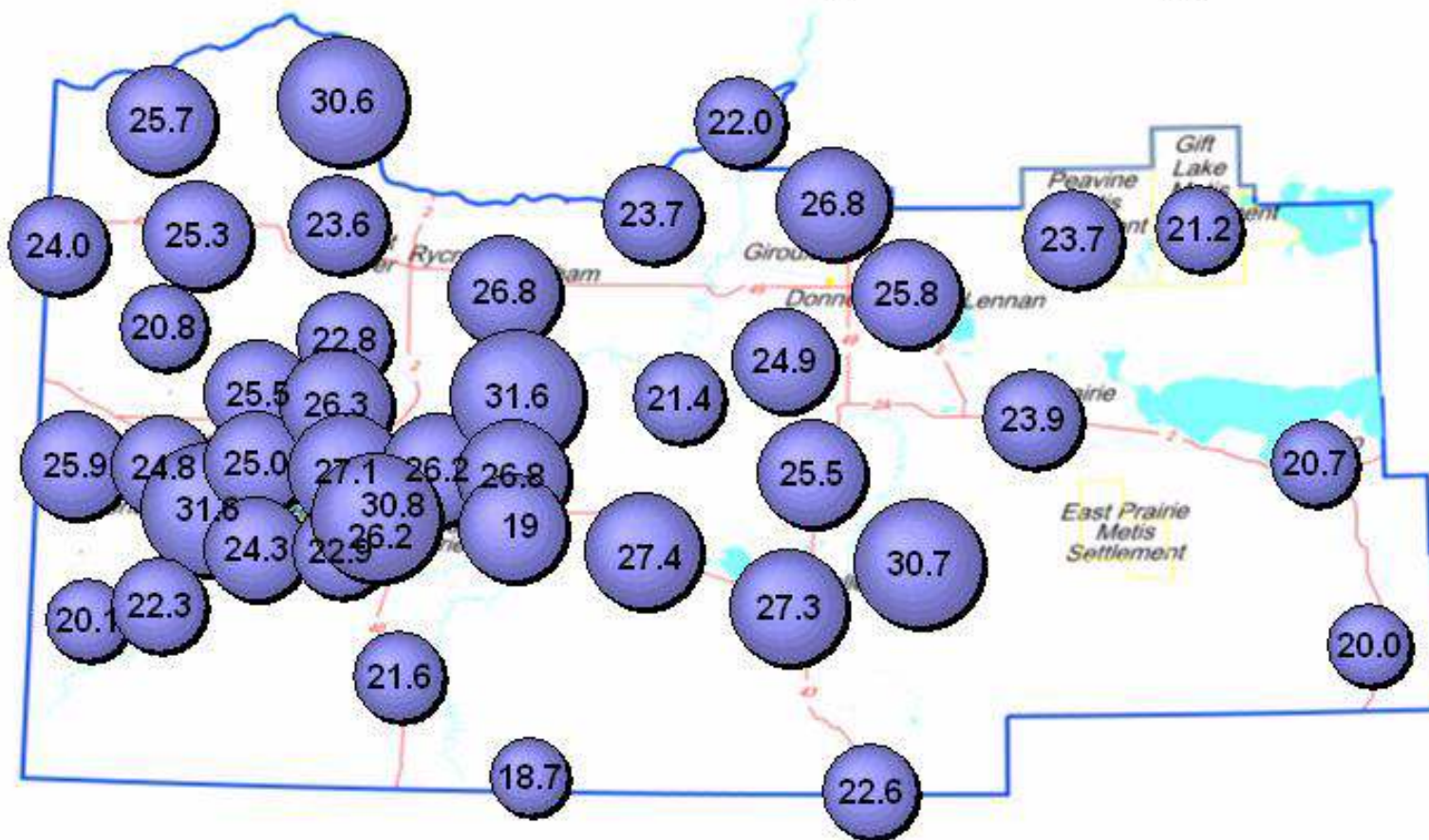
PASZA Passive O 3 Stations - June 2005 Average Concentrations in ppb
