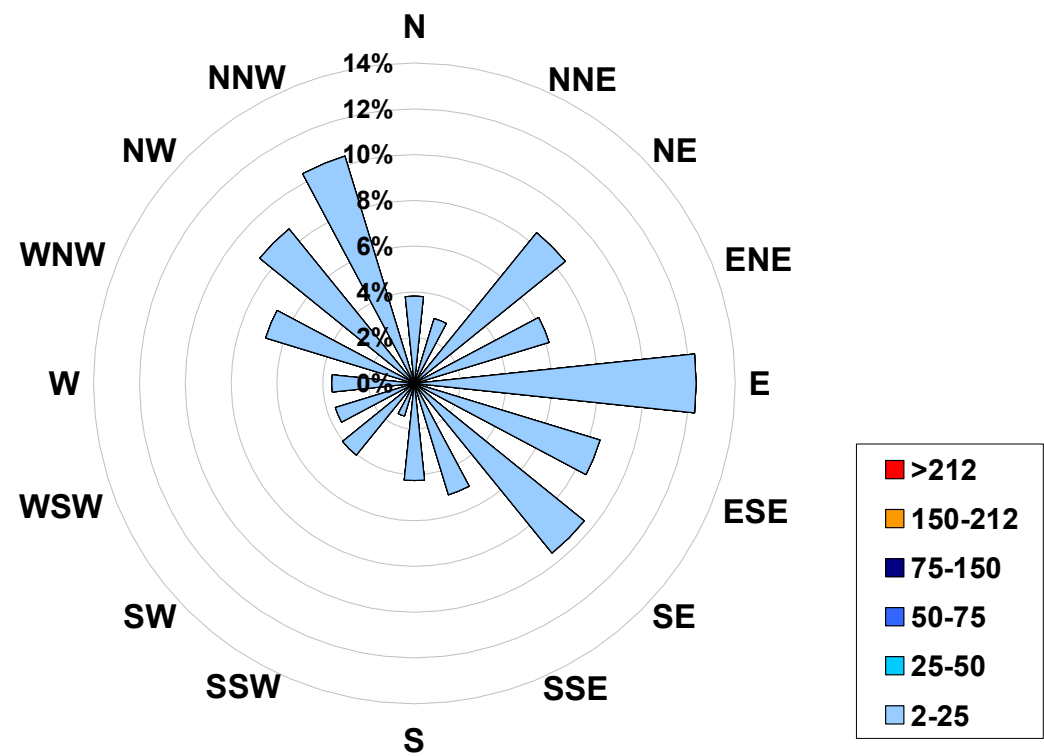
1-hr Average Concentration Rose for Nitrogen Dioxide (in ppb) Located at the Beaverlodge Site for June 2005
