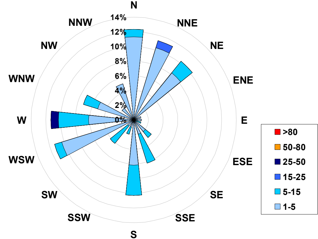
1-hr Average Concentration Rose for Particulate Matter (less than 2.5 microns) (in micrograms per cubic meter) Located at the Smoky Heights Site for June 2005
