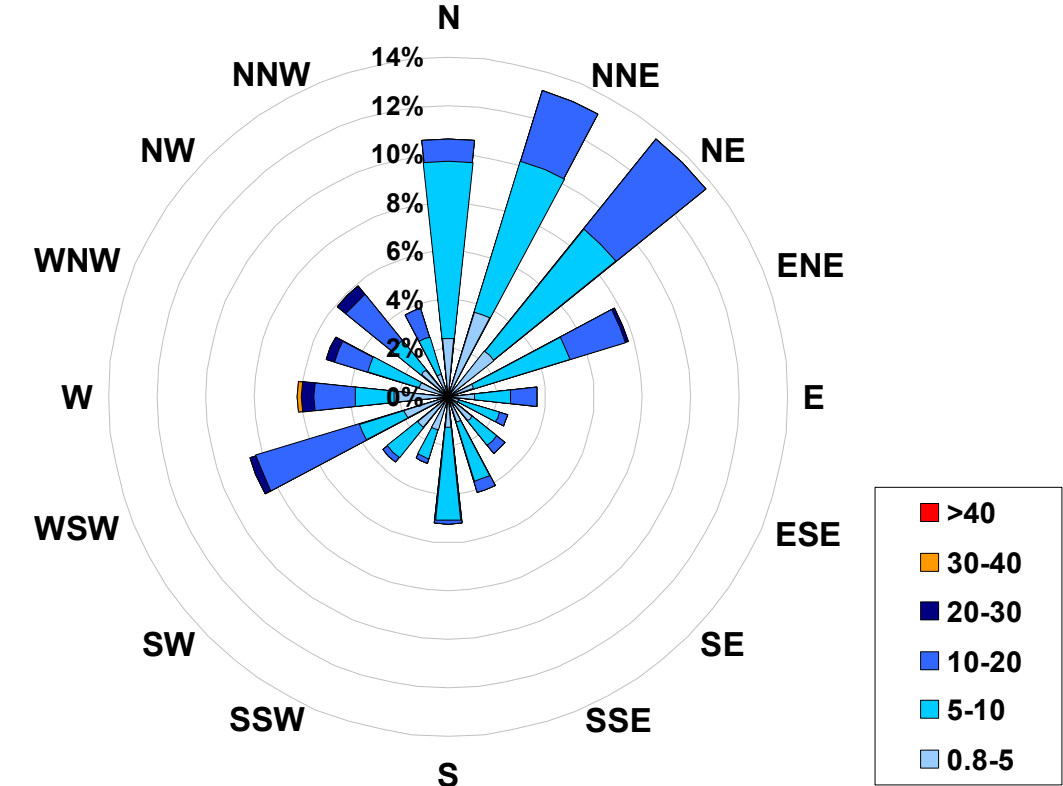
1-hr Average Wind Rose (in km/hr) Located at the Smoky Heights Site for June 2005
