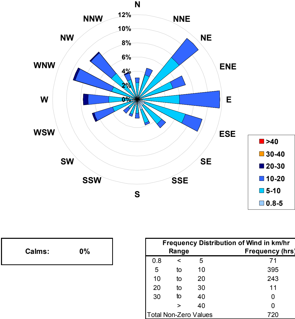
1-hr Average Wind Rose (in km/hr) Located at the Henry Pirker Site for June 2005
