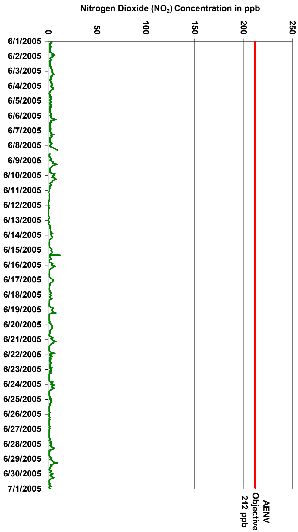
Figure 35. PASZA - Beaverlodge Nitrogen Dioxide 1-hr Average Monthly Trend
