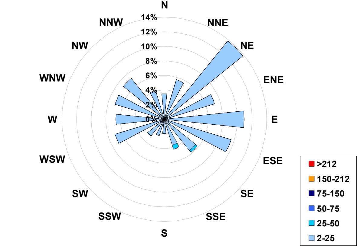
1-hr Average Concentration Rose for Nitrogen Dioxide (in ppb) Located at the Henry Pirker Site for June 2005
