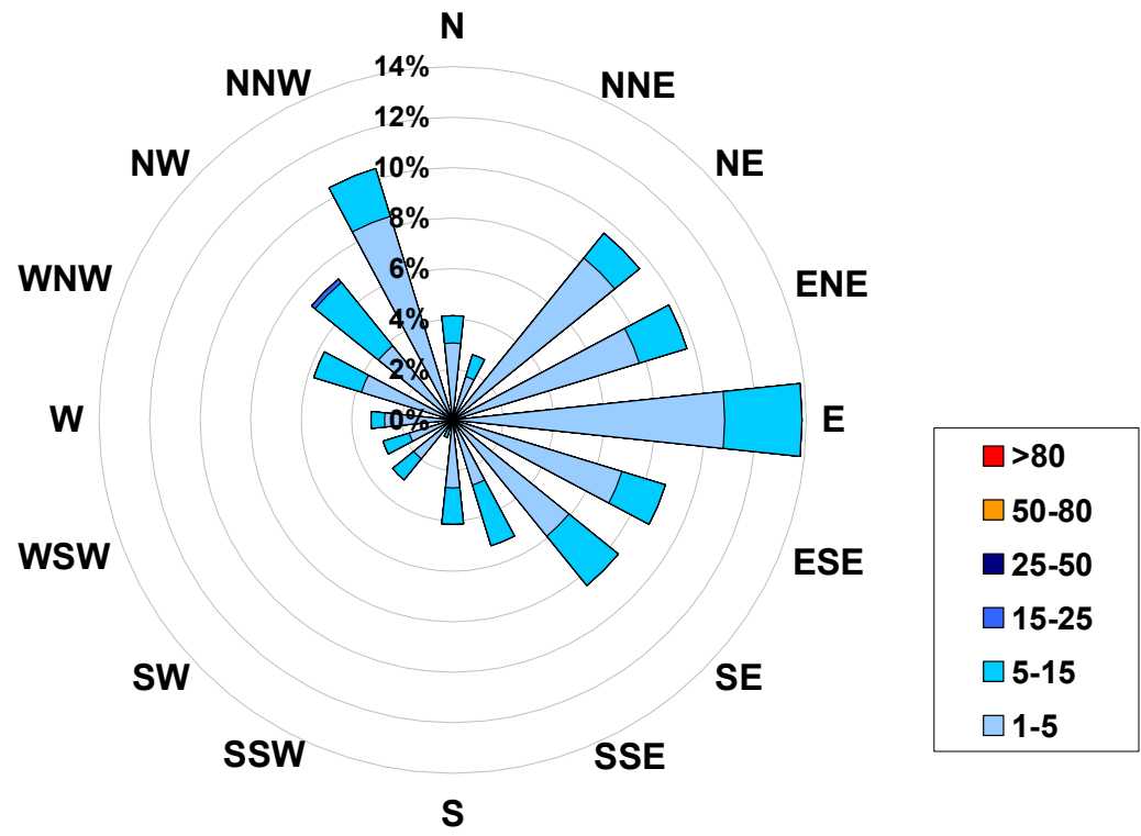
1-hr Average Concentration Rose for Particulate Matter (less than 2.5 microns) (in micrograms per cubic meter) Located at the Beaverlodge Site for June 2005
