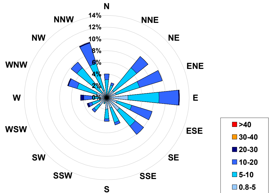
1-hr Average Wind Rose (in km/hr) Located at the Beaverlodge Site for June 2005
