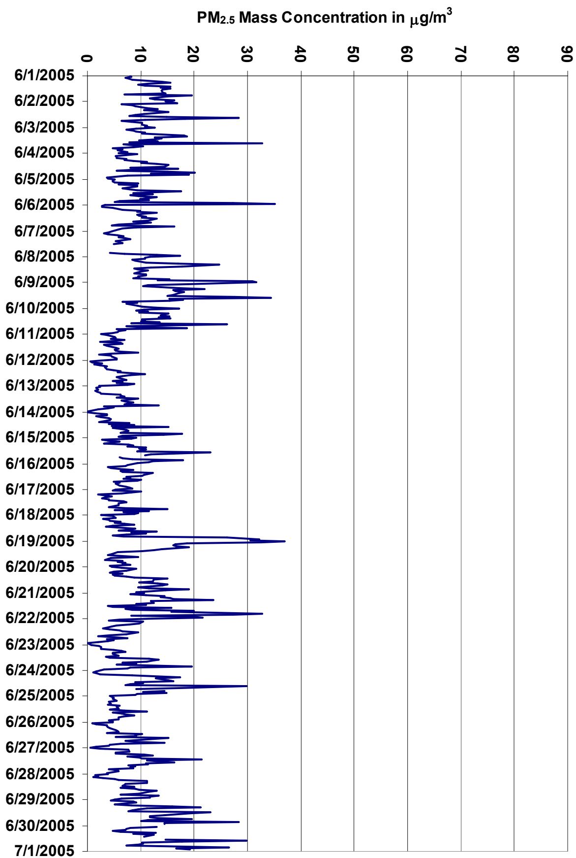
Figure 16. PASZA - Henry Pitker Particulate Matter (less than 2.5 microns) 1-hr Maximum Value Monthly Trend
