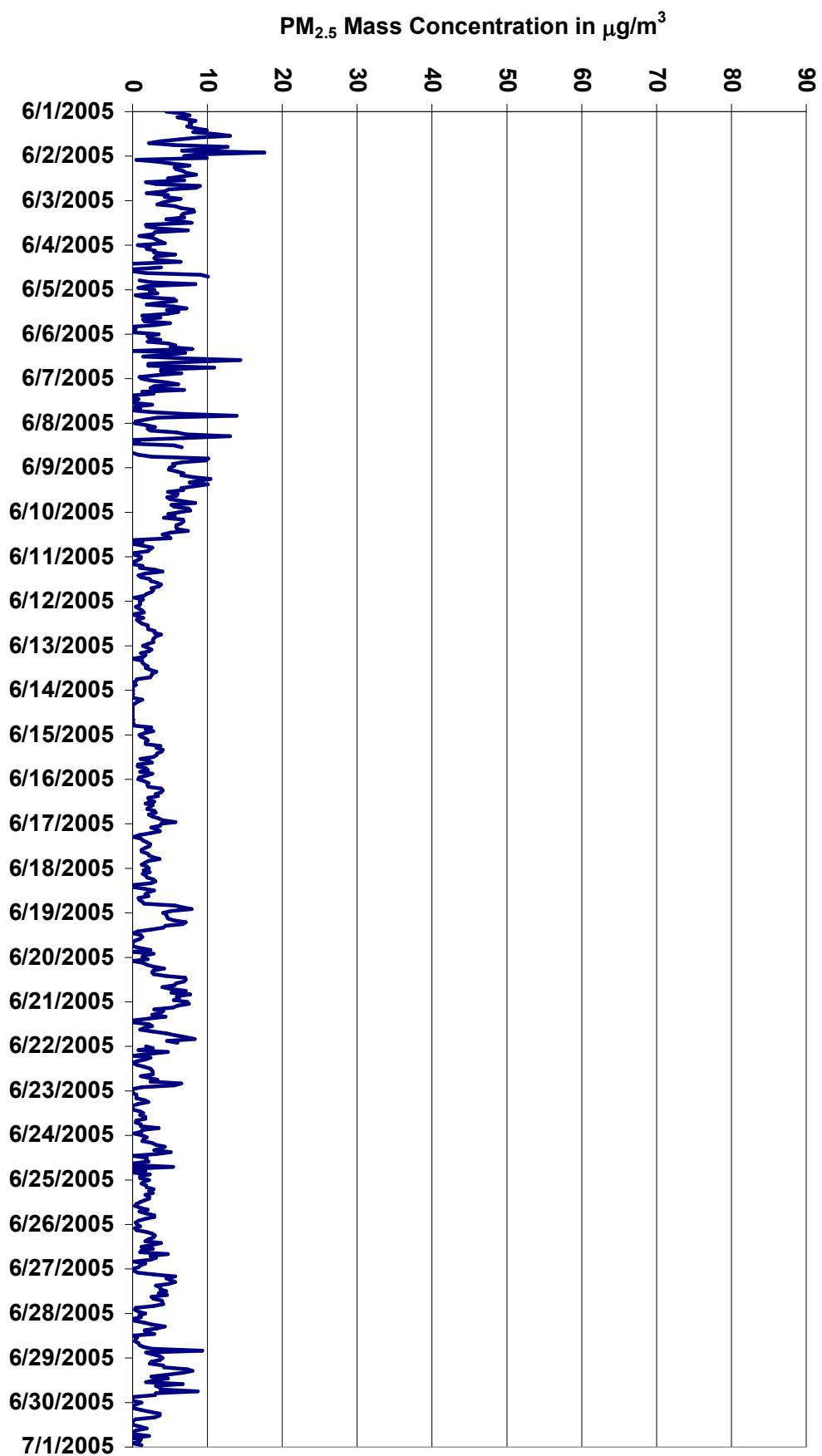
Figure 37. PASZA - Beaverlodge Particulate Matter (less than 2.5 microns) 1-hr Average Monthly Trend
