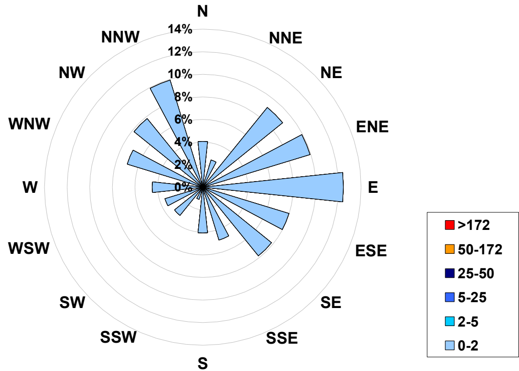
1-hr Average Concentration Rose for Sulphur Dioxide (in ppb) Located at the Beaverlodge Site for June 2005
