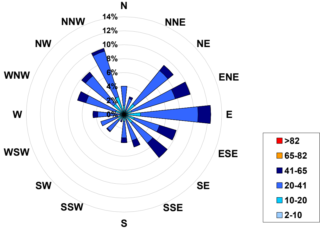
1-hr Average Concentration Rose for Ozone (in ppb) Located at the Beaverlodge Site for June 2005
