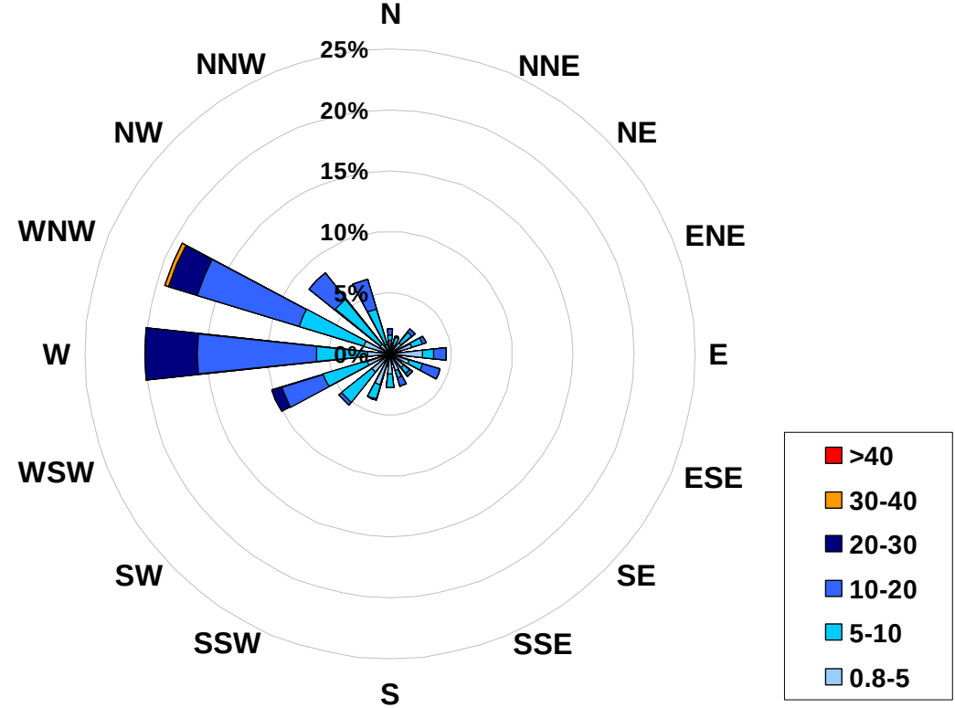
1-hr Average Wind Rose (in km/hr) Located at the Beaverlodge Site for June 2008
