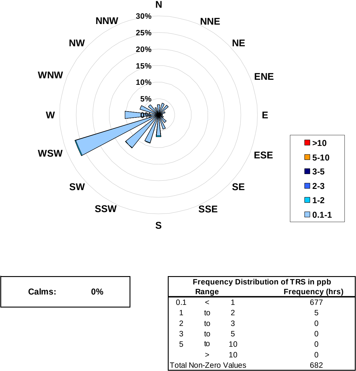
1-hr Average Concentration Rose for Total Reduced Sulphur (in ppb) Located at the Smoky Heights Site for June 2008
