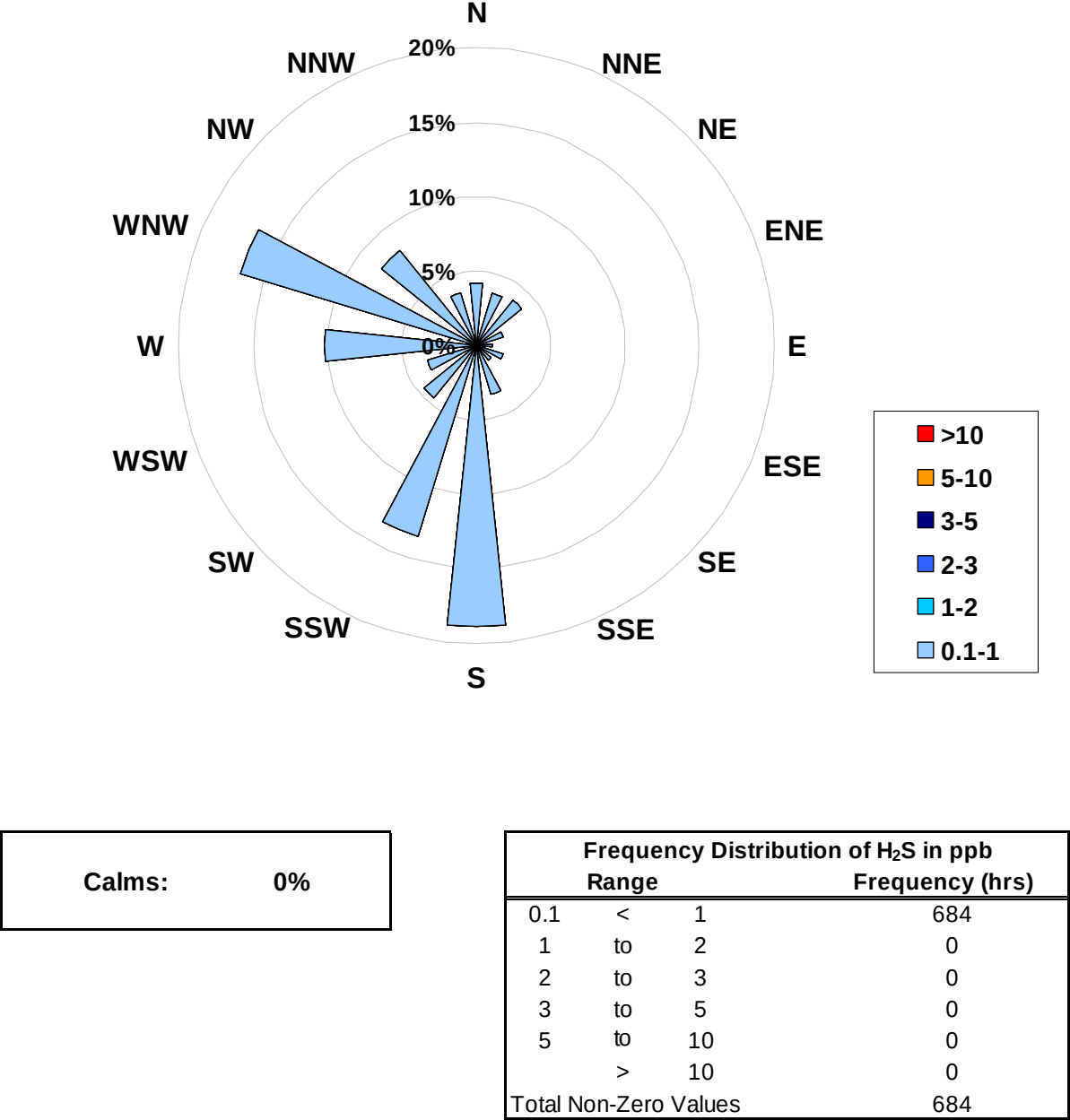
1-hr Average Concentration Rose for Hydrogen Sulphide (in ppb) Located at the Valleyview Site for June 2008
