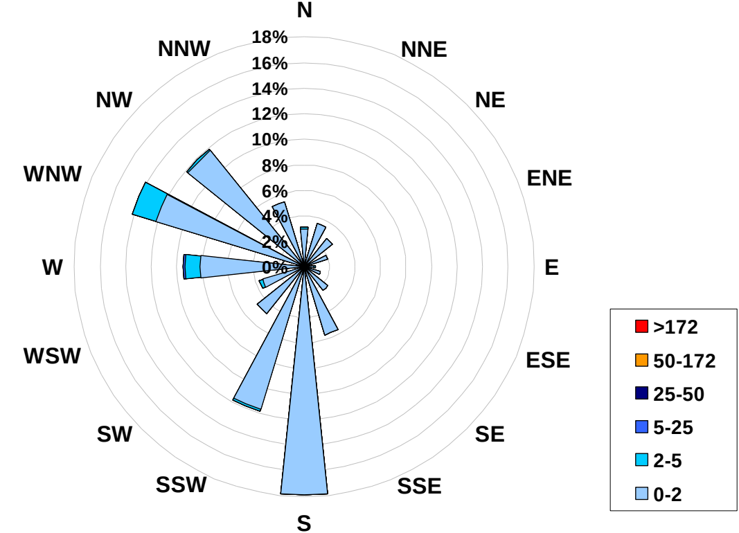
1-hr Average Concentration Rose for Sulphur Dioxide (in ppb) Located at the Valleyview Site for June 2008
