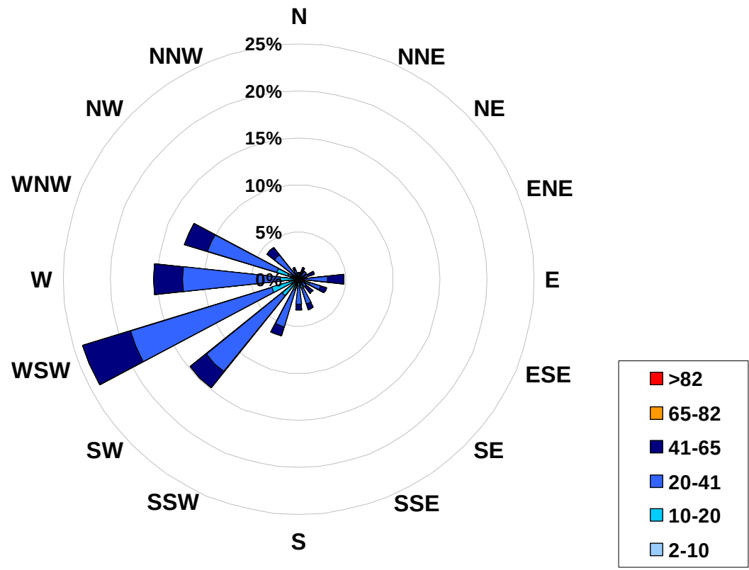
1-hr Average Concentration Rose for Ozone (in ppb) Located at the Henry Pirker Site for June 2008
