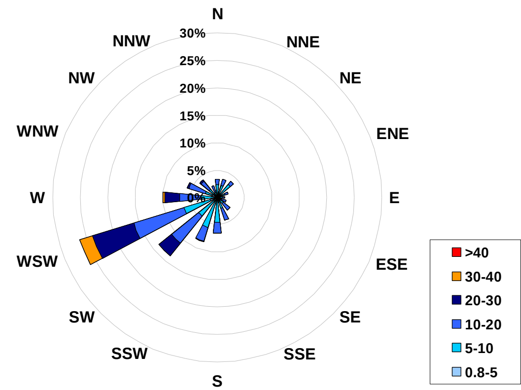
1-hr Average Wind Rose (in km/hr) Located at the Smoky Heights Site for June 2008
