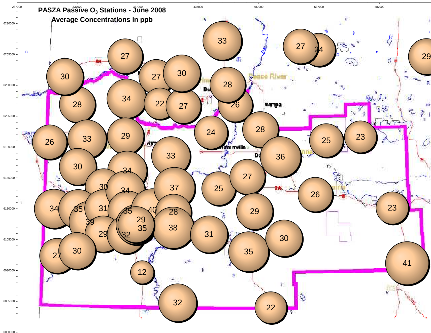
Figure 67. O 3 Bubble Chart
