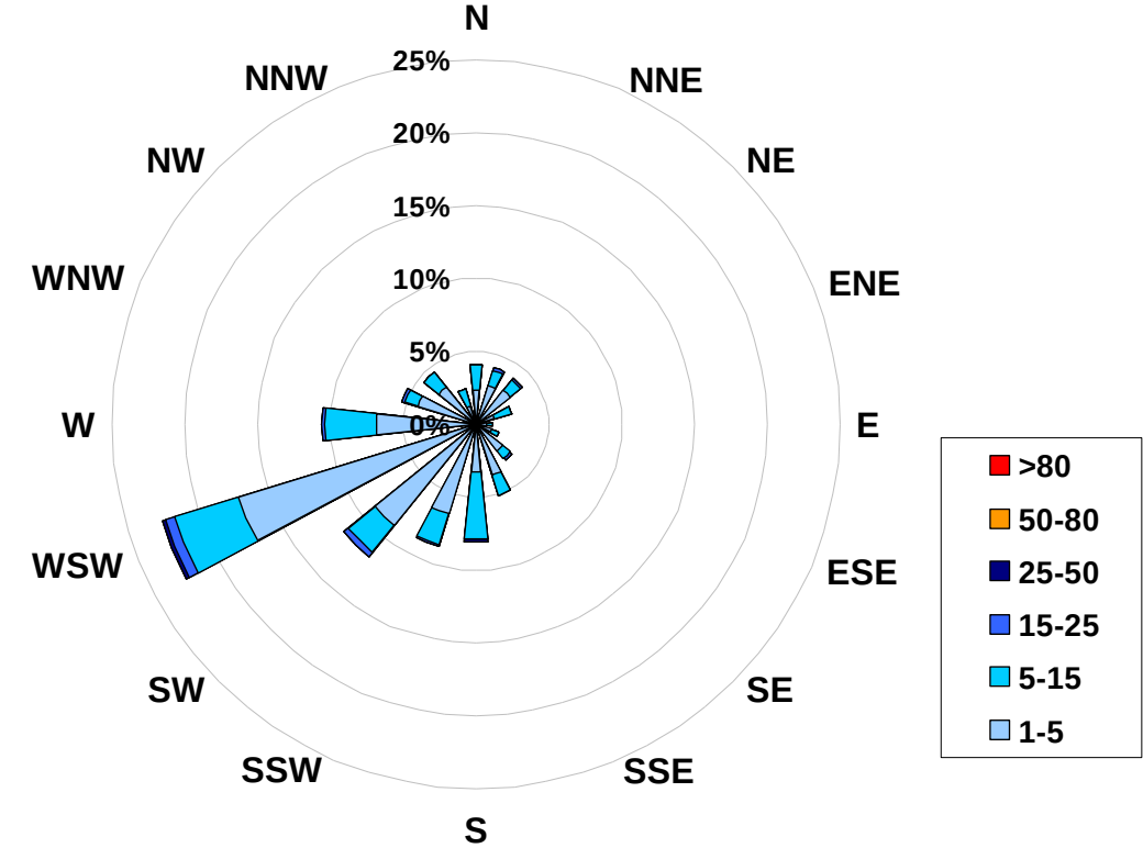
1-hr Average Concentration Rose for Particulate Matter (less than 2.5 microns) (in micrograms per cubic meter) Located at the Smoky Heights Site for June 2008
