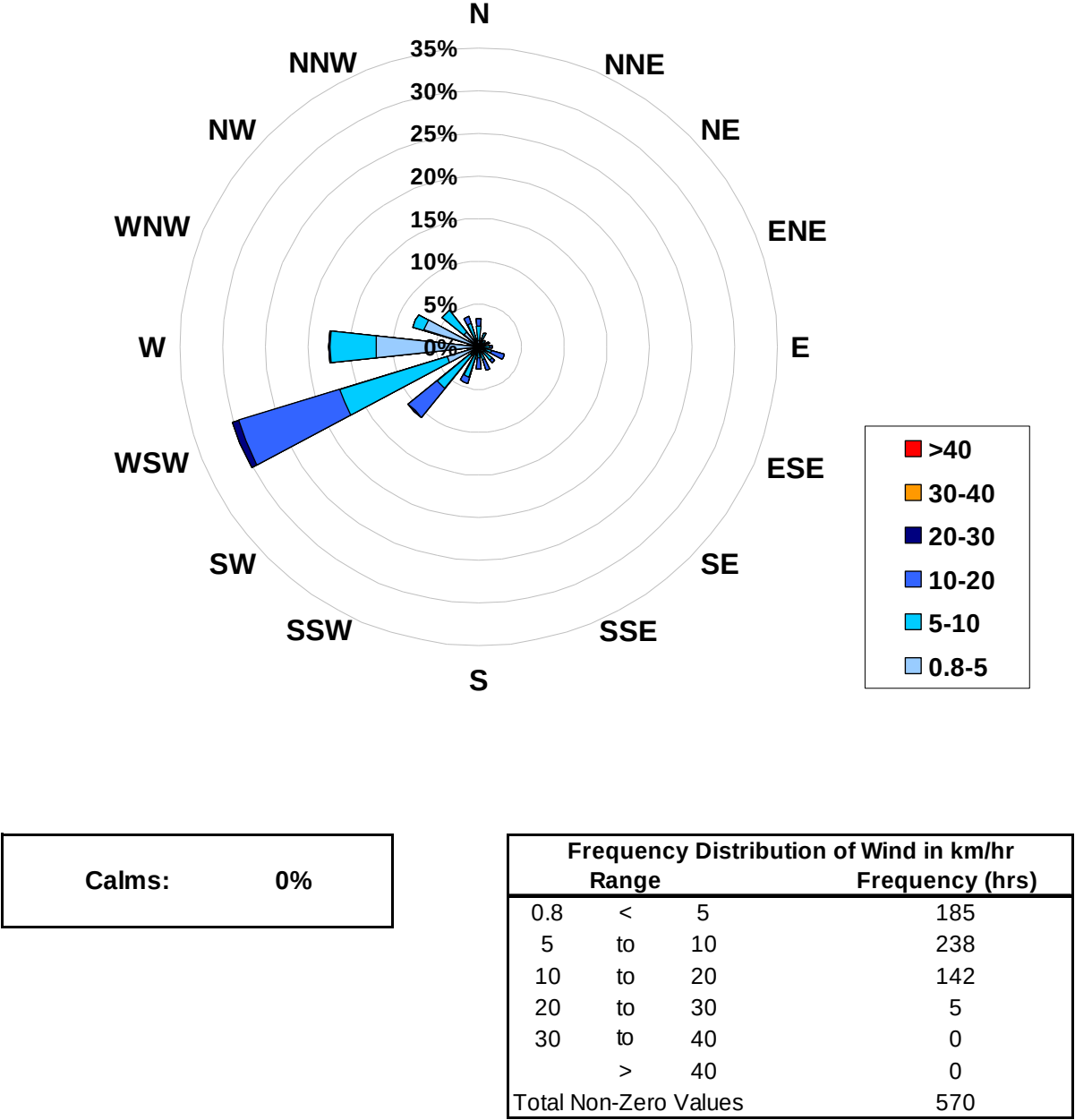
1-hr Average Wind Rose (in km/hr) Located at the Portable-Spirit River Site for June 2008
