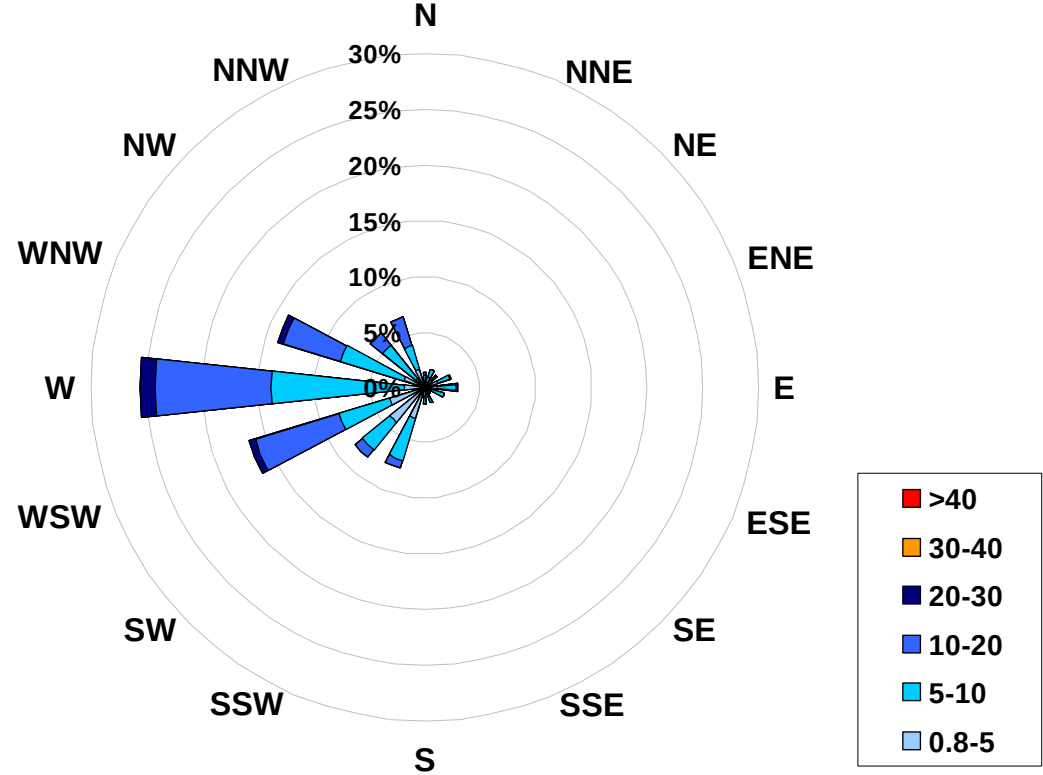
1-hr Average Wind Rose (in km/hr) Located at the Evergreen Park Site for June 2008
