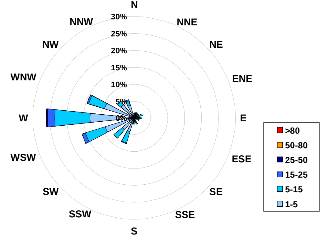
1-hr Average Concentration Rose for Particulate Matter (less than 2.5 microns) (in micrograms per cubic meter) Located at the Evergreen Park Site for June 2008
