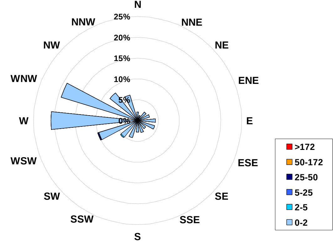
1-hr Average Concentration Rose for Sulphur Dioxide (in ppb) Located at the Beaverlodge Site for June 2008
