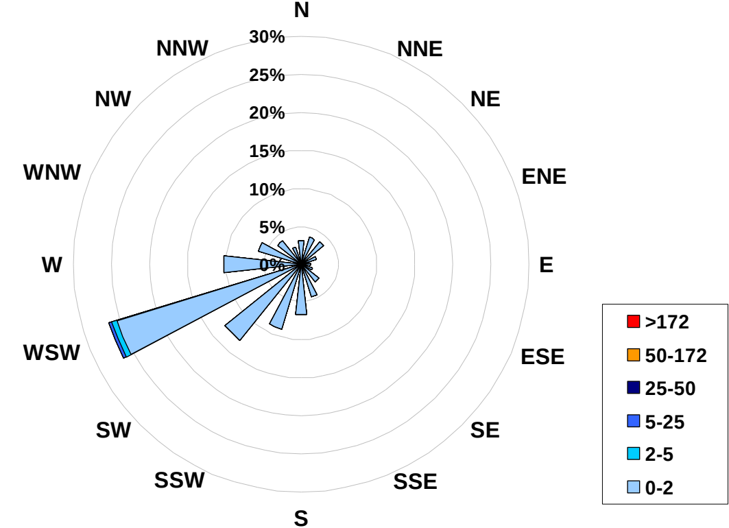
1-hr Average Concentration Rose for Sulphur Dioxide (in ppb) Located at the Smoky Heights Site for June 2008
