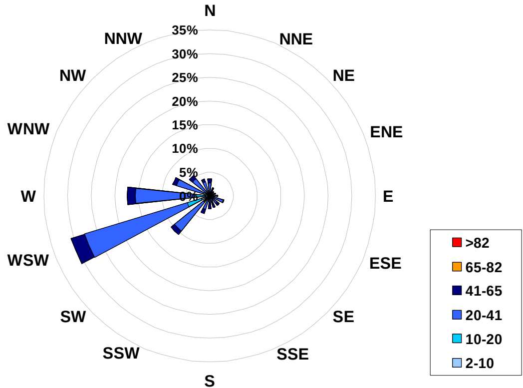
1-hr Average Concentration Rose for Ozone (in ppb) Located at the Portable-Spirit River Site for June 2008
