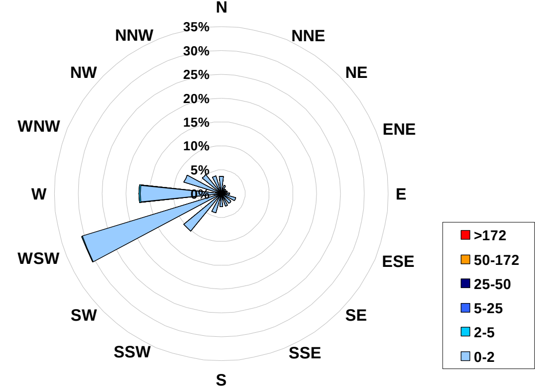
1-hr Average Concentration Rose for Sulphur Dioxide (in ppb) Located at the Portable-Spirit River Site for June 2008
