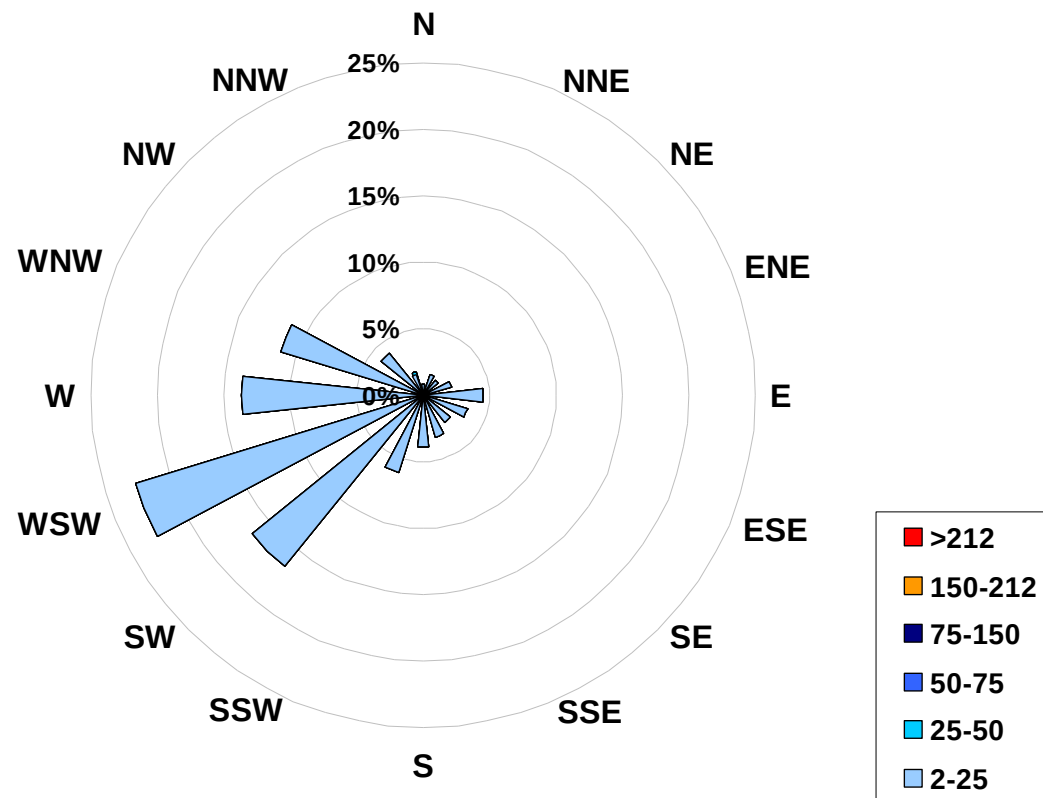
1-hr Average Concentration Rose for Nitrogen Dioxide (in ppb) Located at the Henry Pirker Site for June 2008
