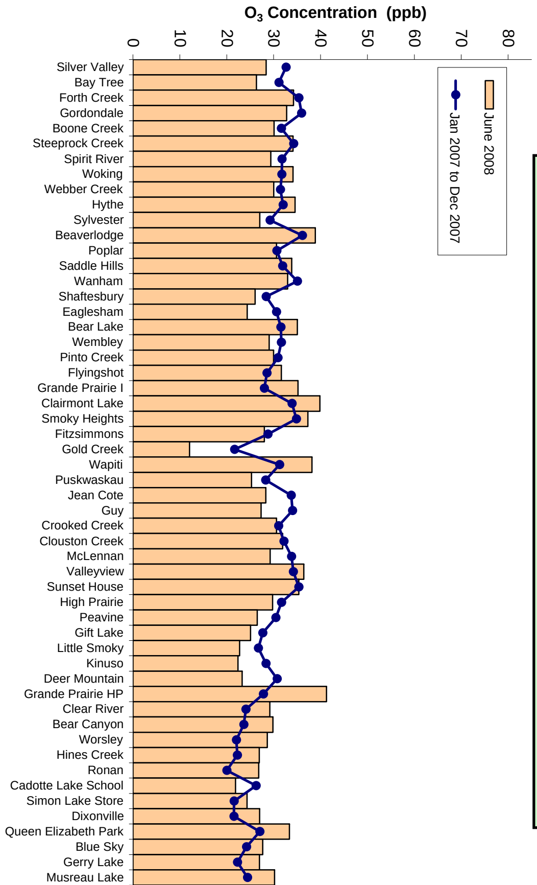
Figure 68. O 3 Summary Chart
