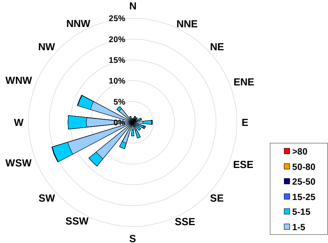
1-hr Average Concentration Rose for Particulate Matter (less than 2.5 microns) (in micrograms per cubic meter) Located at the Henry Pirker Site for June 2008
