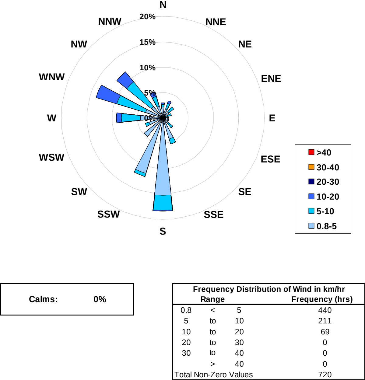
1-hr Average Wind Rose (in km/hr) Located at the Valleyview Site for June 2008
