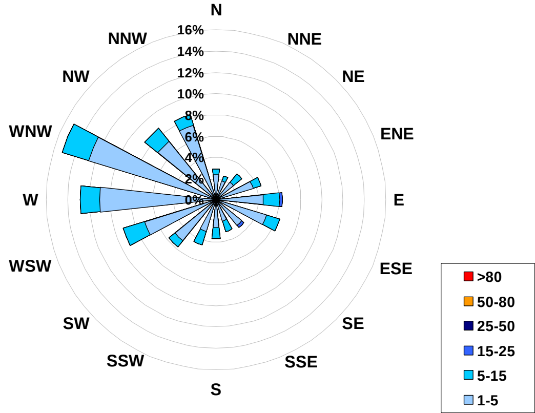
1-hr Average Concentration Rose for Particulate Matter (less than 2.5 microns) (in micrograms per cubic meter) Located at the Beaverlodge Site for June 2008
