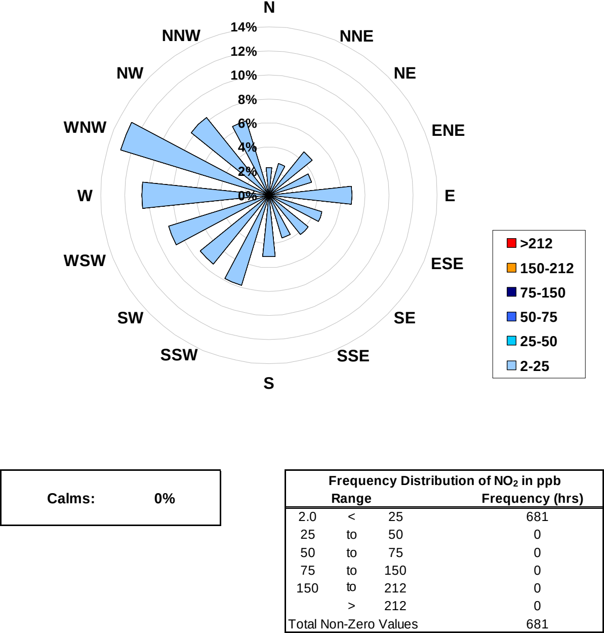
1-hr Average Concentration Rose for Nitrogen Dioxide (in ppb) Located at the Beaverlodge Site for June 2008
