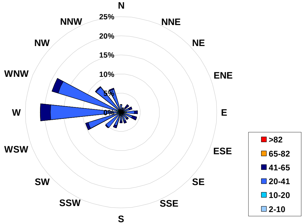
1-hr Average Concentration Rose for Ozone (in ppb) Located at the Beaverlodge Site for June 2008
