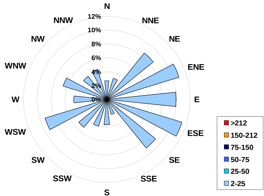
1-hr Average Concentration Rose for Nitrogen Dioxide (in ppb) Located at the Beaverlodge Site for March 2008
