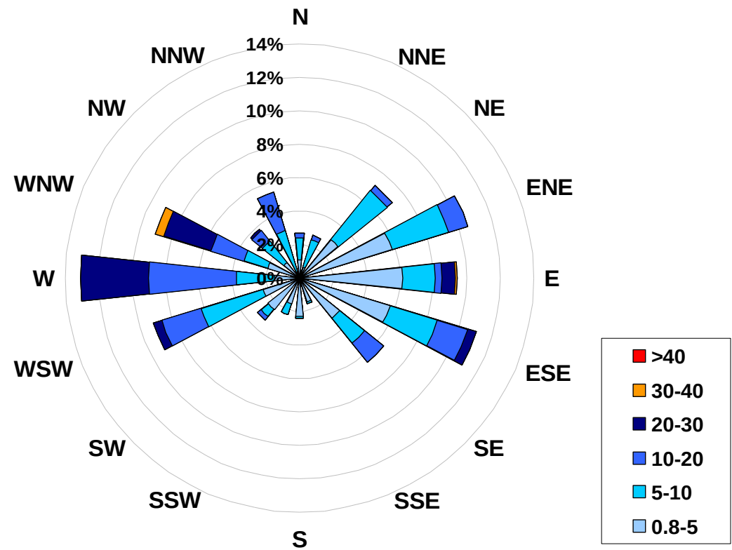
1-hr Average Wind Rose (in km/hr) Located at the Beaverlodge Site for March 2008
