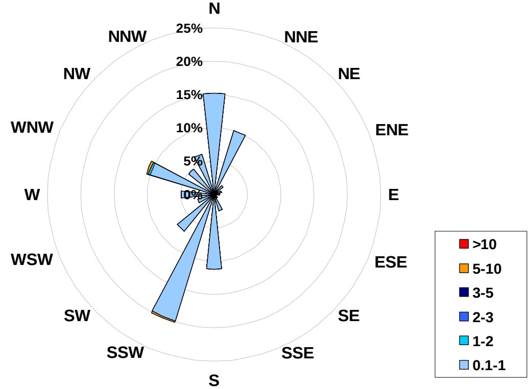
1-hr Average Concentration Rose for Hydrogen Sulphide (in ppb) Located at the Valleyview Site for March 2008
