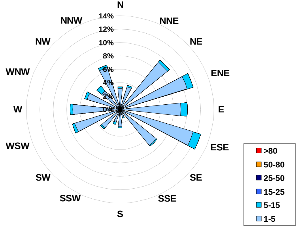
1-hr Average Concentration Rose for Particulate Matter (less than 2.5 microns) (in micrograms per cubic meter) Located at the Beaverlodge Site for March 2008
