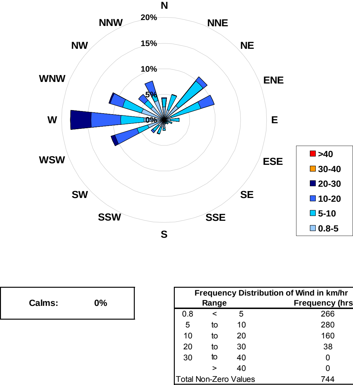
1-hr Average Wind Rose (in km/hr) Located at the Evergreen Park Site for March 2008
