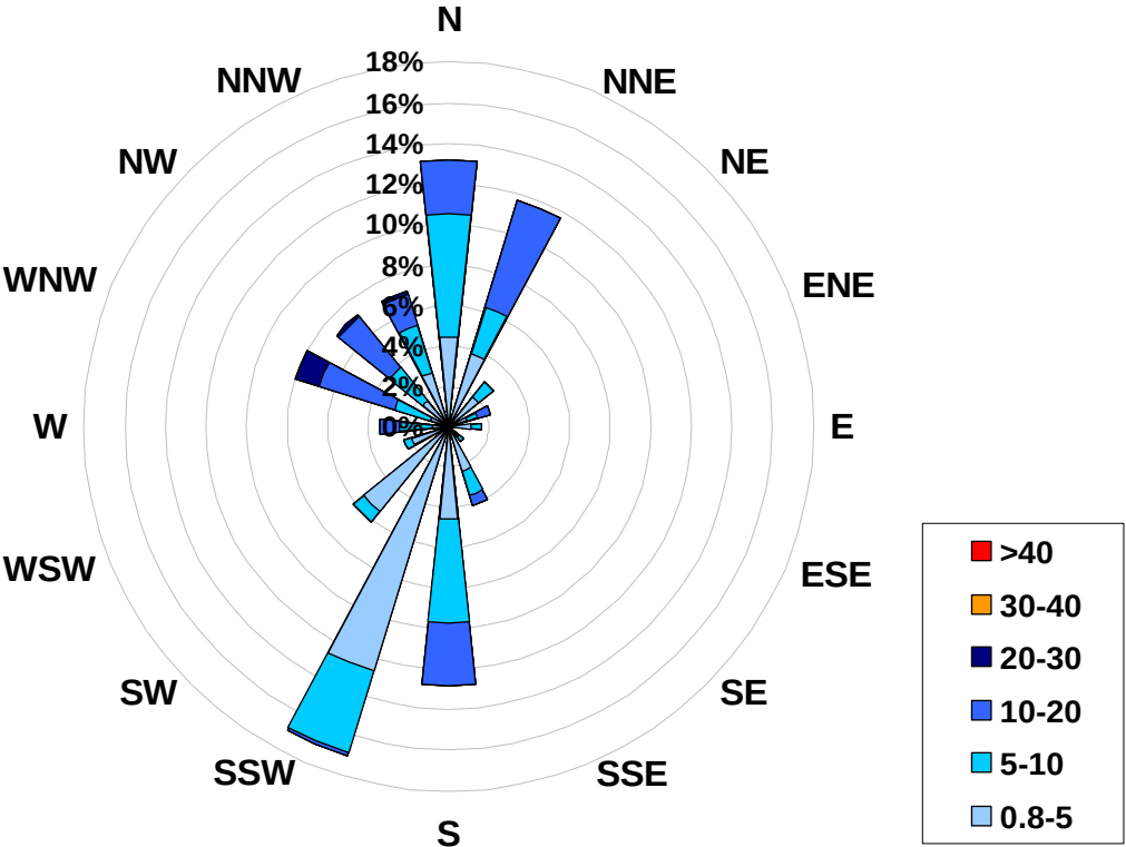
1-hr Average Wind Rose (in km/hr) Located at the Valleyview Site for March 2008
