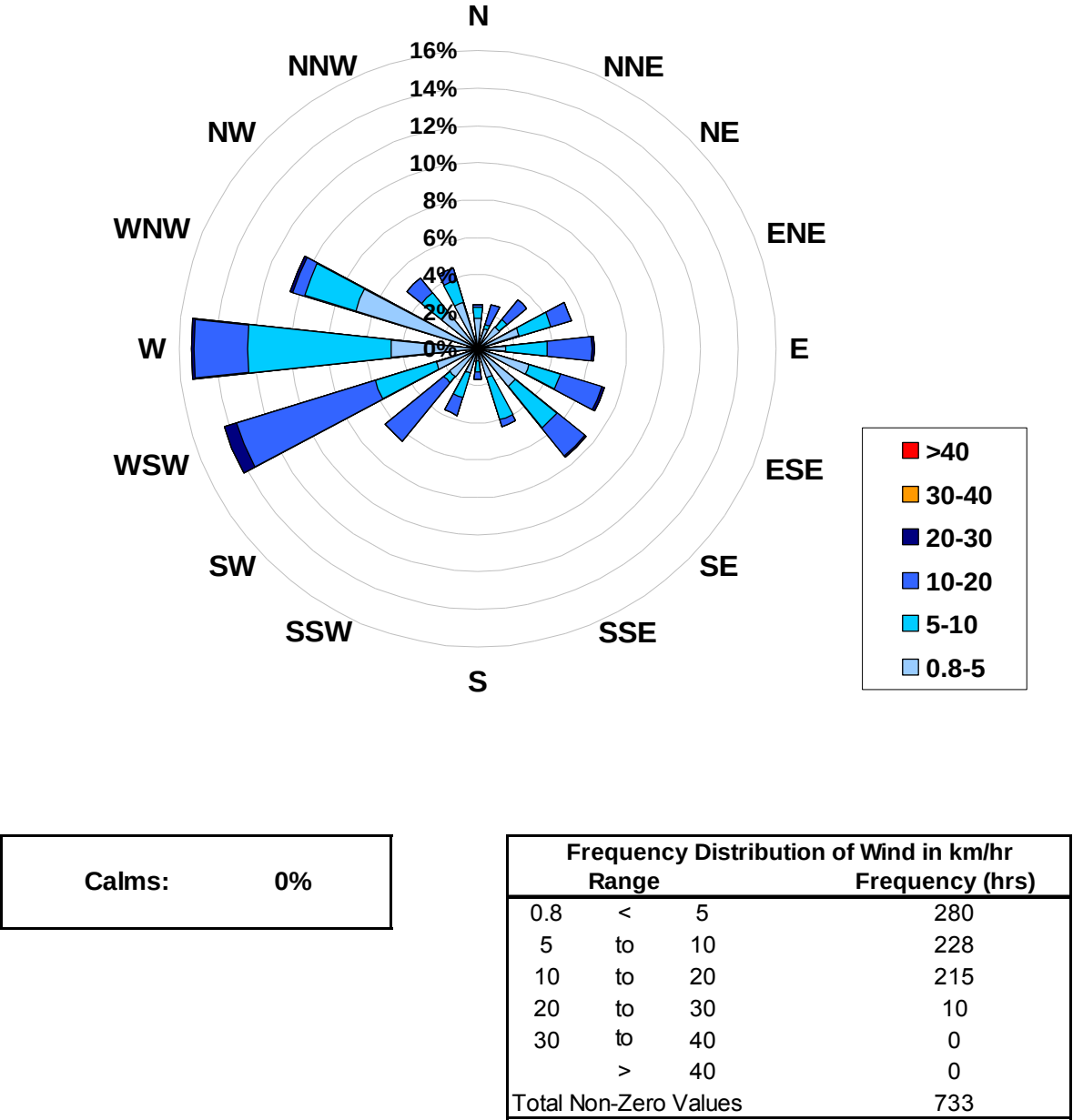
1-hr Average Wind Rose (in km/hr) Located at the Portable-Spirit River Site for March 2008
