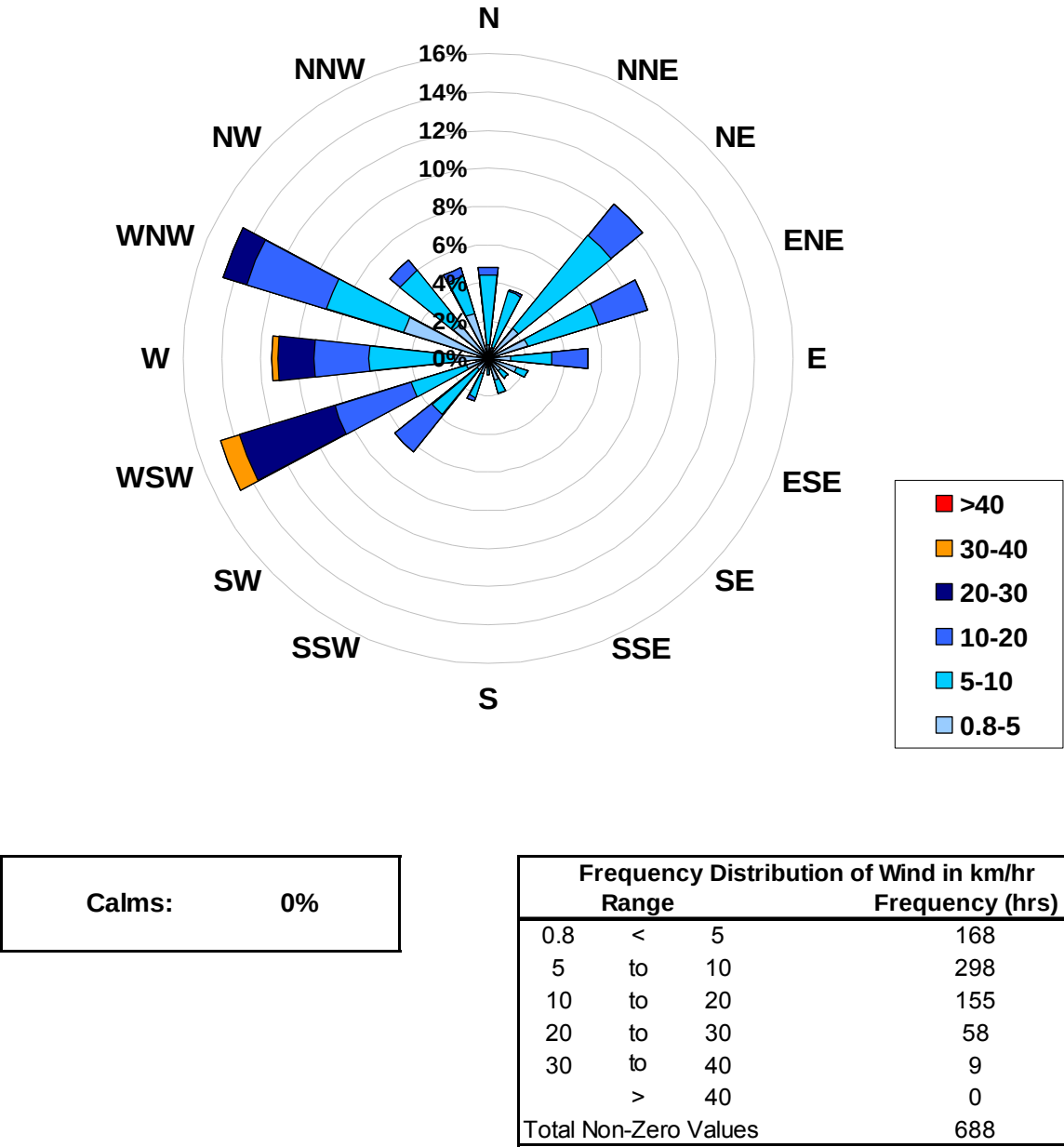
1-hr Average Wind Rose (in km/hr) Located at the Henry Pirker Site for March 2008
