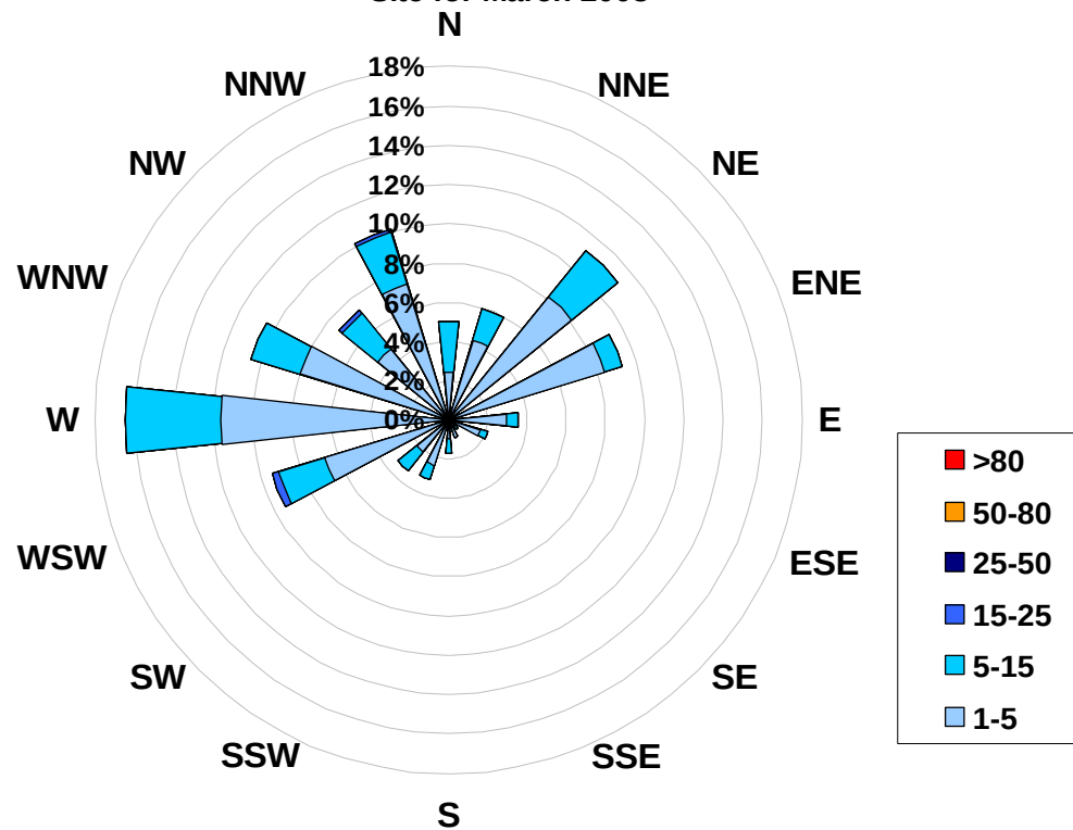
1-hr Average Concentration Rose for Particulate Matter (less than 2.5 microns) (in micrograms per cubic meter) Located at the Evergreen Park Site for March 2008
