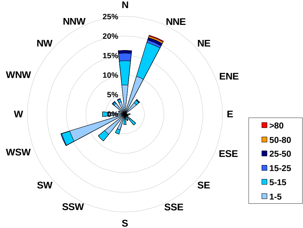
1-hr Average Concentration Rose for Particulate Matter (less than 2.5 microns) (in micrograms per cubic meter) Located at the Smoky Heights Site for March 2008
