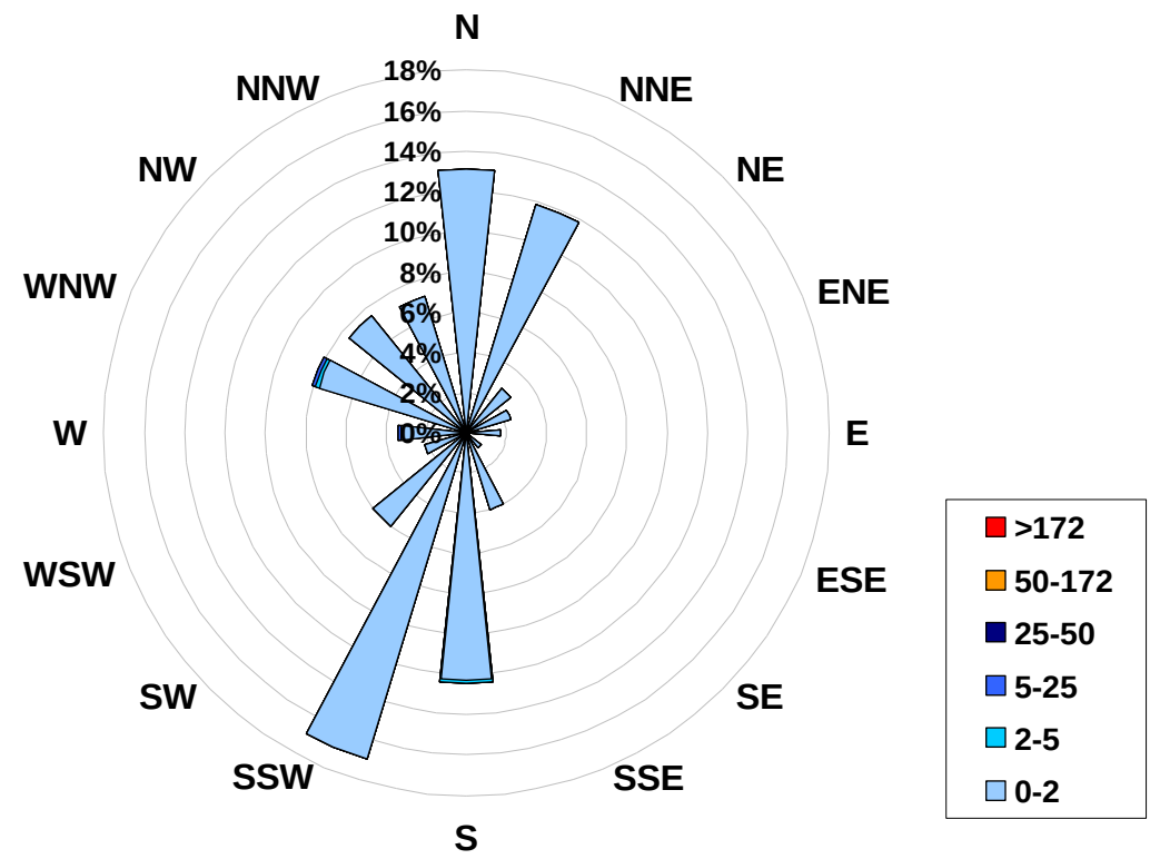
1-hr Average Concentration Rose for Sulphur Dioxide (in ppb) Located at the Valleyview Site for March 2008
