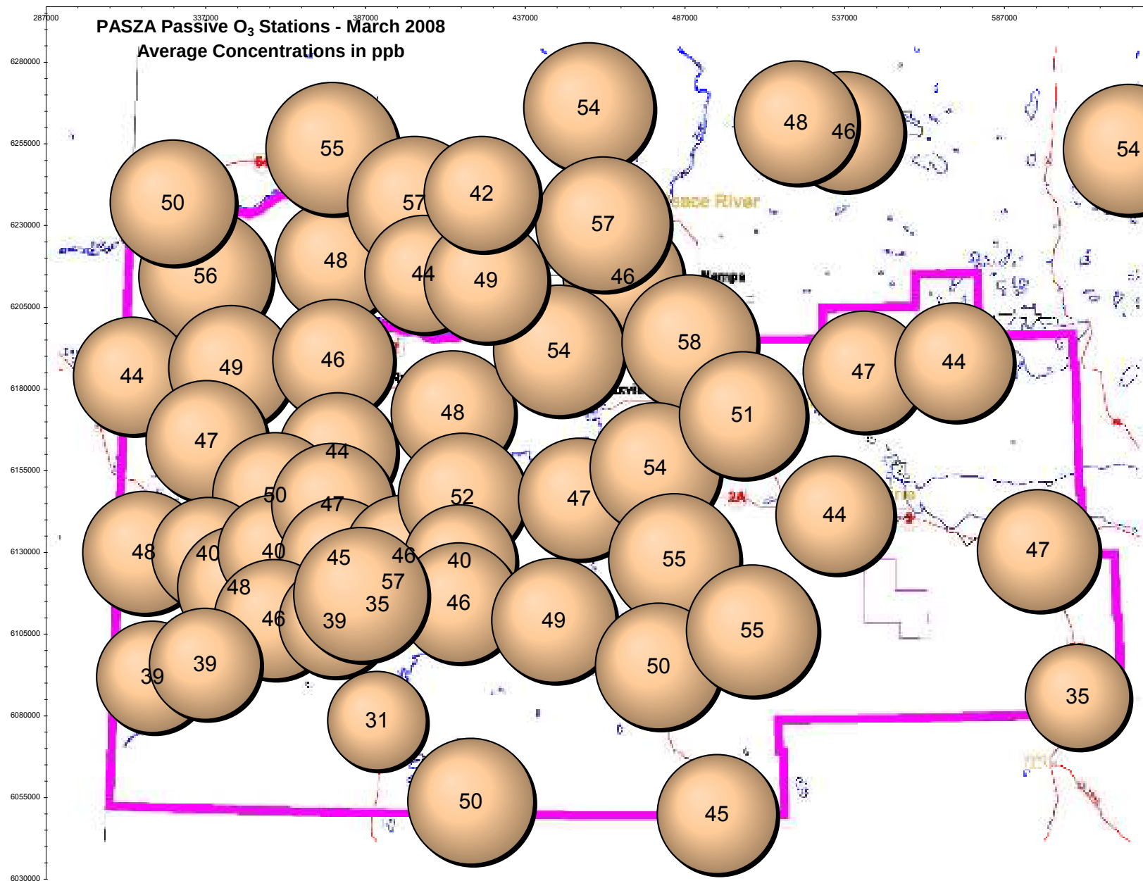
Figure 64. O 3 Bubble Chart
