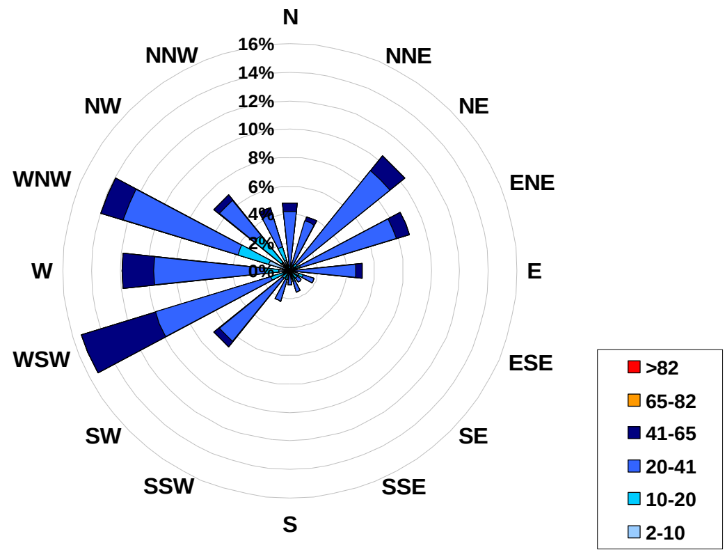
1-hr Average Concentration Rose for Ozone (in ppb) Located at the Henry Pirker Site for March 2008
