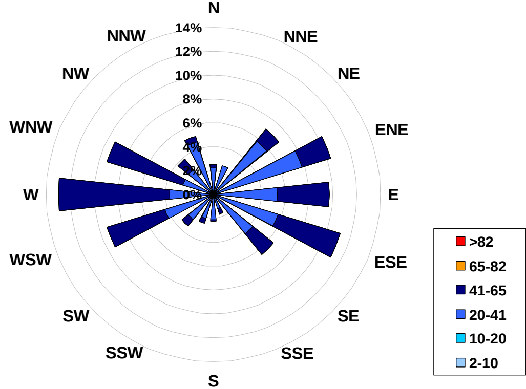
1-hr Average Concentration Rose for Ozone (in ppb) Located at the Beaverlodge Site for March 2008
