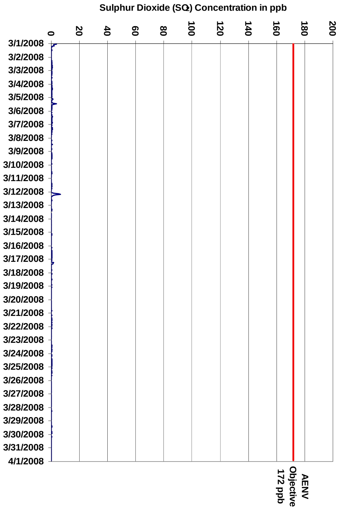
Figure 56. PASZA - Valleyview Sulphur Dioxide 1-hr Average Monthly Trend
