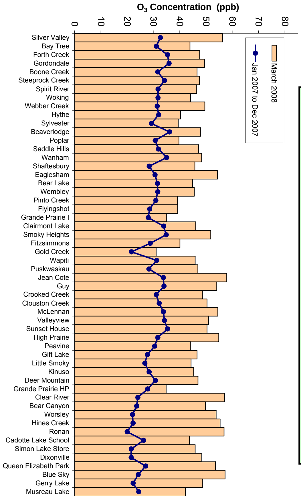
Figure 65. O 3 Summary Chart
