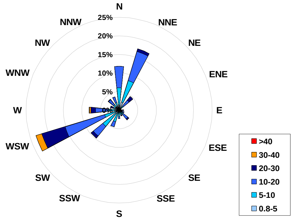
1-hr Average Wind Rose (in km/hr) Located at the Smoky Heights Site for March 2008
