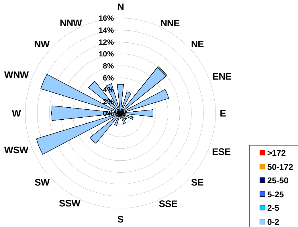
1-hr Average Concentration Rose for Sulphur Dioxide (in ppb) Located at the Henry Pirker Site for March 2008
