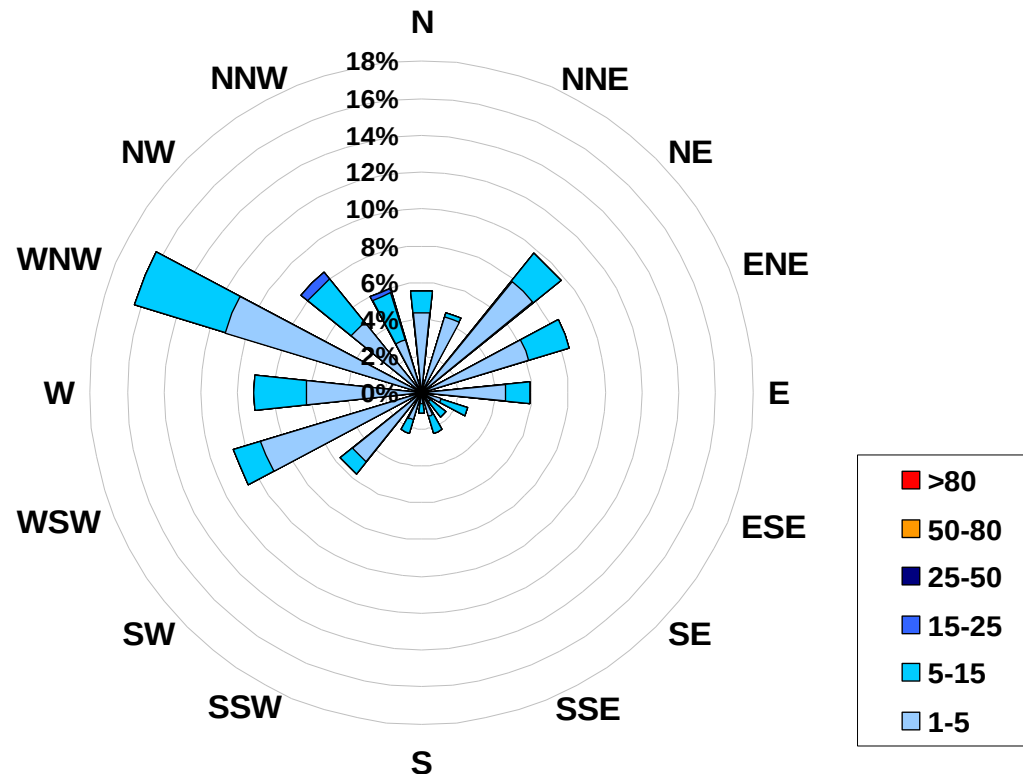
1-hr Average Concentration Rose for Particulate Matter (less than 2.5 microns) (in micrograms per cubic meter) Located at the Henry Pirker Site for March 2008
