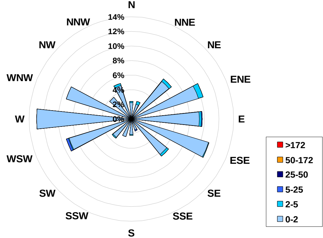
1-hr Average Concentration Rose for Sulphur Dioxide (in ppb) Located at the Beaverlodge Site for March 2008
