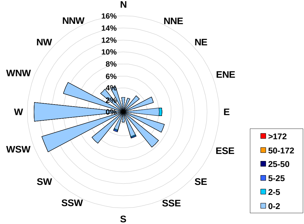
1-hr Average Concentration Rose for Sulphur Dioxide (in ppb) Located at the Portable-Spirit River Site for March 2008
