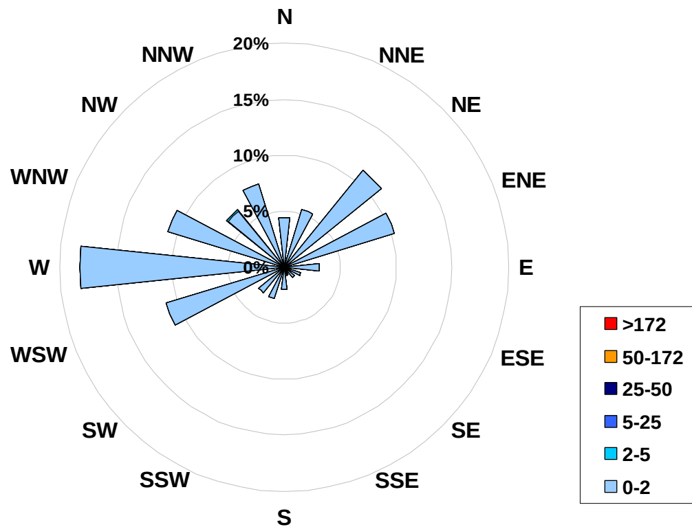
1-hr Average Concentration Rose for Sulphur Dioxide (in ppb) Located at the Evergreen Park Site for March 2008
