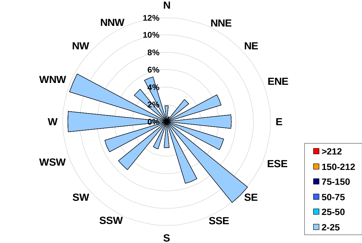
1-hr Average Concentration Rose for Nitrogen Dioxide (in ppb) Located at the Portable-Spirit River Site for March 2008
