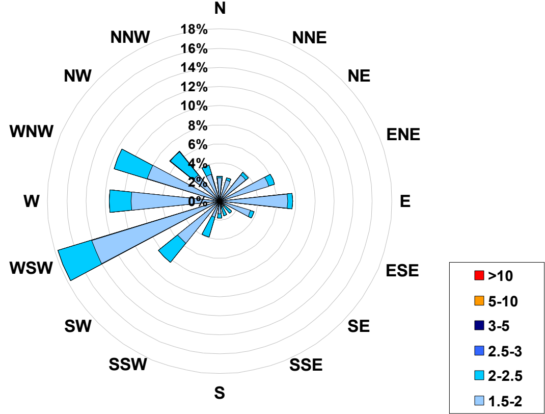
1-hr Average Concentration Rose for Total Hydrocarbons (in ppm) Located at the Henry Pirker Site for May 2006
