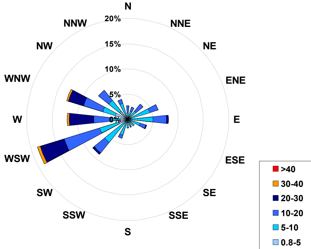
1-hr Average Wind Rose (in km/hr) Located at the Henry Pirker Site for May 2006
