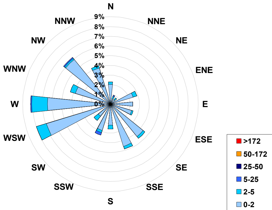
1-hr Average Concentration Rose for Sulphur Dioxide (in ppb) Located at the Evergreen Park Site for May 2006
