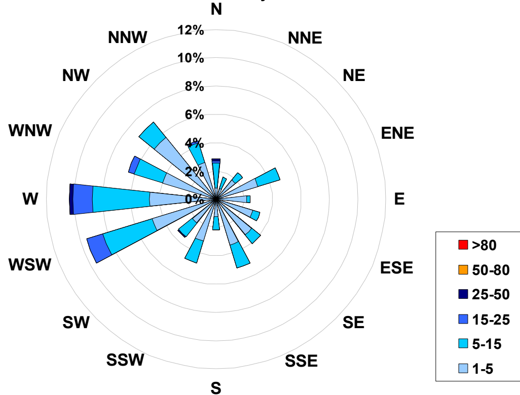
1-hr Average Concentration Rose for Particulate Matter (less than 2.5 microns) (in micrograms per cubic meter) Located at the Evergreen Park Site for May 2006
