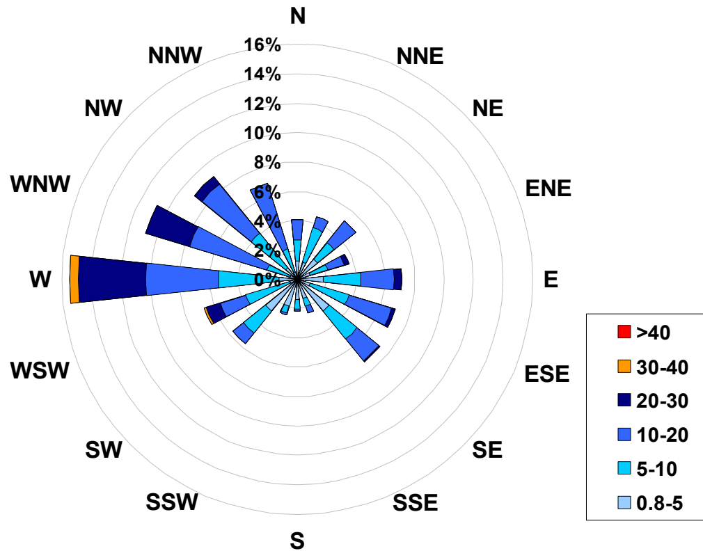
1-hr Average Wind Rose (in km/hr) Located at the Beaverlodge Site for May 2006
