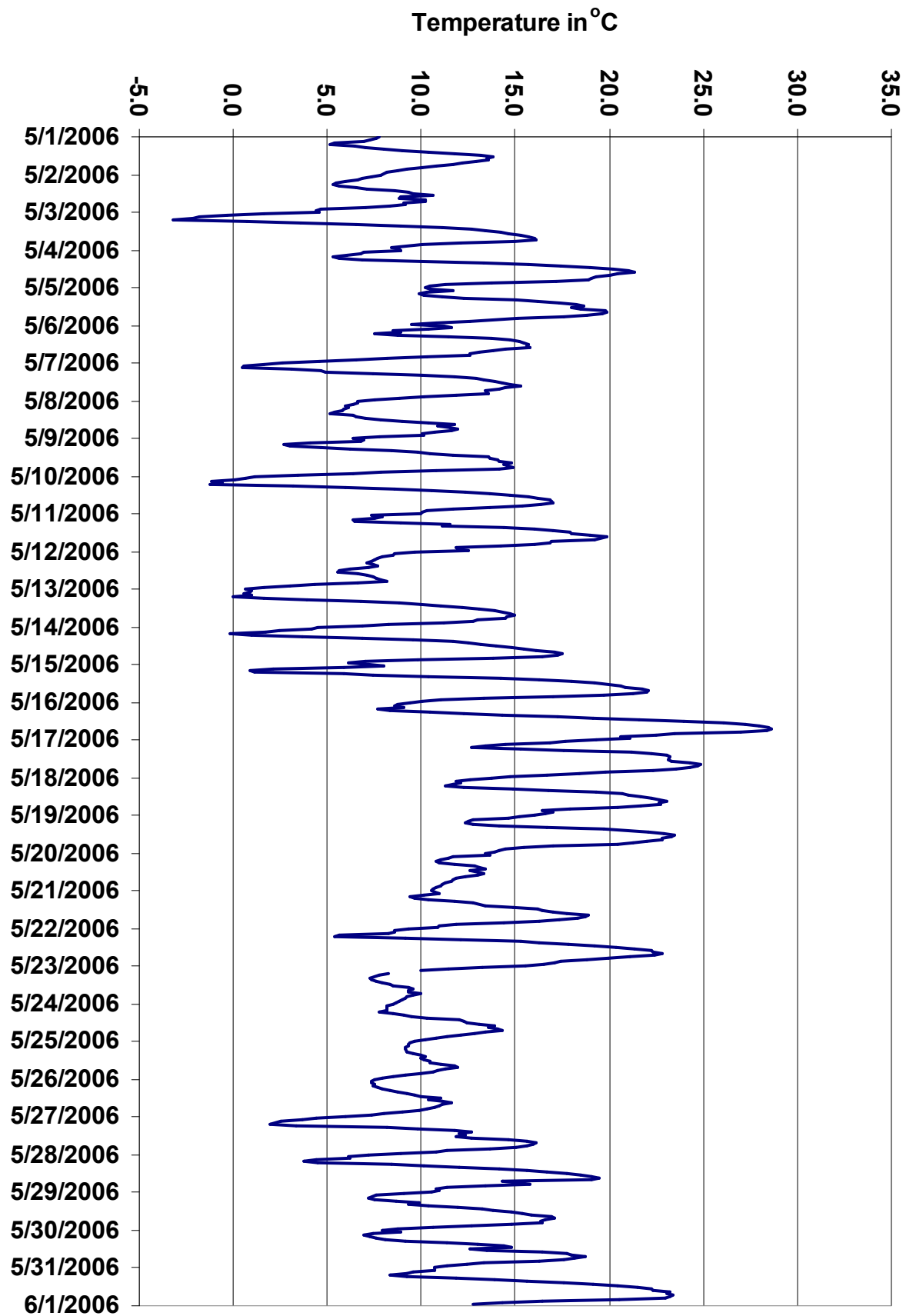
Figure 33. PASZA - Smoky Heights Temperature 1-hr Average Monthly Trend
