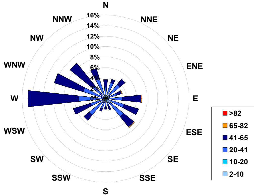
1-hr Average Concentration Rose for Ozone (in ppb) Located at the Beaverlodge Site for May 2006
