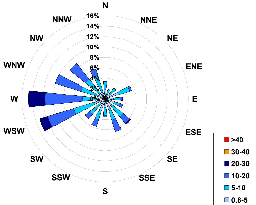
1-hr Average Wind Rose (in km/hr) Located at the Evergreen Park Site for May 2006
