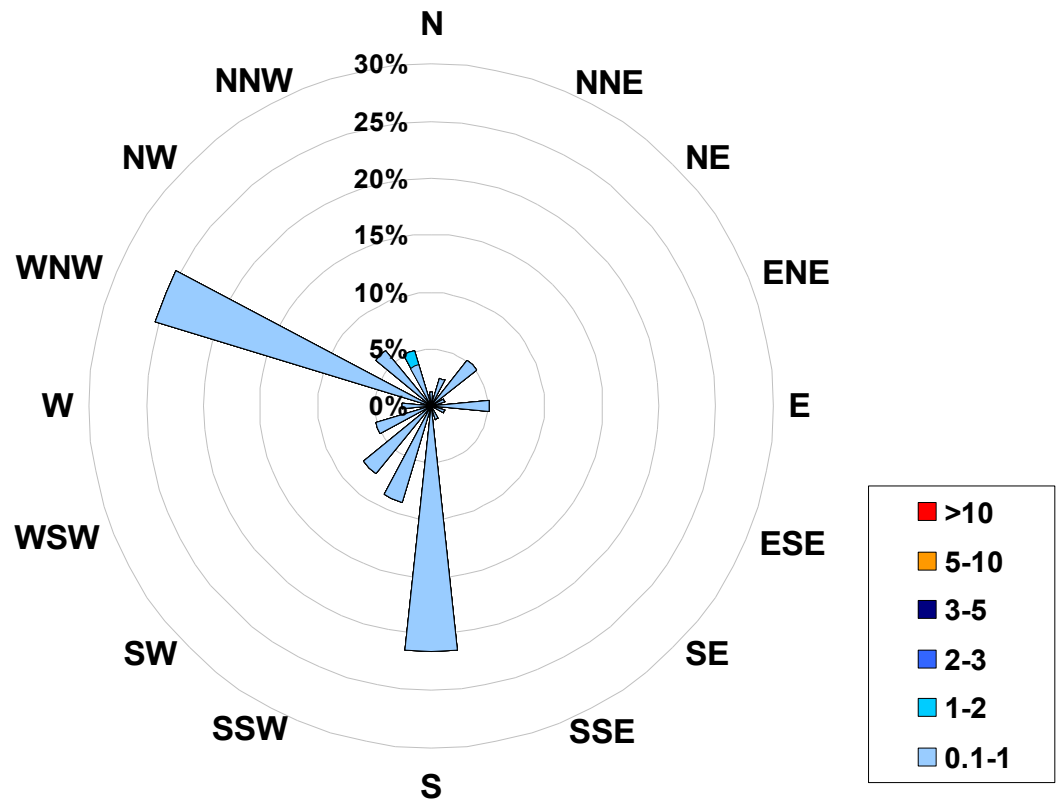
1-hr Average Concentration Rose for Hydrogen Sulphide (in ppb) Located at the Valleyview Site for May 2007
