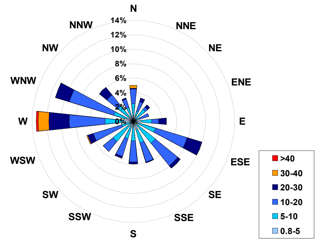
1-hr Average Wind Rose (in km/hr) Located at the Portable-Falher Site for May 2007
