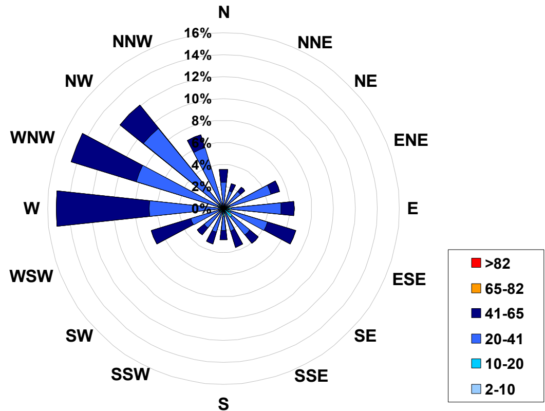
1-hr Average Concentration Rose for Ozone (in ppb) Located at the Beaverlodge Site for May 2007
