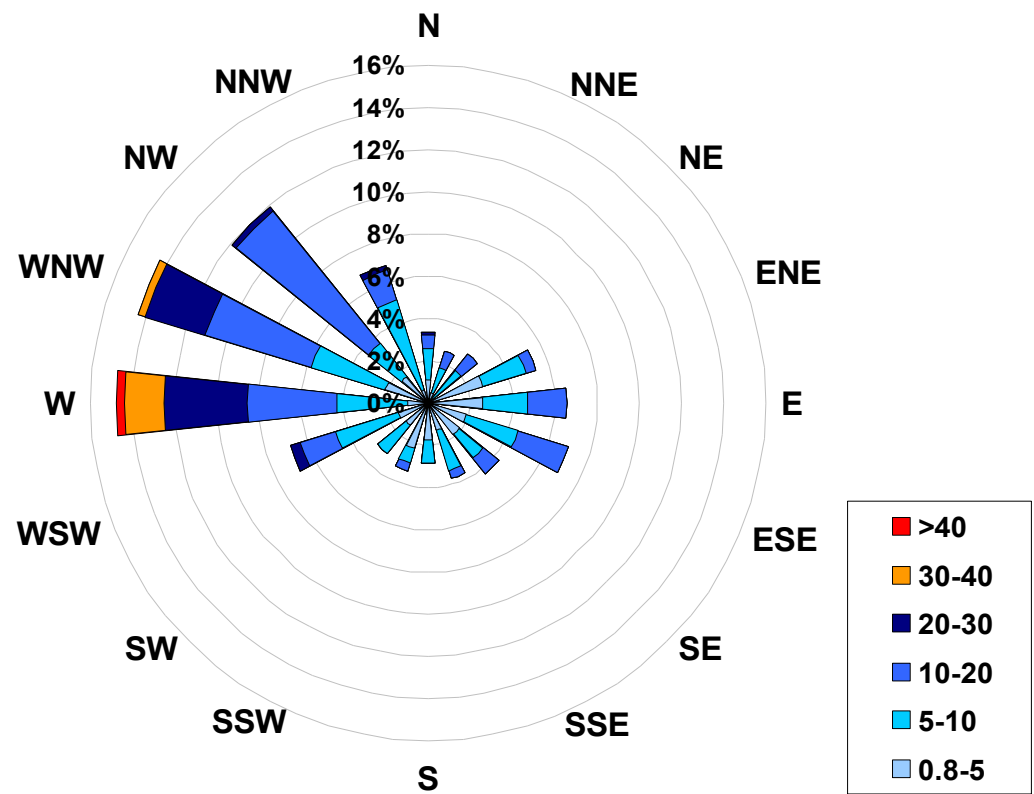
1-hr Average Wind Rose (in km/hr) Located at the Beaverlodge Site for May 2007
