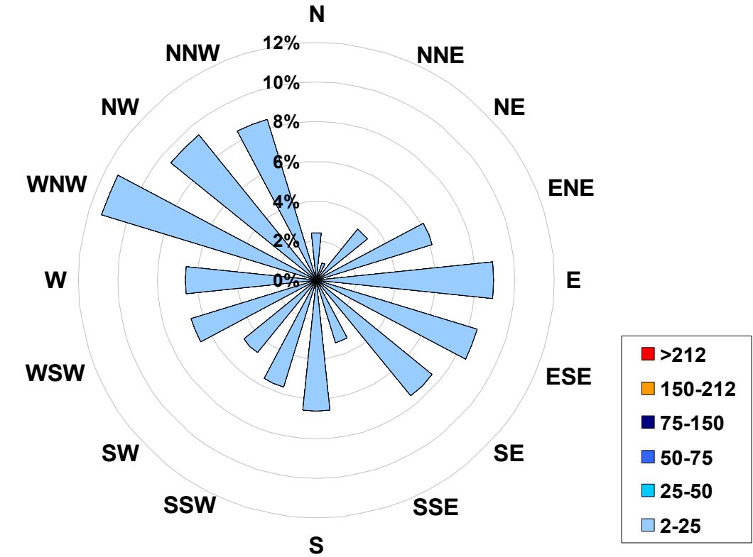
1-hr Average Concentration Rose for Nitrogen Dioxide (in ppb) Located at the Beaverlodge Site for May 2007
