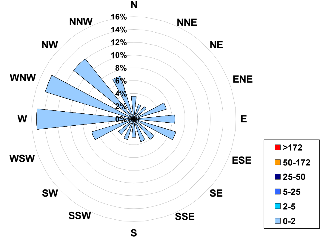
1-hr Average Concentration Rose for Sulphur Dioxide (in ppb) Located at the Beaverlodge Site for May 2007
