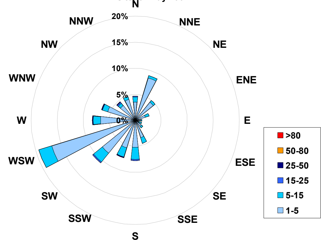
1-hr Average Concentration Rose for Particulate Matter (less than 2.5 microns) (in micrograms per cubic meter) Located at the Smoky Heights Site for May 2007
