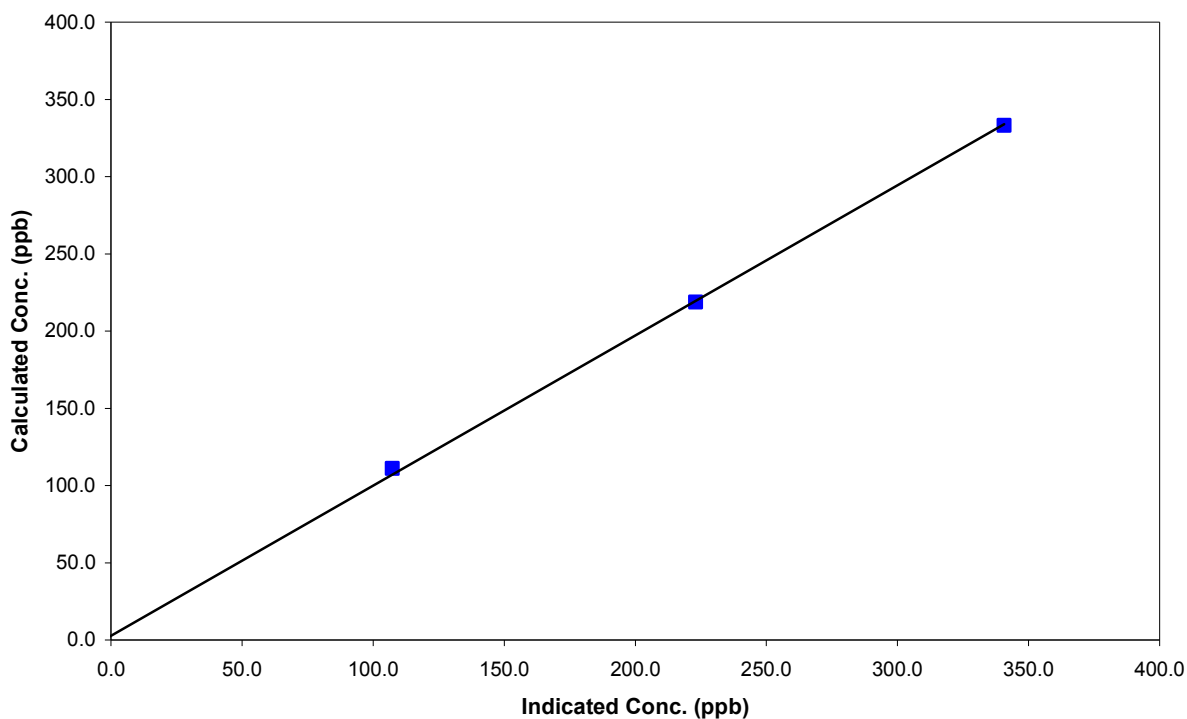
NO 2 Calibration Curve
