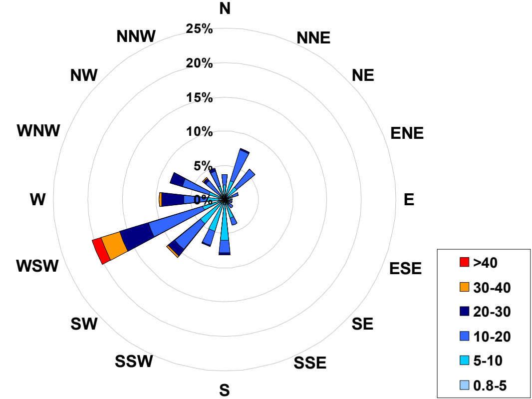
1-hr Average Wind Rose (in km/hr) Located at the Smoky Heights Site for May 2007
