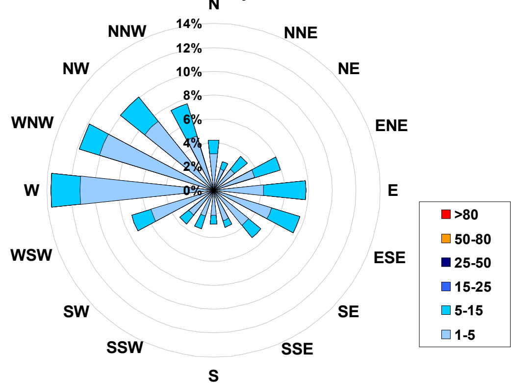
1-hr Average Concentration Rose for Particulate Matter (less than 2.5 microns) (in micrograms per cubic meter) Located at the Beaverlodge Site for May 2007
