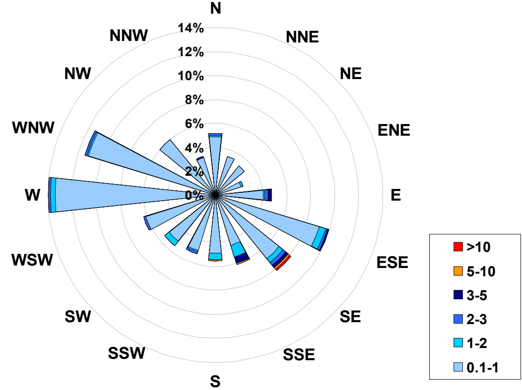
1-hr Average Concentration Rose for Total Reduced Sulphur (in ppb) Located at the Portable-Falher Site for May 2007
