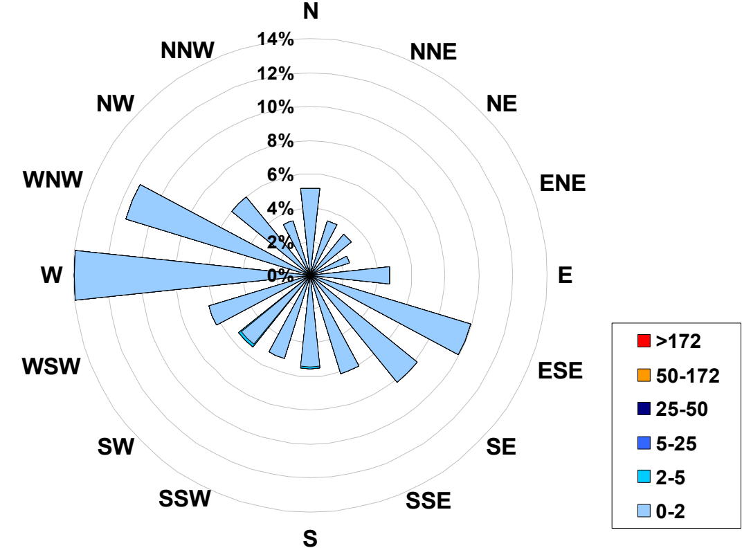
1-hr Average Concentration Rose for Sulphur Dioxide (in ppb) Located at the Portable-Falher Site for May 2007
