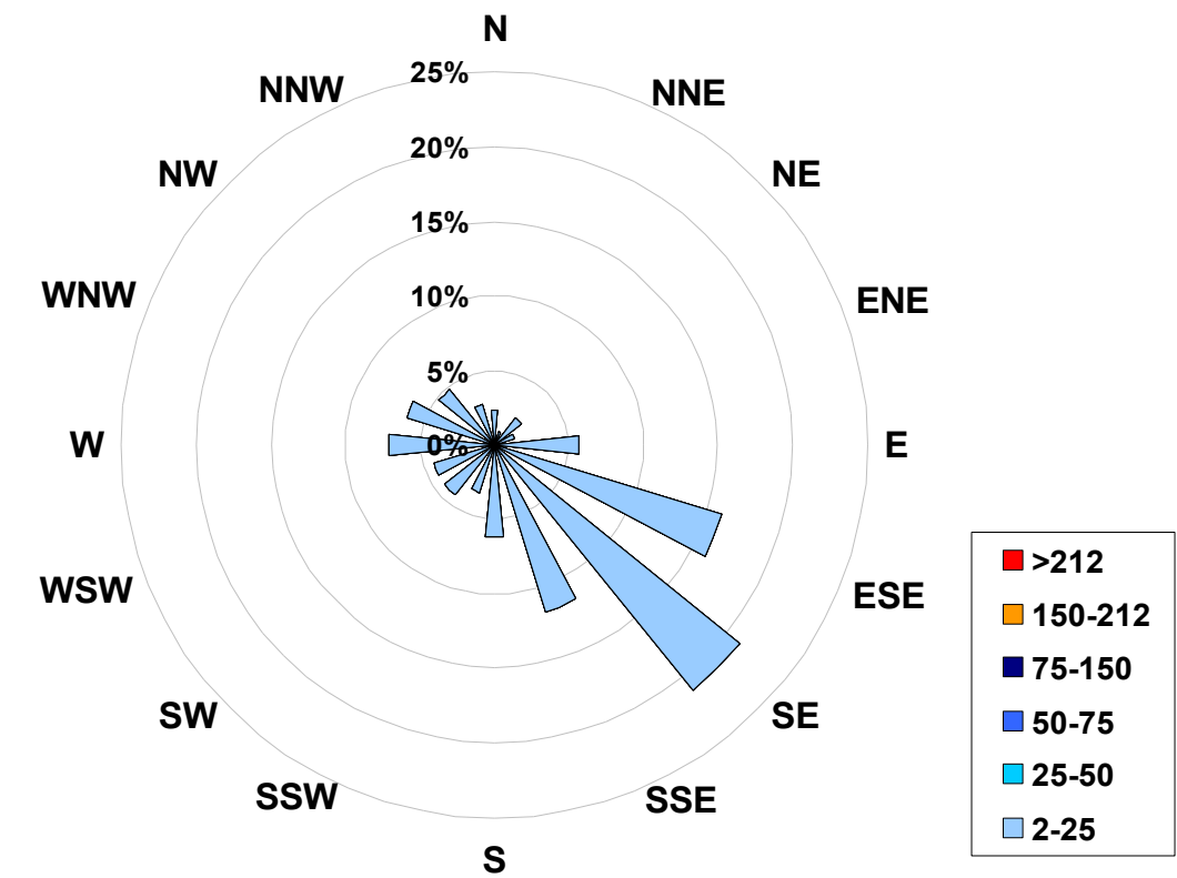
1-hr Average Concentration Rose for Nitrogen Dioxide (in ppb) Located at the Portable-Falher Site for May 2007
