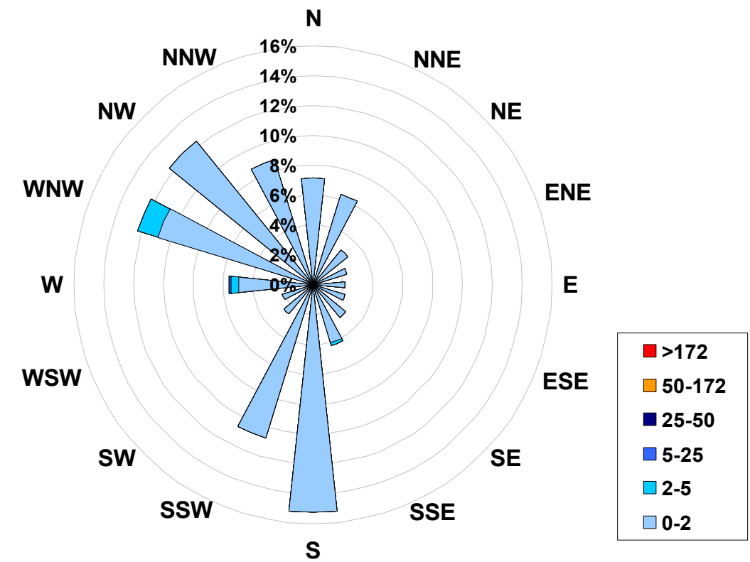
1-hr Average Concentration Rose for Sulphur Dioxide (in ppb) Located at the Valleyview Site for May 2007
