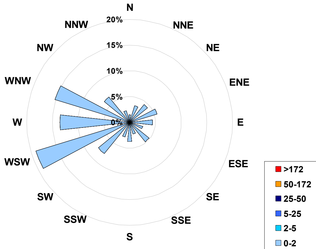
1-hr Average Concentration Rose for Sulphur Dioxide (in ppb) Located at the Henry Pirker Site for May 2007
