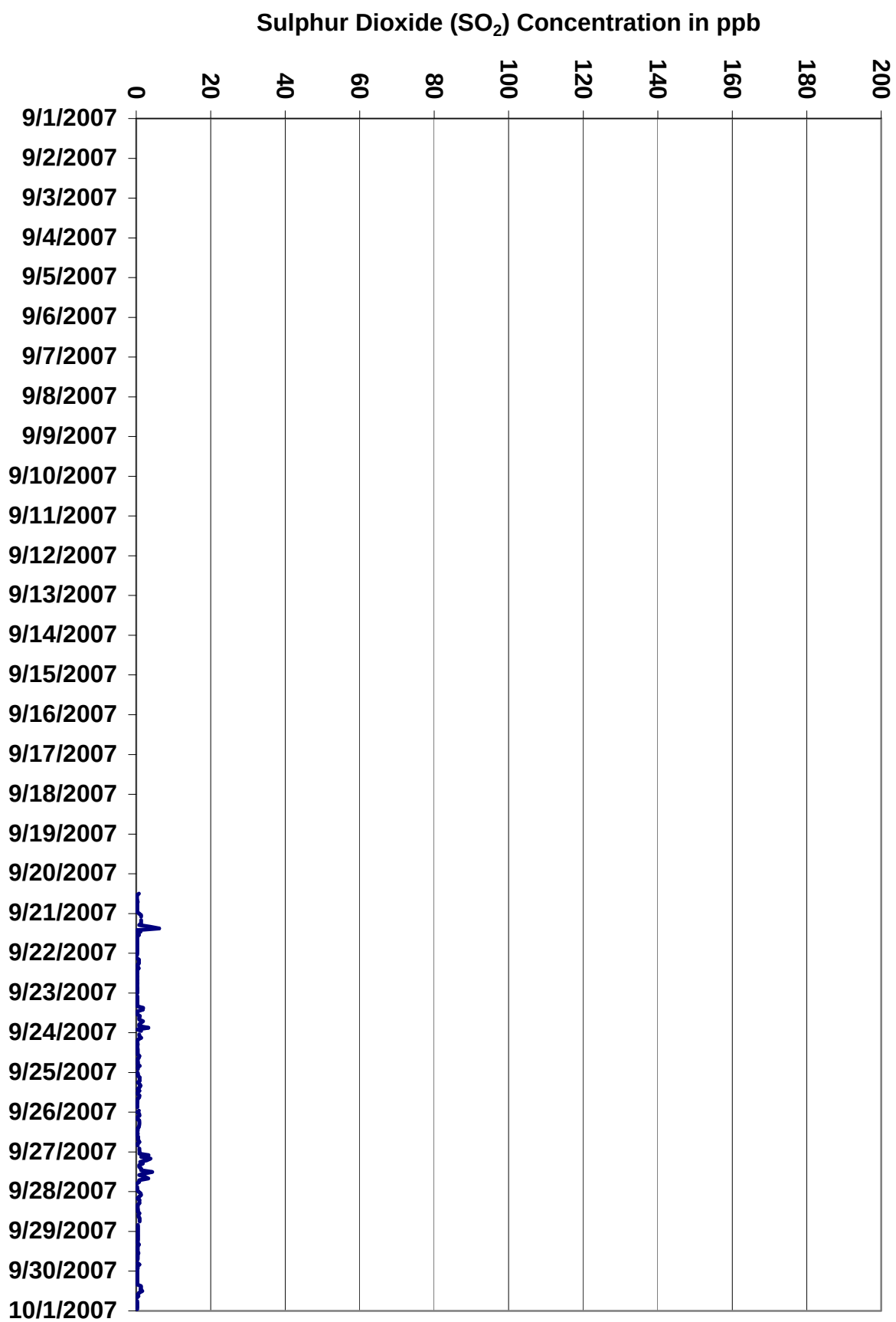
Figure 47. PASZA - Portable-Spirit River Sulphur Dioxide Instantaneous (30 Second) Maximum Value Monthly Trend
