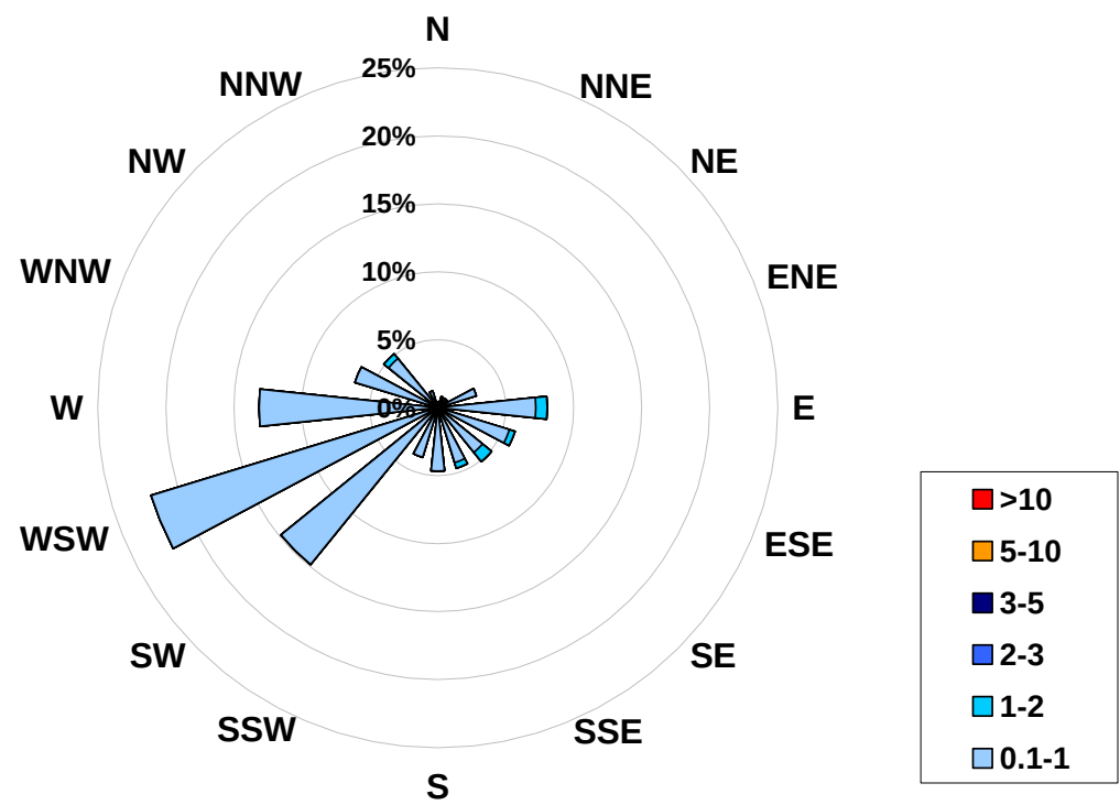
1-hr Average Concentration Rose for Total Reduced Sulphur (in ppb) Located at the Portable-Spirit River Site for September 2007
