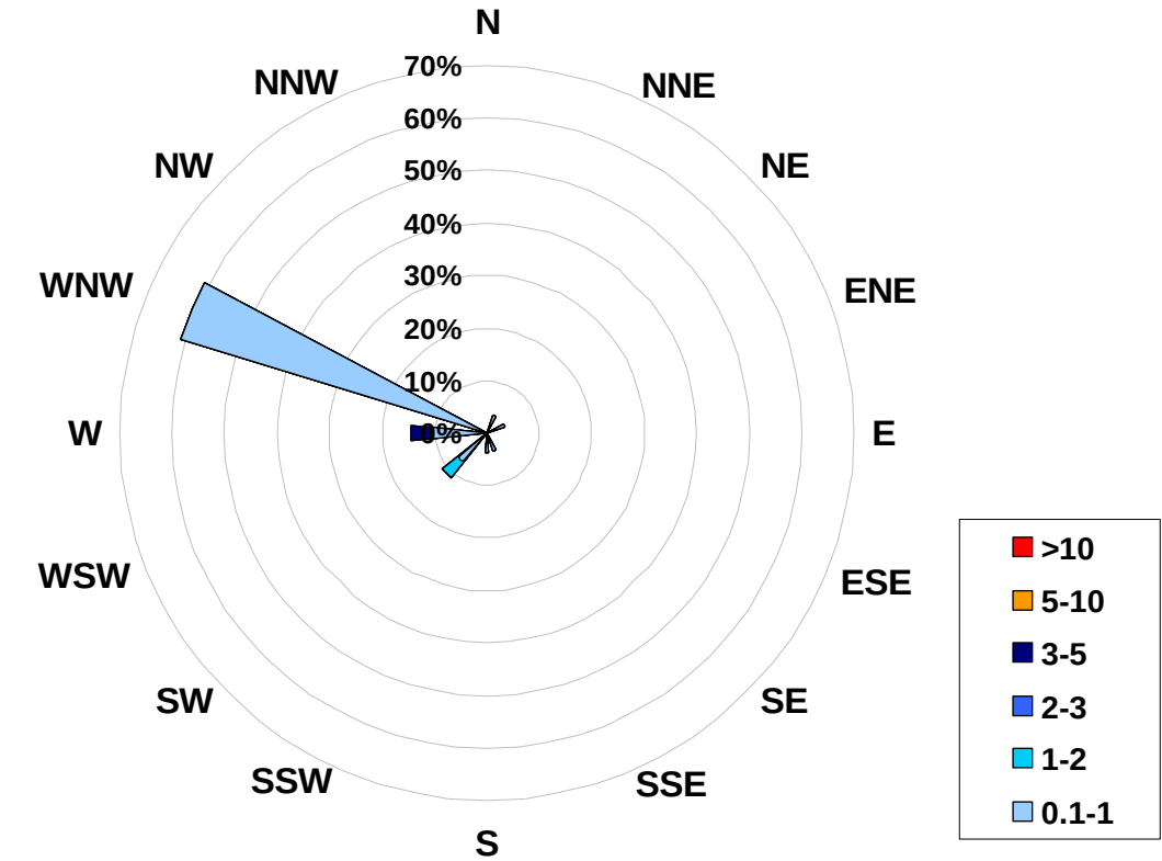
1-hr Average Concentration Rose for Hydrogen Sulphide (in ppb) Located at the Valleyview Site for September 2007
