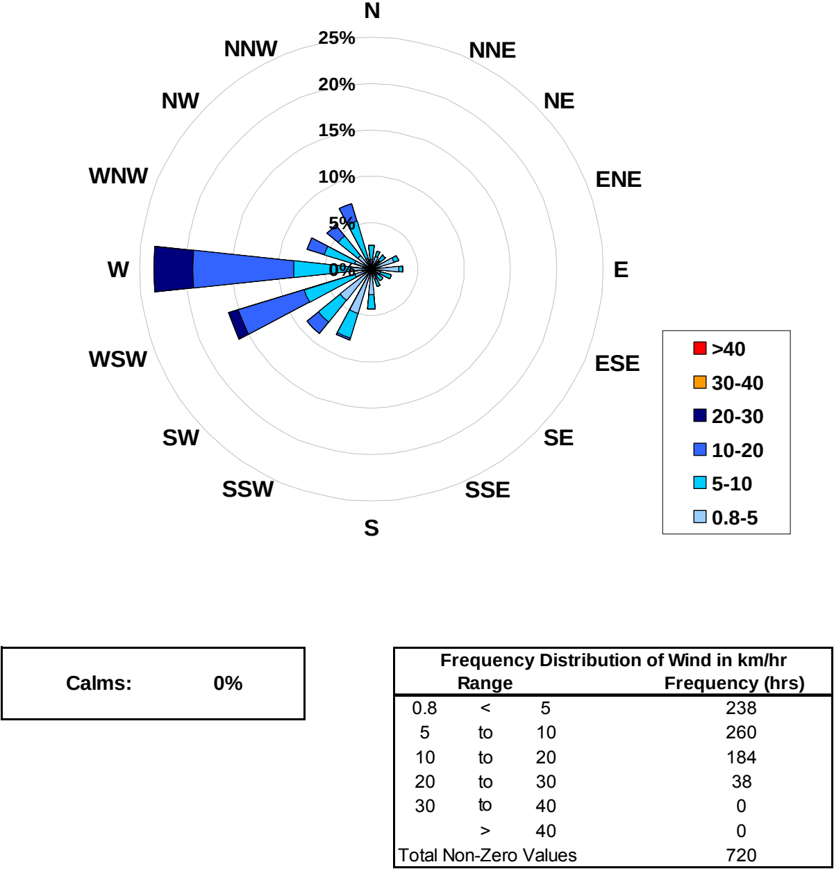
1-hr Average Wind Rose (in km/hr) Located at the Evergreen Park Site for September 2007
