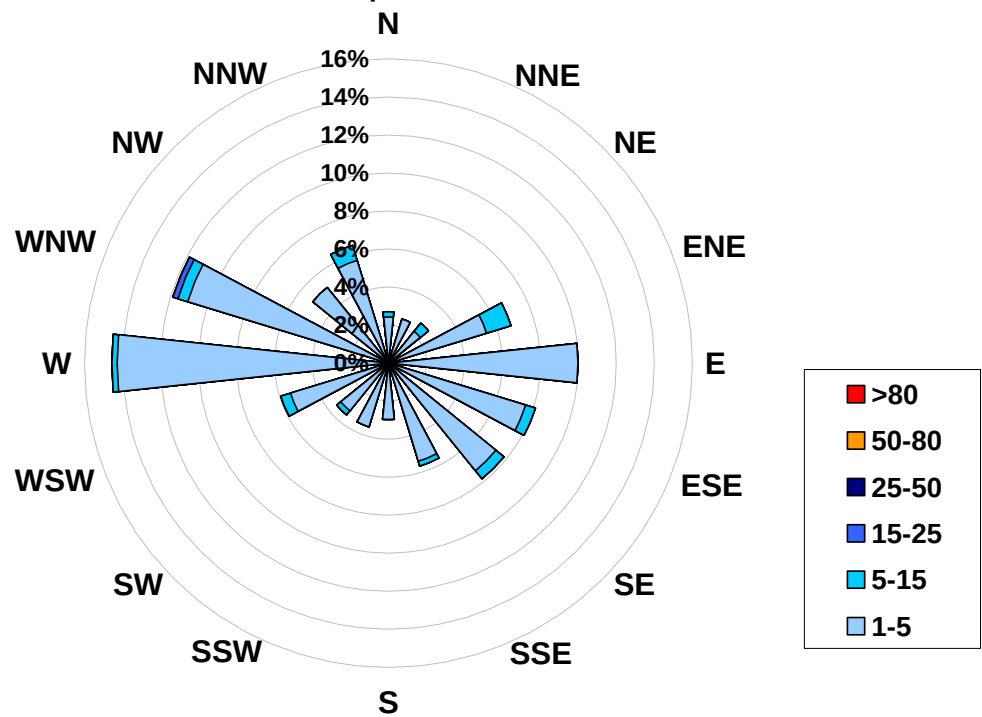
1-hr Average Concentration Rose for Particulate Matter (less than 2.5 microns) (in micrograms per cubic meter) Located at the Beaverlodge Site for September 2007
