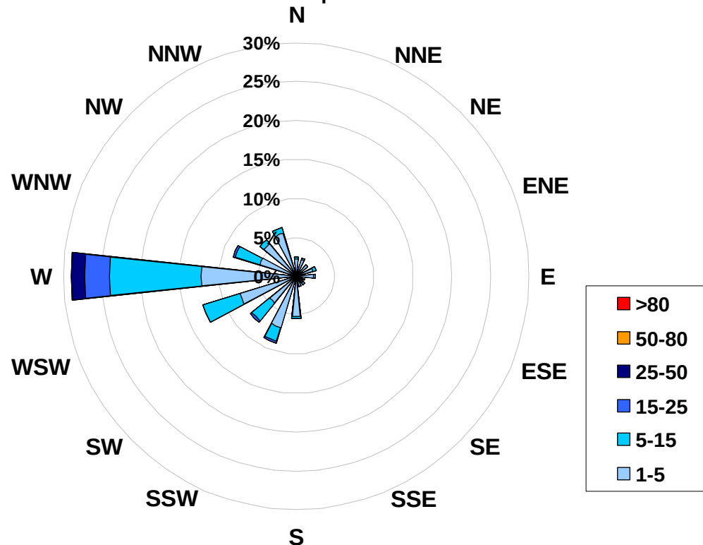
1-hr Average Concentration Rose for Particulate Matter (less than 2.5 microns) (in micrograms per cubic meter) Located at the Evergreen Park Site for September 2007
