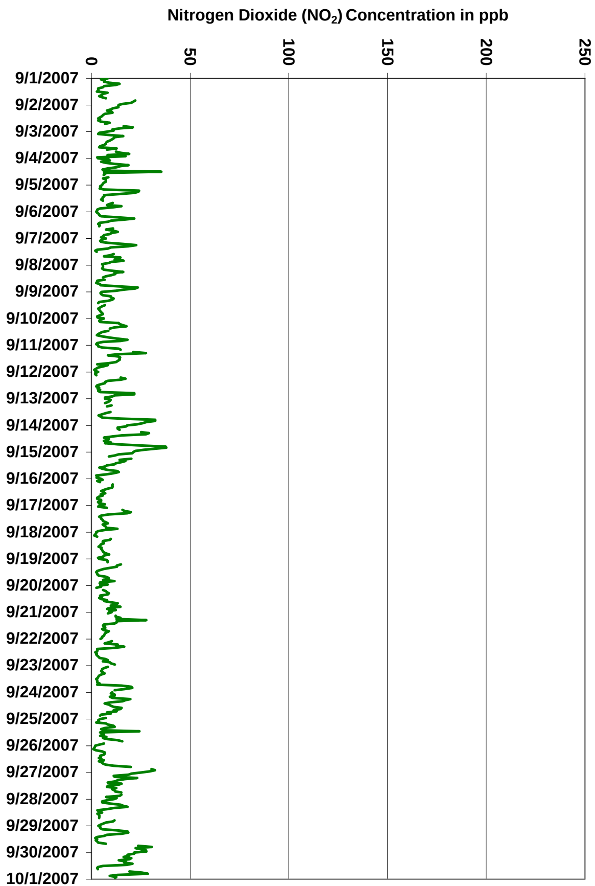
Figure 4. PASZA - Henry Pirkner Nitrogen Dioxide Instantaneous (30 Second) Maximum Value Monthly Trend
