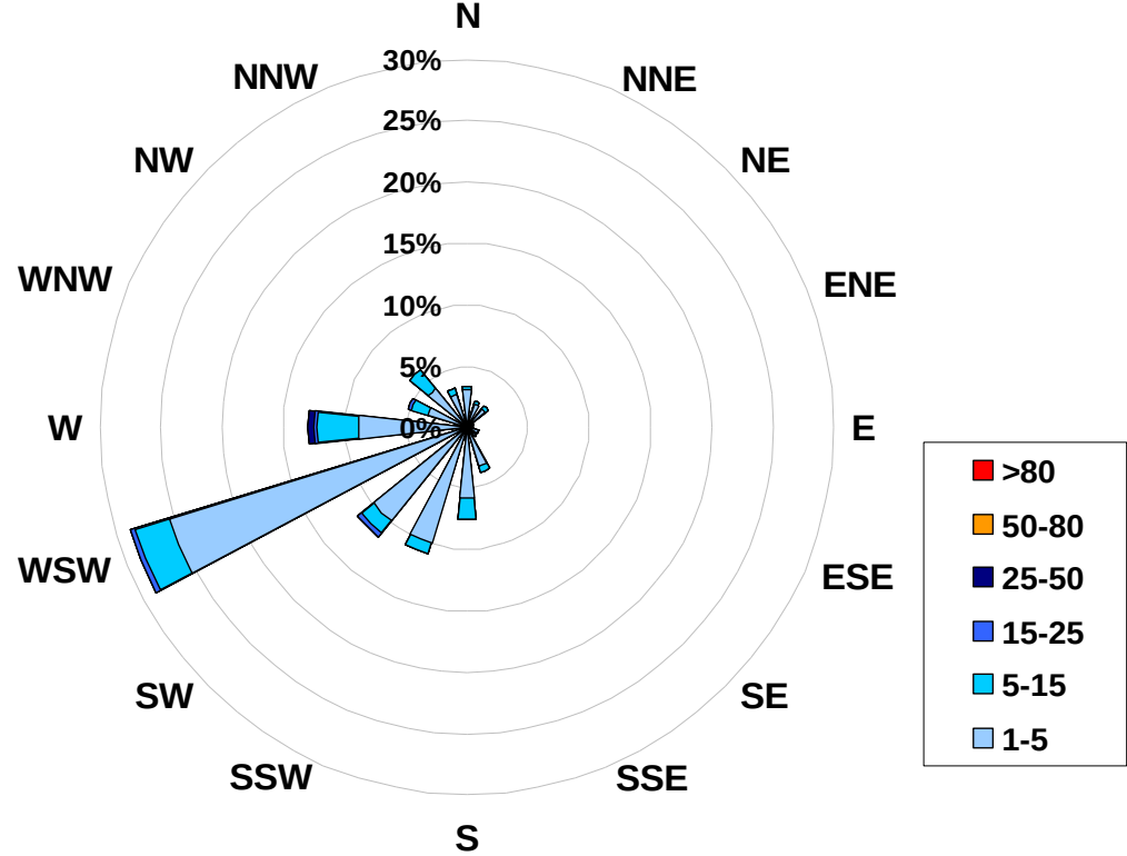
1-hr Average Concentration Rose for Particulate Matter (less than 2.5 microns) (in micrograms per cubic meter) Located at the Smoky Heights Site for September 2007
