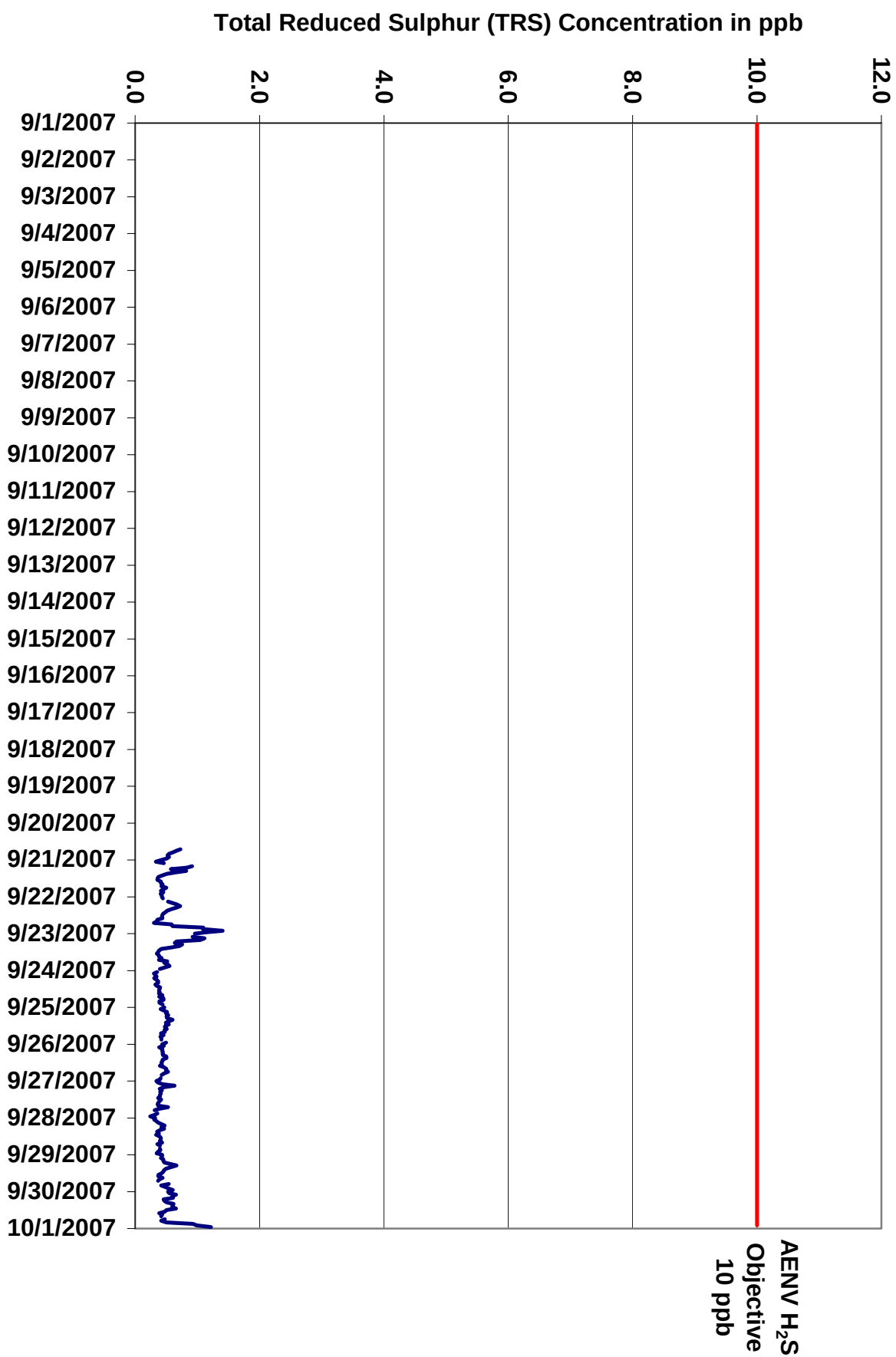
Figure 54. PASZA - Portable-Spirit River Total Reduced Sulphur 1-hr Average Monthly Trend
