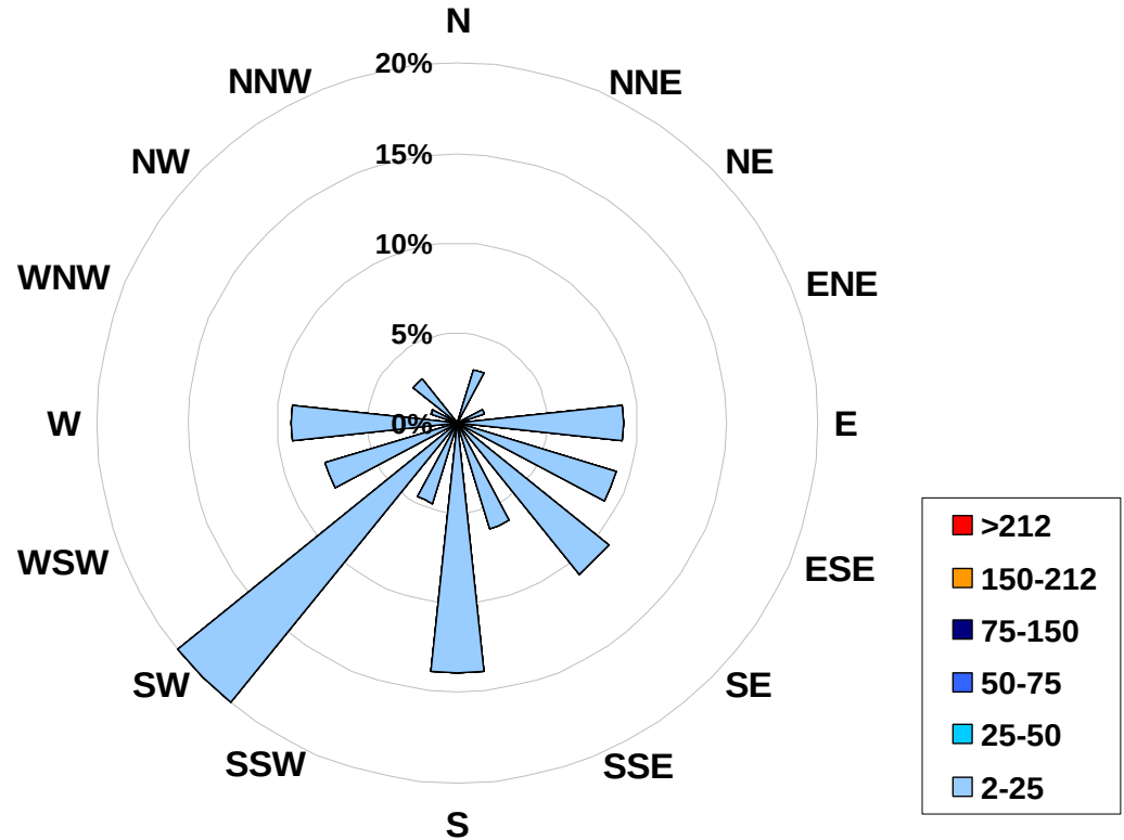
1-hr Average Concentration Rose for Nitrogen Dioxide (in ppb) Located at the Portable-Spirit River Site for September 2007
