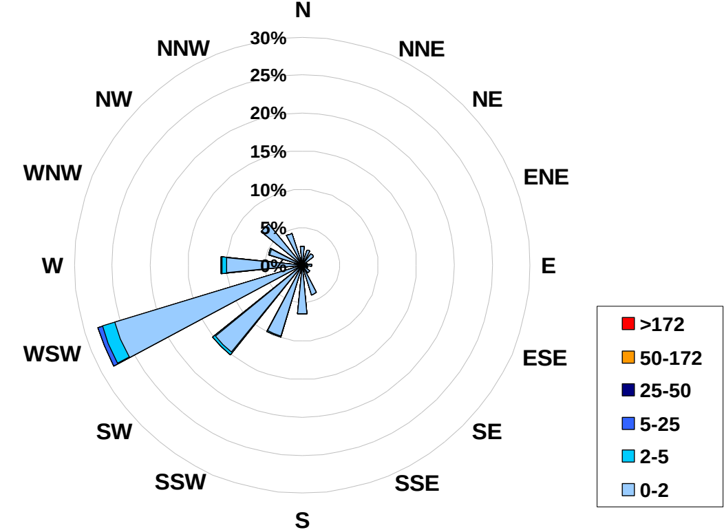
1-hr Average Concentration Rose for Sulphur Dioxide (in ppb) Located at the Smoky Heights Site for September 2007
