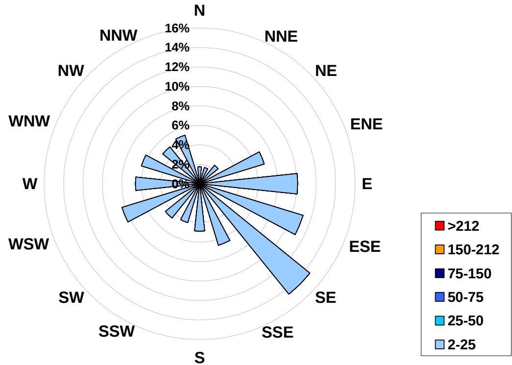
1-hr Average Concentration Rose for Nitrogen Dioxide (in ppb) Located at the Beaverlodge Site for September 2007
