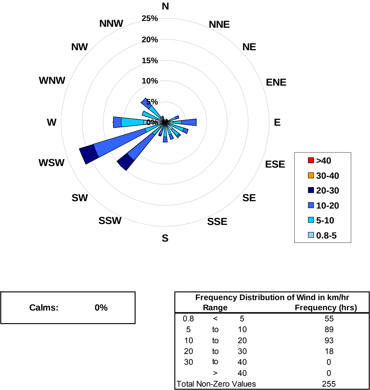
1-hr Average Wind Rose (in km/hr) Located at the Portable-Spirit River Site for September 2007
