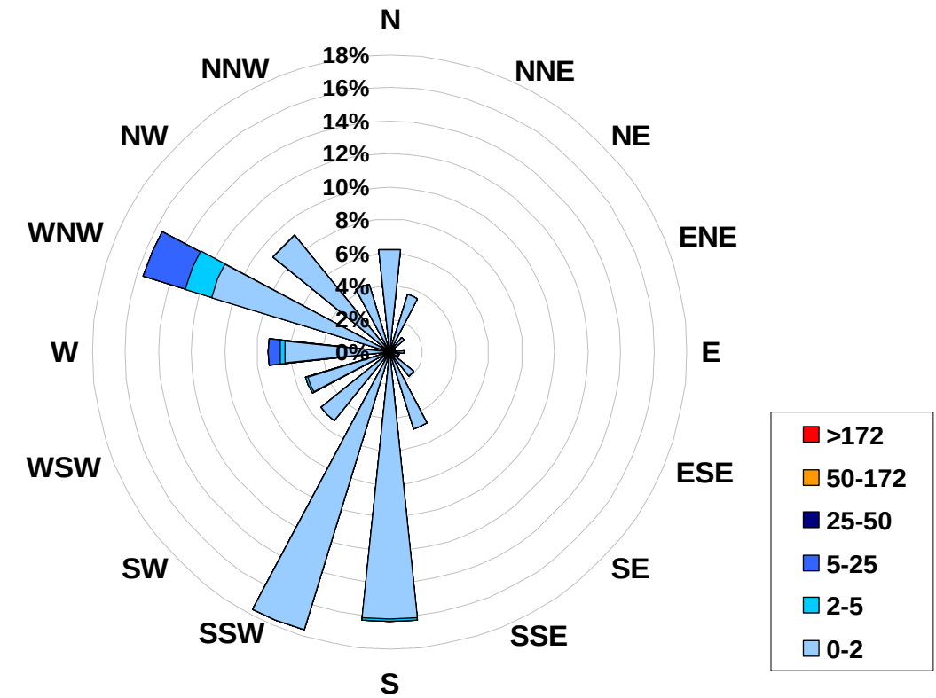
1-hr Average Concentration Rose for Sulphur Dioxide (in ppb) Located at the Valleyview Site for September 2007
