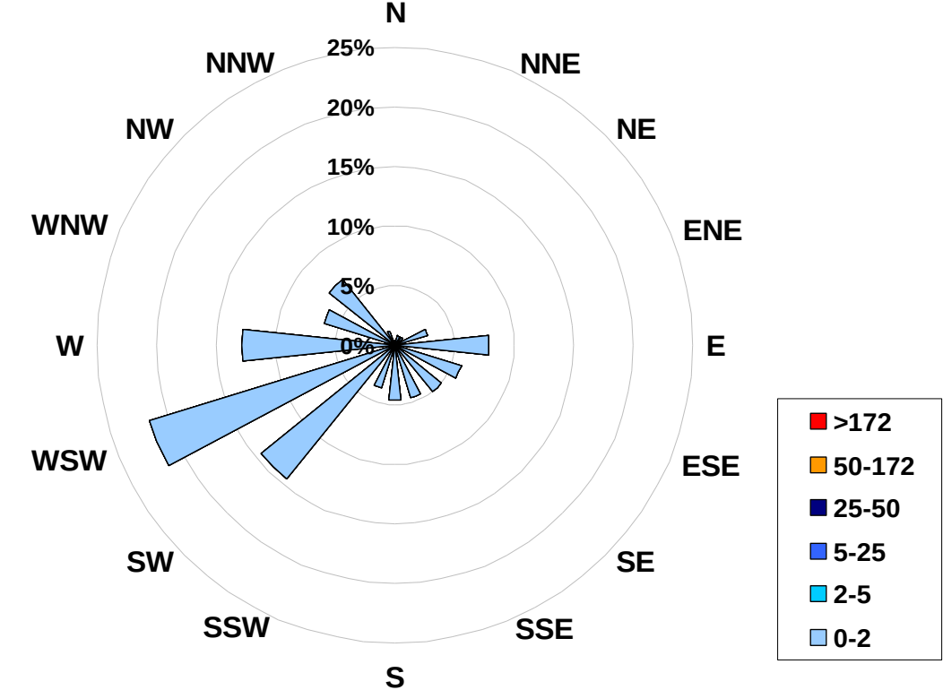
1-hr Average Concentration Rose for Sulphur Dioxide (in ppb) Located at the Portable-Spirit RiverSite for September 2007
