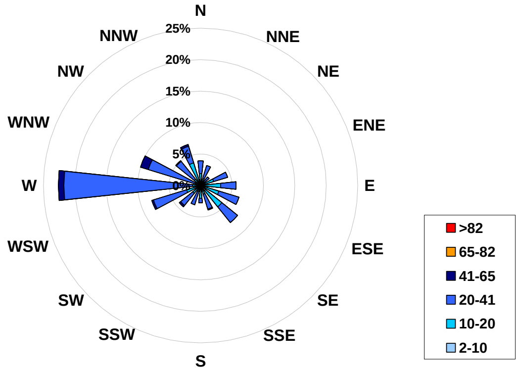
1-hr Average Concentration Rose for Ozone (in ppb) Located at the Beaverlodge Site for September 2007
