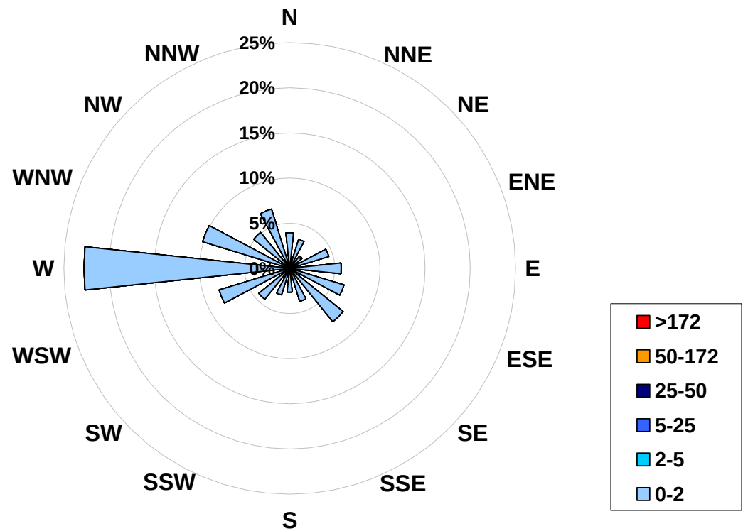
1-hr Average Concentration Rose for Sulphur Dioxide (in ppb) Located at the Beaverlodge Site for September 2007
