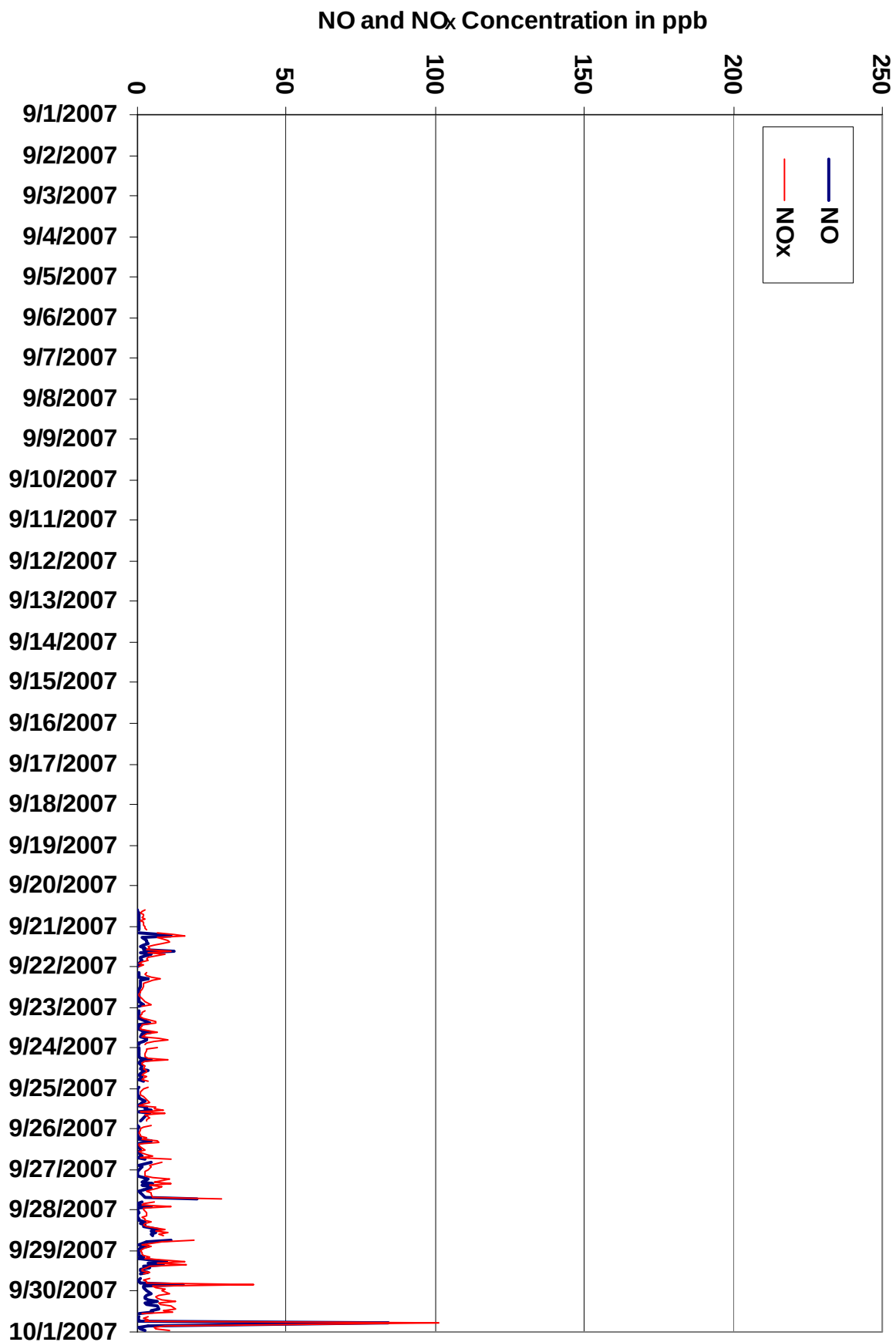
Figure 51. PASZA - Portable-Spirit River Oxides of Nitrogen Instantaneous (30 Second) Maximum Value Monthly Trend
