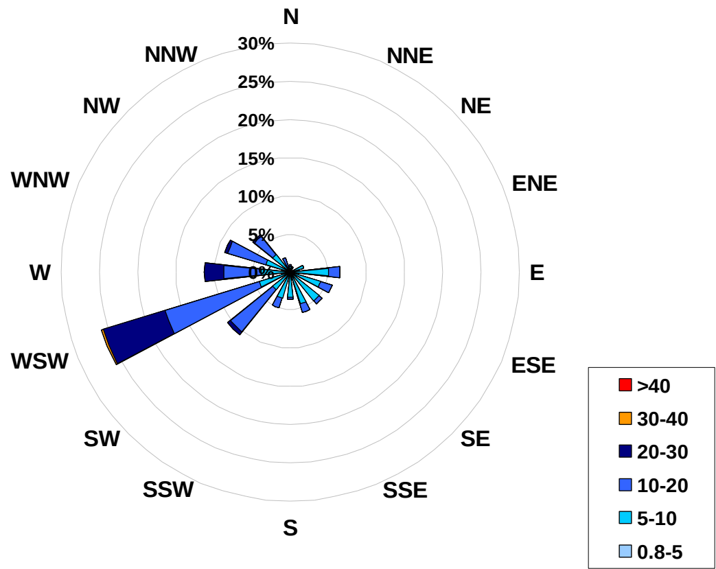
1-hr Average Wind Rose (in km/hr) Located at the Henry Pirker Site for September 2007
