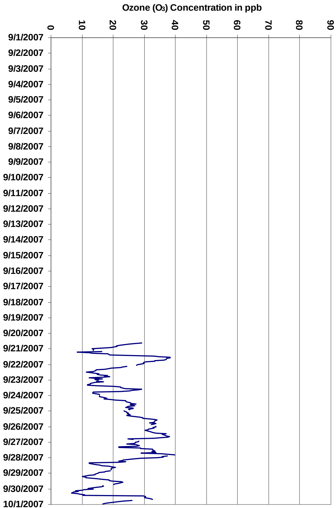
Figure 53. PASZA - Portable-Spirit River Ozone Instantaneous (30 Second) Maximum Value Monthly Trend
